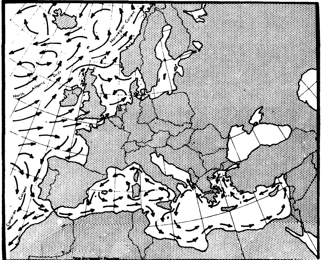
FIGURE 4-1 OCEAN CURRENTS AFFECTING EUROPE 4-1
