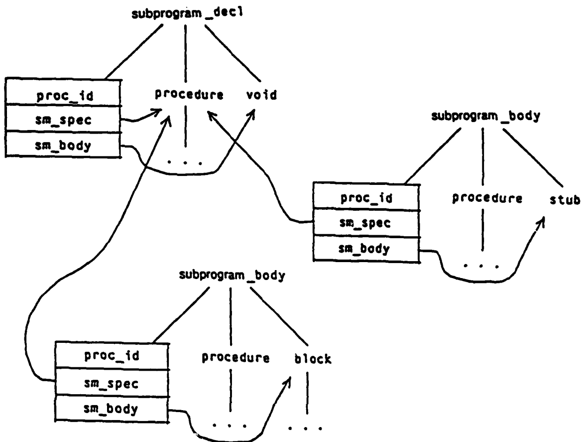
Figure 3-14: Example of a Subprogram Body as a subunit (I)
