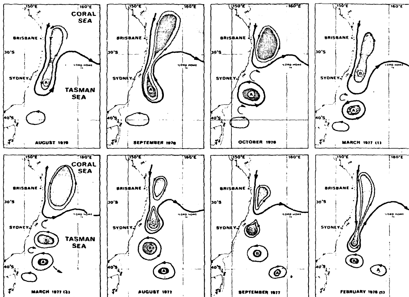
Fig. 3. A summary of the observations of eddies A, B and C over the period August 1976 through February 1978. The heavy line marks the division between the Coral Sea water ( T_{250} > 15 C) and Tasman Sea water ( T_{250} < 15 C). The most heavily shaded areas represent the regions of highest dynamic height ( T_{250} > 17 C). From Nilsson and Cresswell, 1980.
