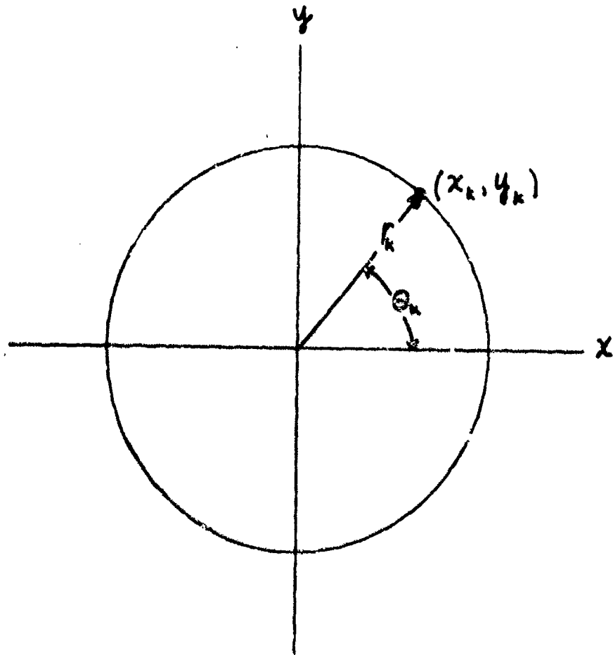
Figure 4. A coherence sample as a point on the unit circle in the complex plane. A coherence estimate is the average of such samples over a specified number of frequencies and/or a specified number of time epochs.
