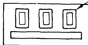
b) Two-Input "Wire-or" Phase Splitter (extra base diffusion not connected)
