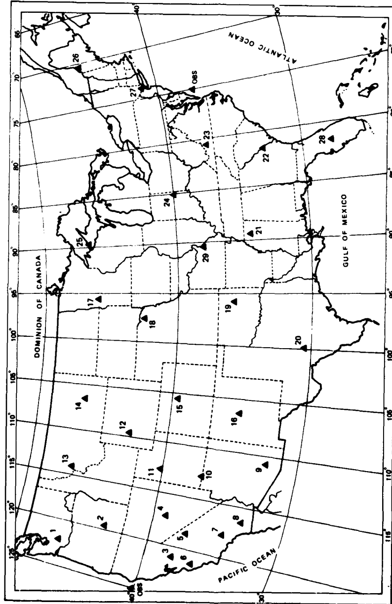
EXHIBIT C-1 Proposed locations of 29 continental and 2 ocean-bottom observatories for the National Digital Seismograph Network (NDSN).
