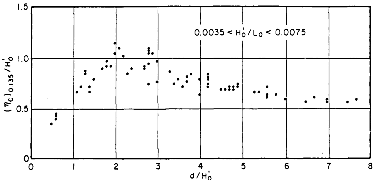
Figure 23. Wave crest elevation exceeded by 13.5 percent of the wave crests.
