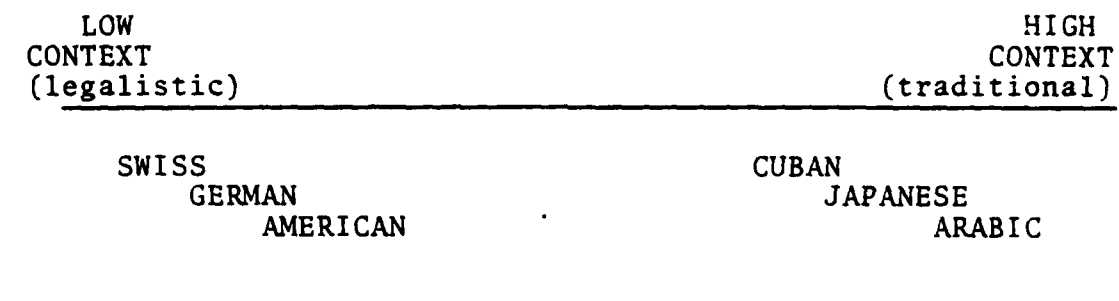
Figure 2.2. Context Bandwidth.
