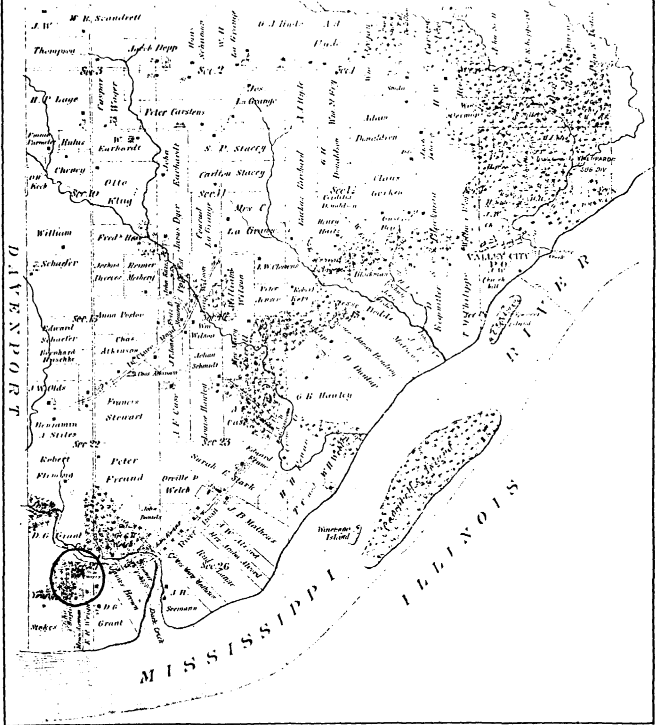
Figure 2. 1882 Schmidt and Huebinger Atlas Plat Map Showing Location of Quarry Near Project Area B.
