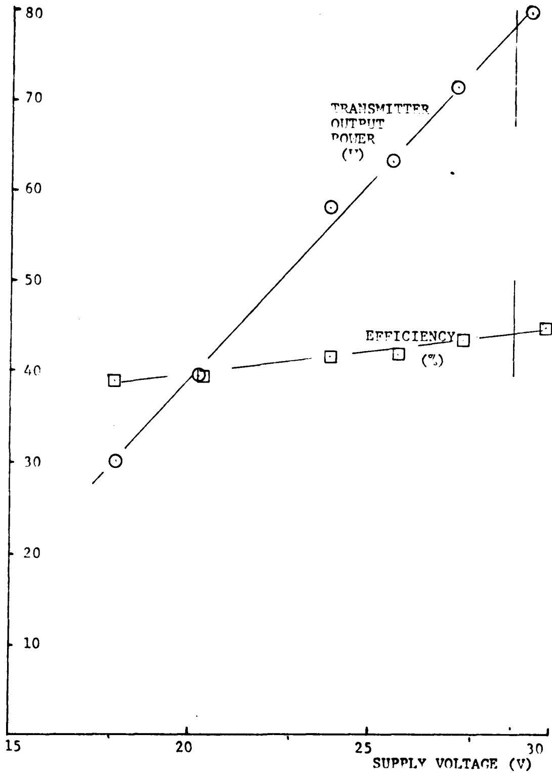
FIGURE 17. TRANSMITTER POWER OUTPUT
