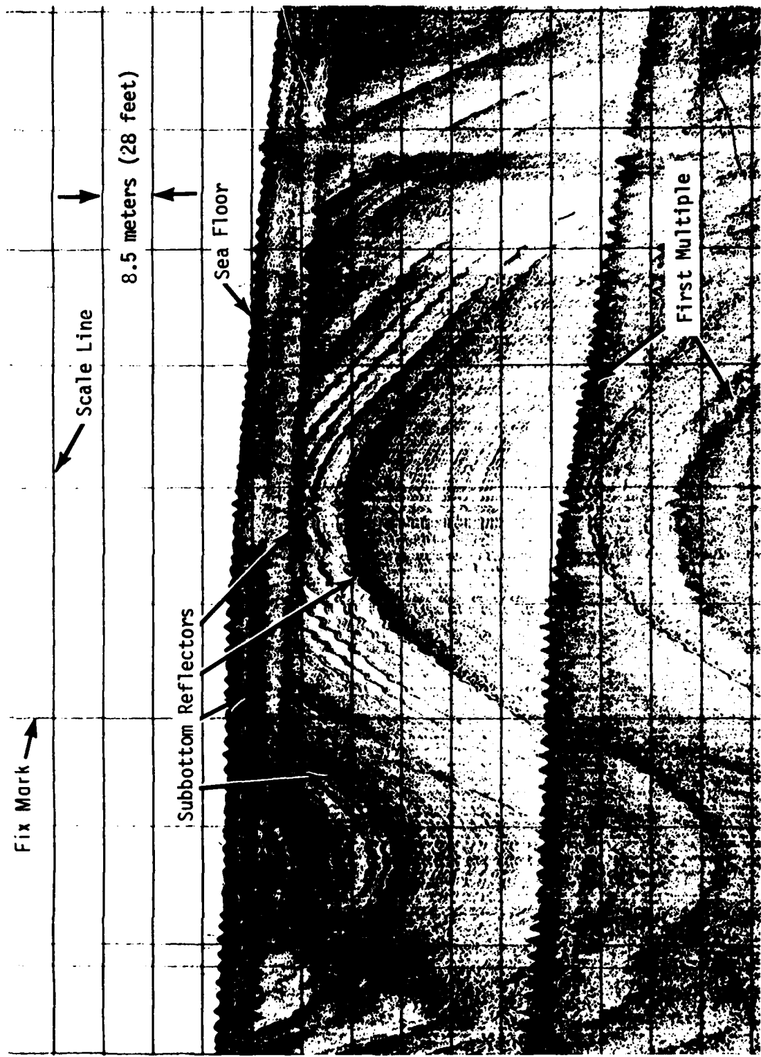
Figure 4. Example of Uniboom profile showing Holocene age sandy sediments overlying folded consolidated bedrock.
