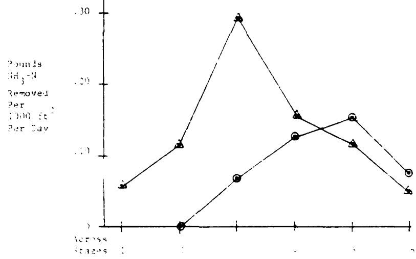
Figure 6. Effects of Dissolved Oxygen Concentration on the NH 3 -N Removal Rate (Data from Table 1)
