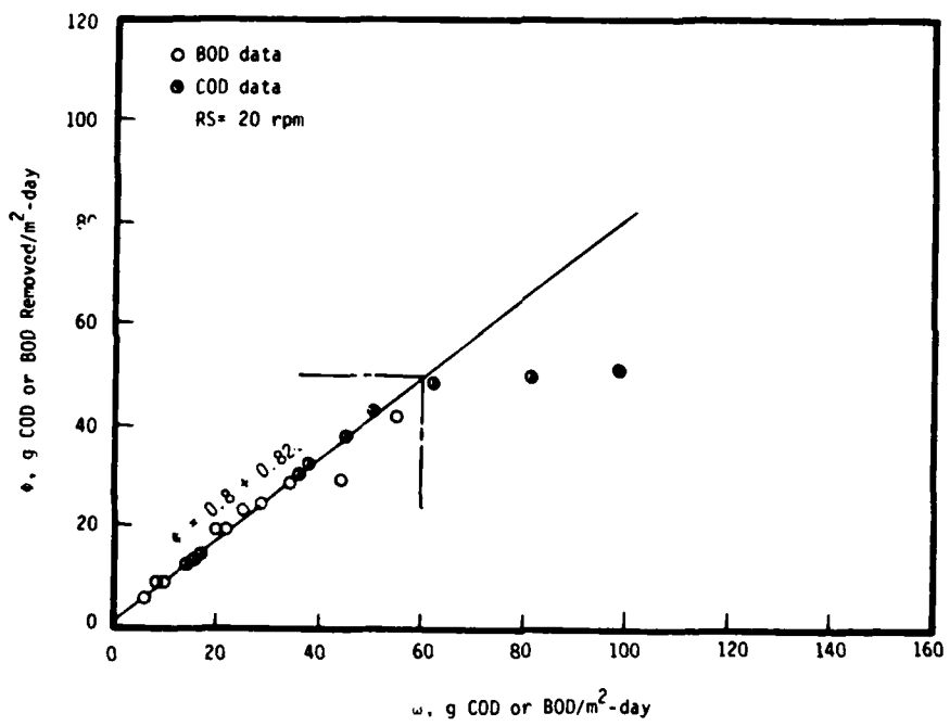
Figure 4. Relationship Between Organic Loading and Substrate Removal Efficiency In Air RBC System
