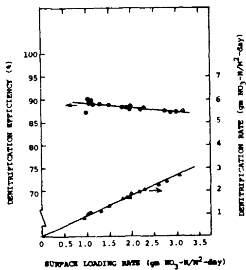
Figure 6. Level of Denitrification Vs. Surface Loading Rate of Nitrate-Nitrogen (NO 3 -N)
