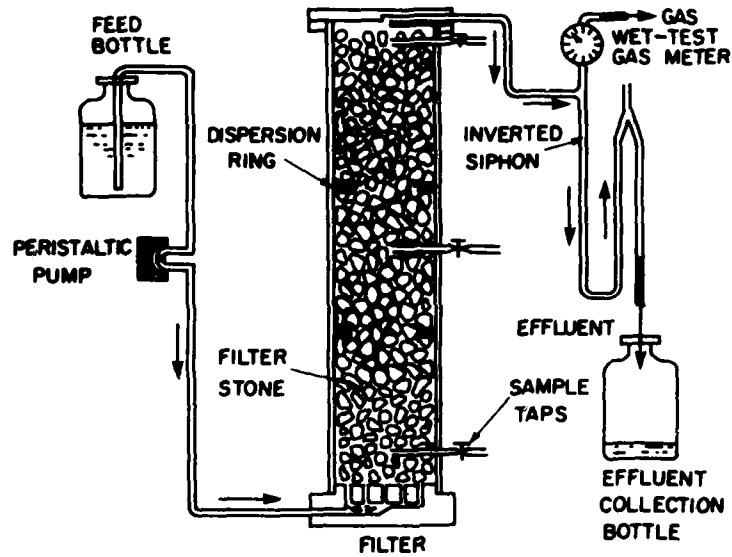
Figure 3. Schematic Illustration of Anaerobic Filter System.
