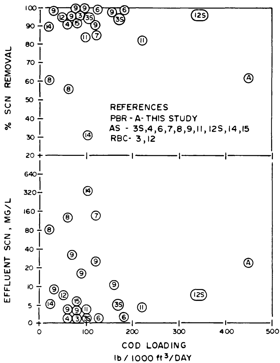
FIGURE 8 SCN REMOVAL VERSUS ORGANIC LOAD FOR VARIOUS BIOLOGICAL REACTORS
