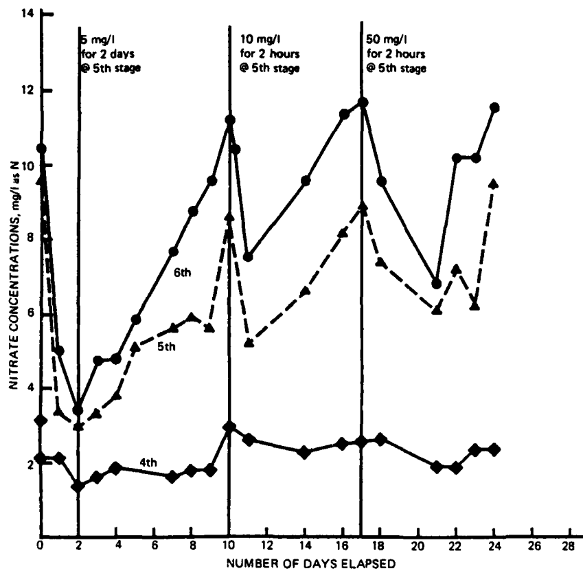
FIGURE 6. SHOCK RESPONSES ON NITRIFYING CULTURES
