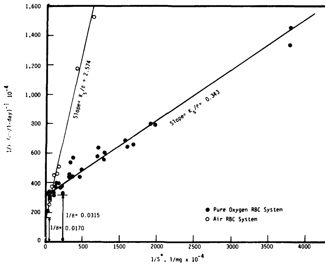
Figure 7. Determination of \mu and K_s On BOD Data Basis
