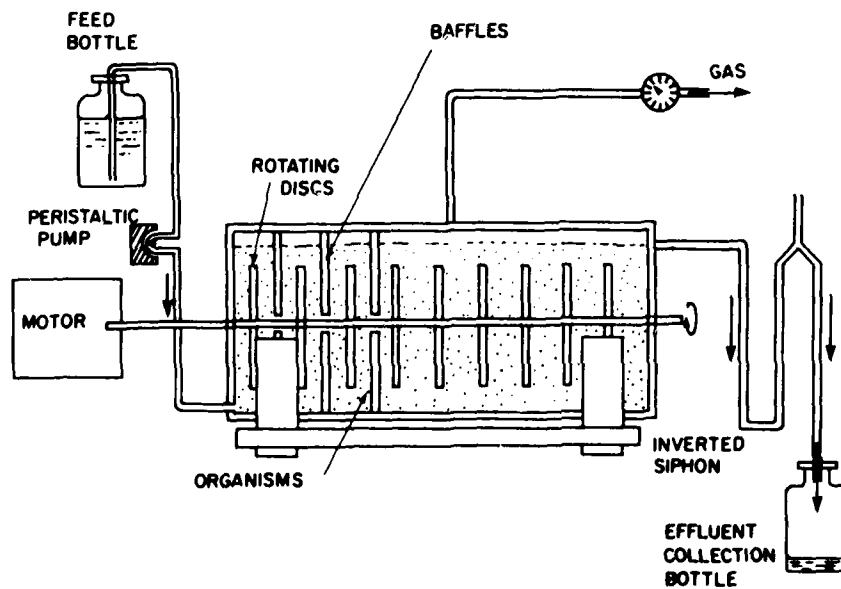
Figure 4. Schematic Illustration of Anaerobic Rotating Biological Contactor System.
