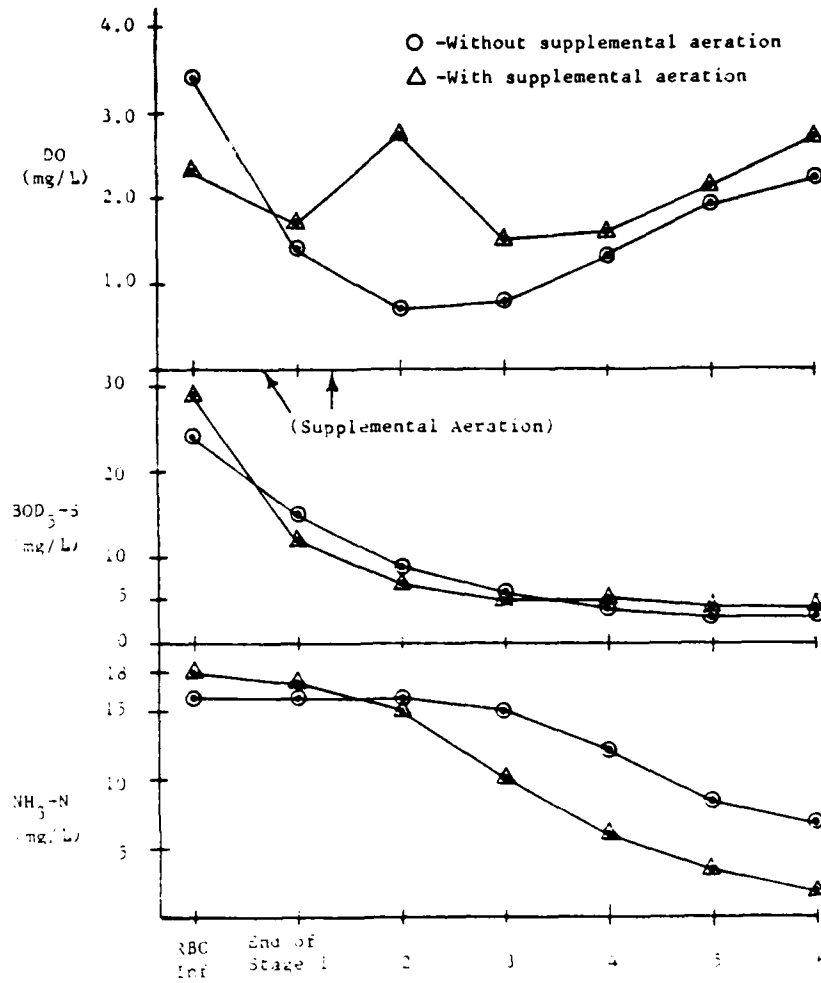
Figure 3. Comparison of DO, BOD 5-S , and NH 3-N Levels Through RBC Bank + with and without Supplemental Aeration (Data from Table 1).
