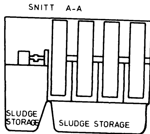
Figure 3. Plan and sectional side view of the RBC, S5 Rotordisk.
