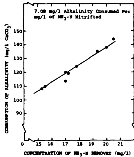
Figure 10. Consumption of Alkalinity as a Function of NH 3 -N Nitrified
