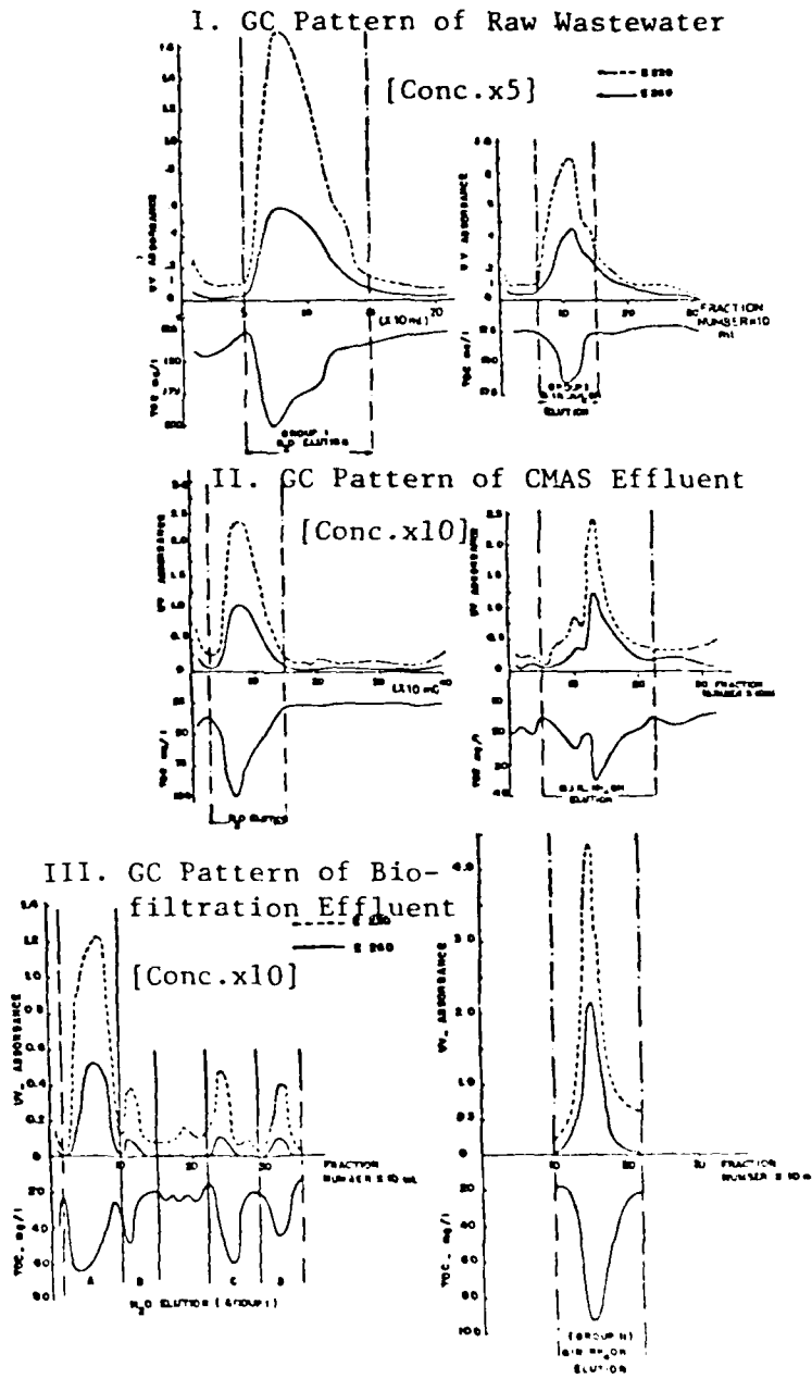
Figure 8. GC Patterns of Raw and Biologically Treated Tannery Effluents.
