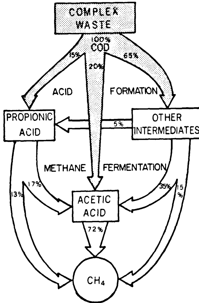
Figure 2. Metabolic Pathway In Methane Fermentation of Complex Organic Wastes [ taken from McCarty ( 1 ) ]
