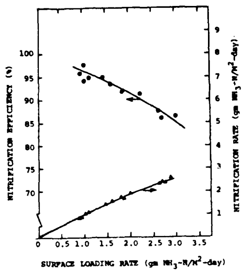
Figure 5. Level of Nitrification Vs. Surface Loading Rate of Ammonia-Nitrogen (NH 3 -N)
