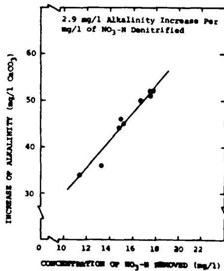
Figure 11. Increase of Alkalinity as a Function of NO 3 -N Denitrified
