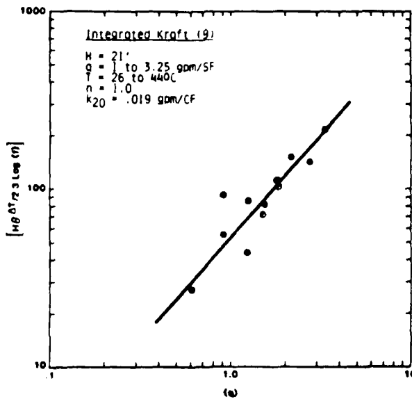
Figure 11 Treatment of Integrated Kraft Effluent on a Surfloc Tower (9)
