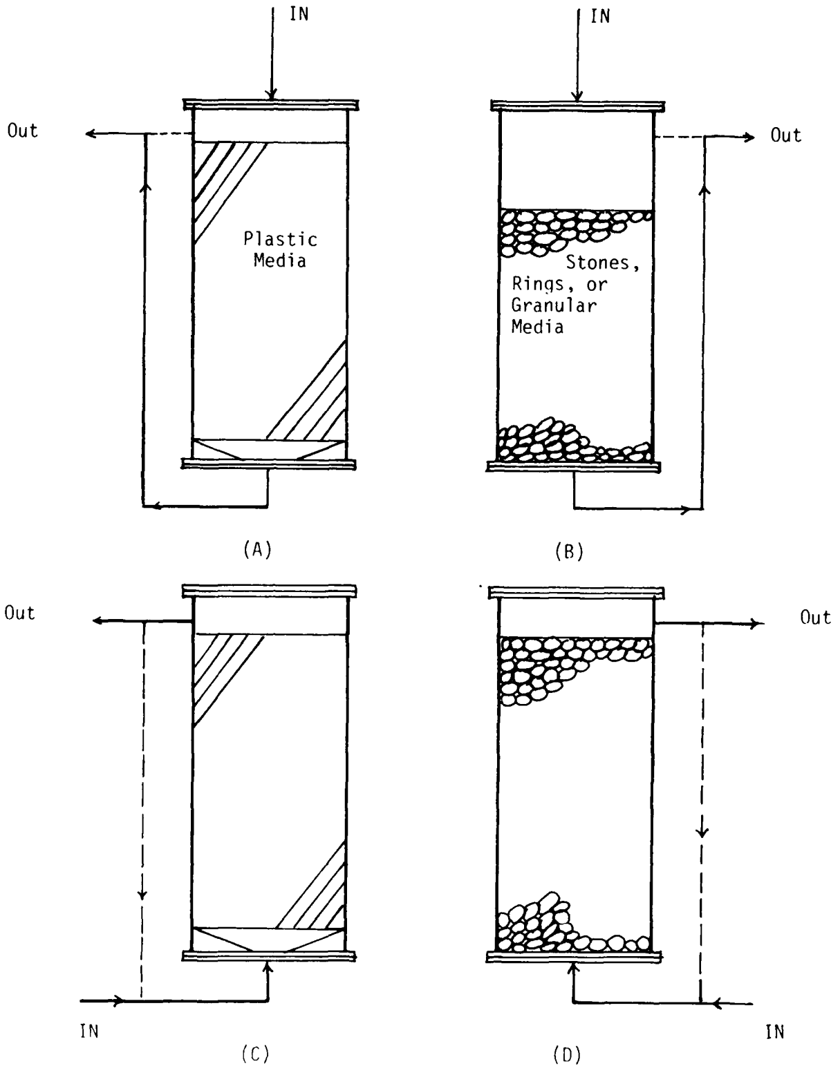
Figure 1. Schematic of Anaerobic Filters- (A) and (B) Downflow Reactors; (C) and (D) Upflow Reactors
