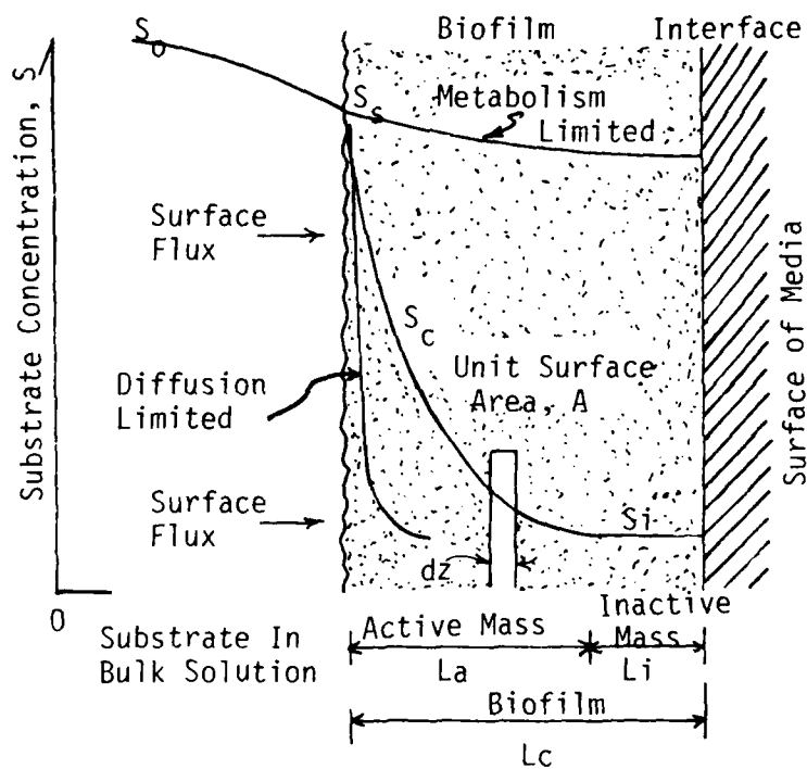
Figure 3. Substrate Concentration Profile Within A Biofilm [taken from Williamson & McCarty (37)]
