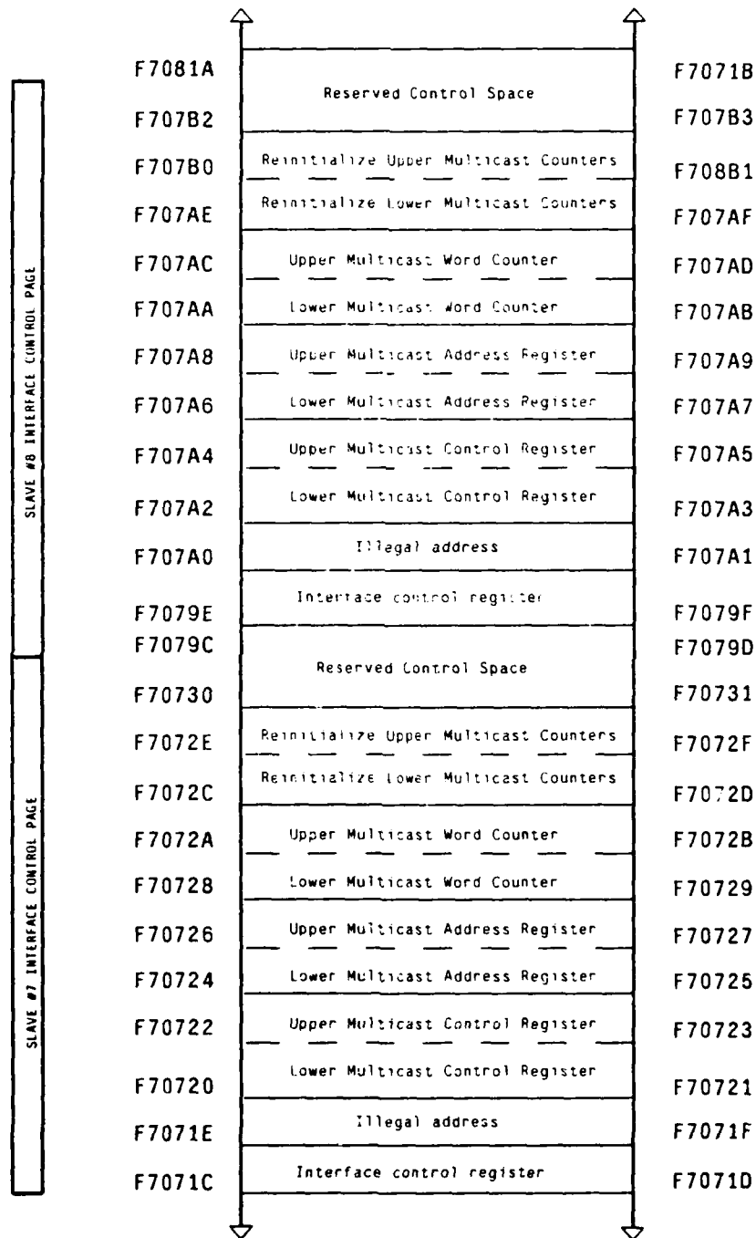
Figure 4-23: Slave #7 and Slave #8 interface control page
