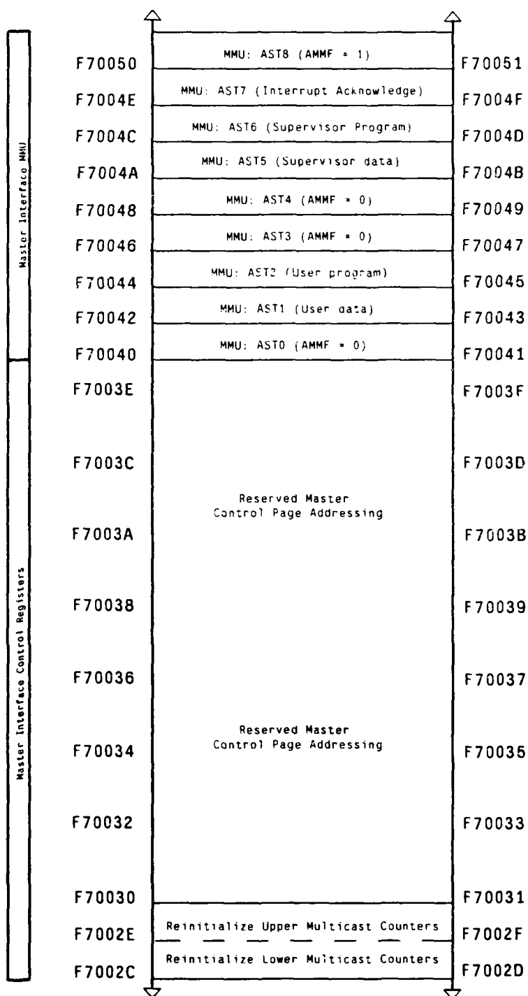
Figure 4-18: Master interface control page
