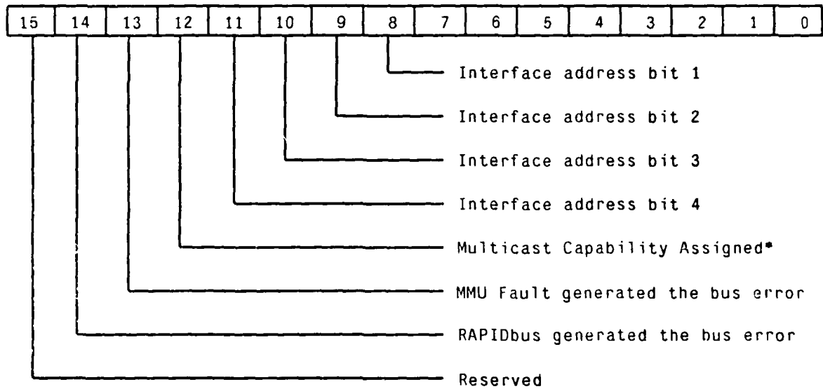
Figure 4-13: Interface control register high byte
