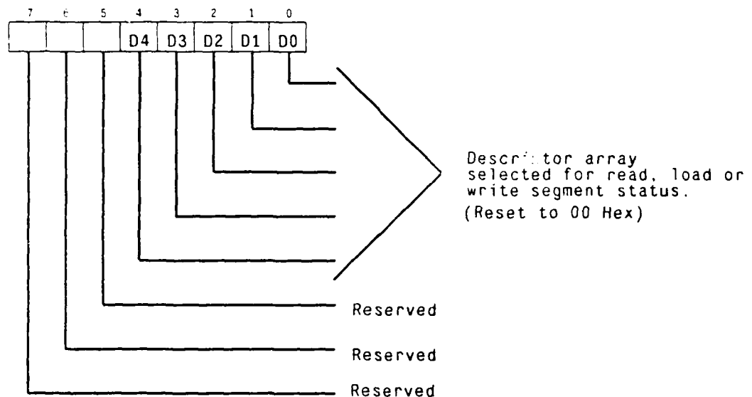
Figure 4-6: The descriptor pointer selects the descriptor array that is used in a load descriptor operation, read segment status, and the write segment status operation [16]
