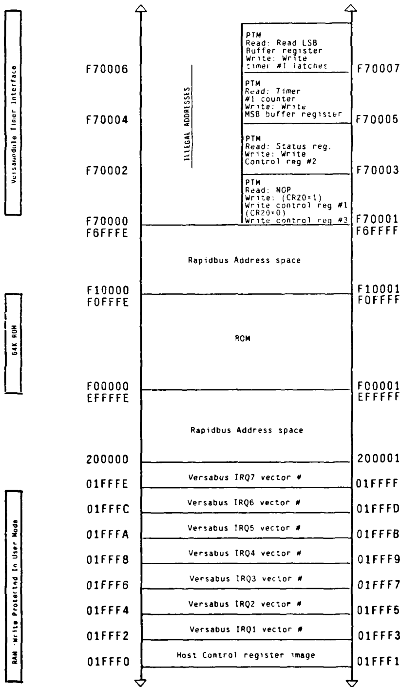
Figure 4-16: Upper RAM supervisor space, ROM, and Timers
