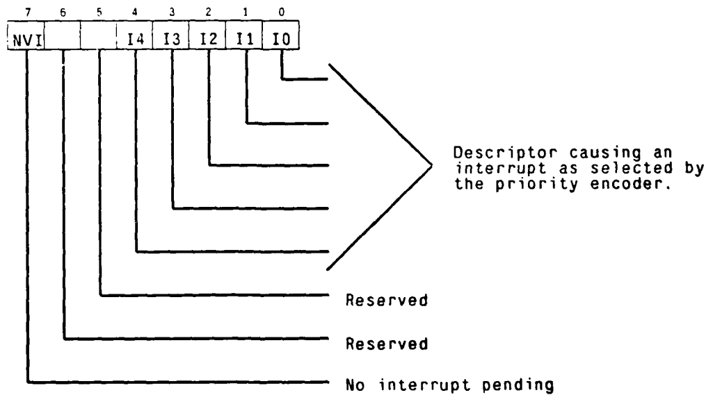
Figure 4-10: The interrupt descriptor pointer indicates which descriptor array was in use when an interrupt was generated [16].
