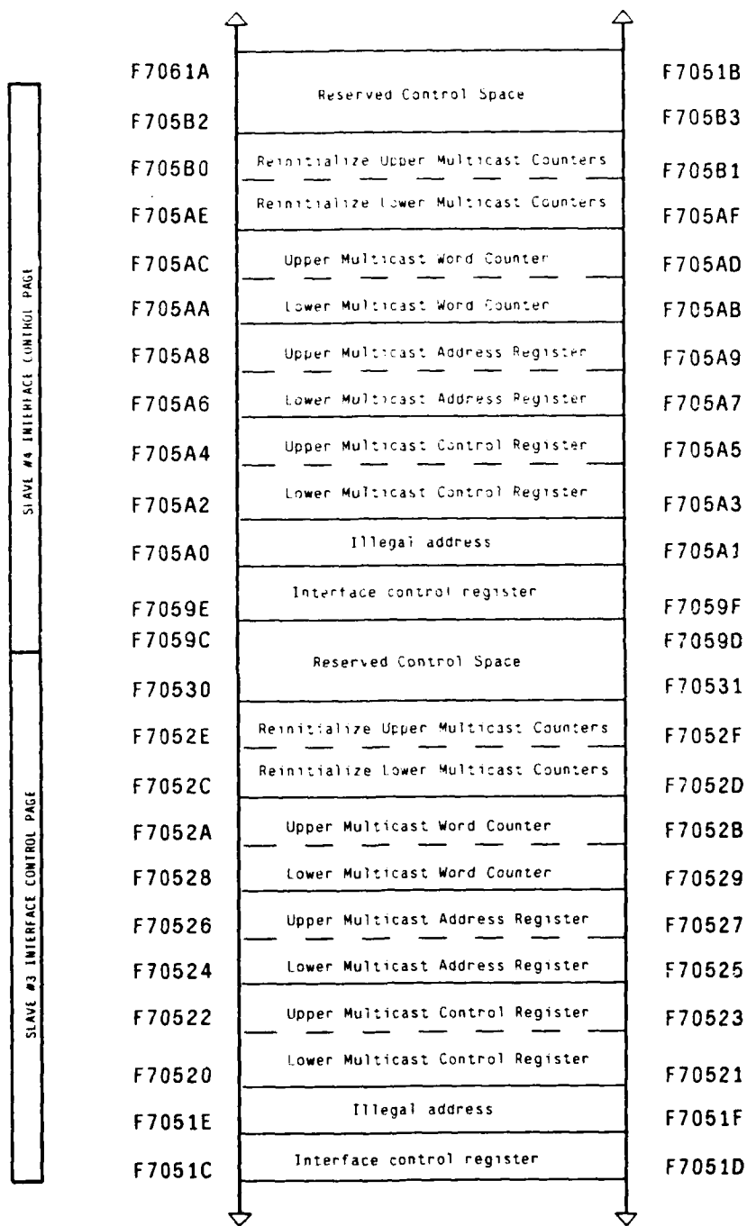
Figure 4-21: Slave #3 and Slave #4 interface control page
