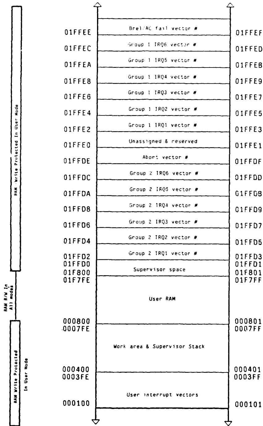
Figure 4-15: User RAM and upper supervisor space
