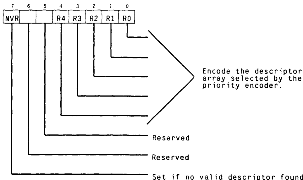
Figure 4-11: The Result Descriptor Pointer identifies the descriptor involved in a write violation, load descriptor failure, or direct translation success [16].
