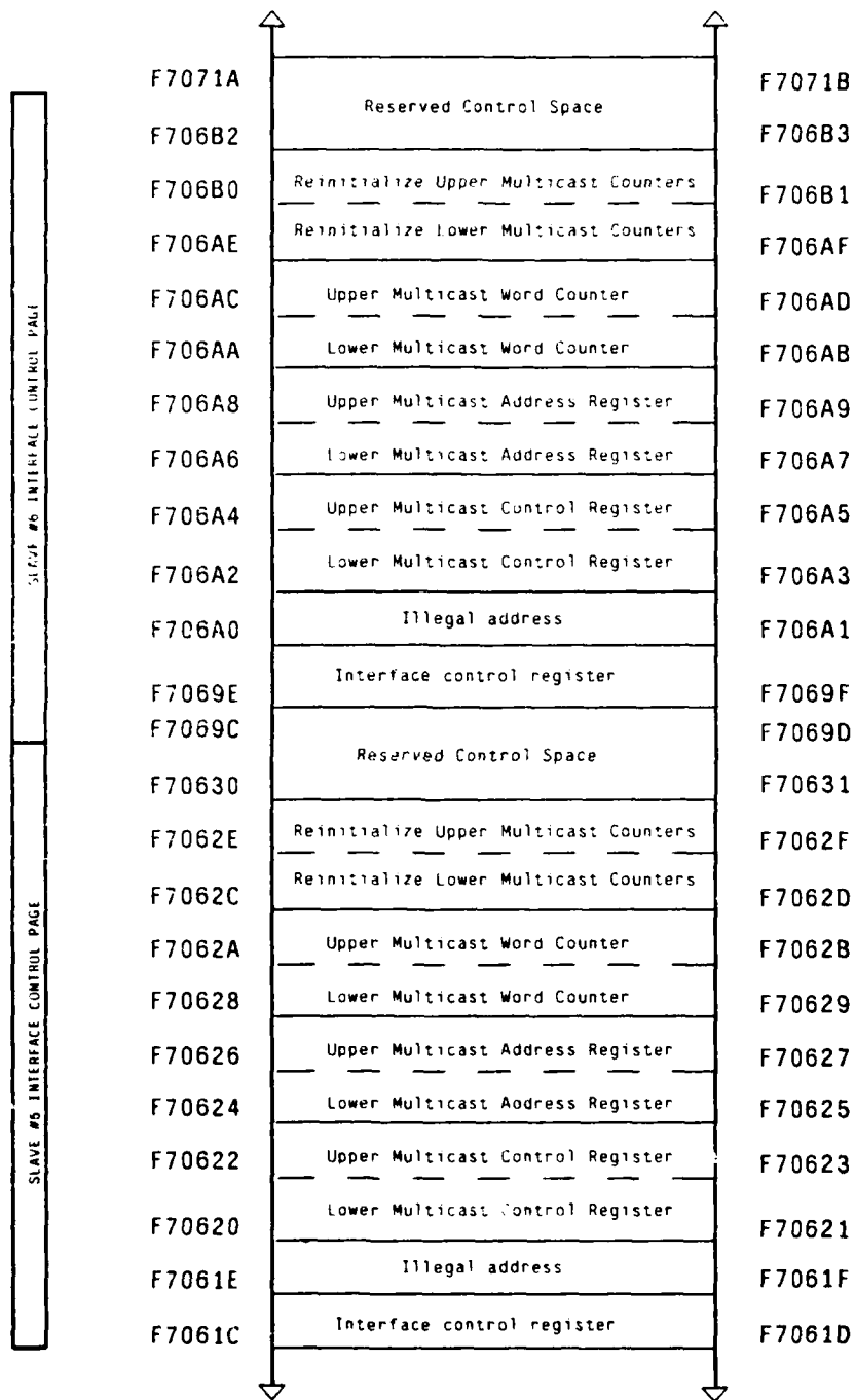
Figure 4-22: Slave #5 and Slave #6 interface control page
