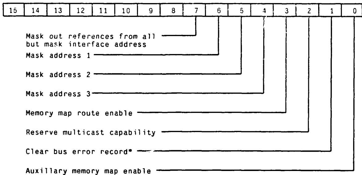
Figure 4-12: Interface control register low byte
