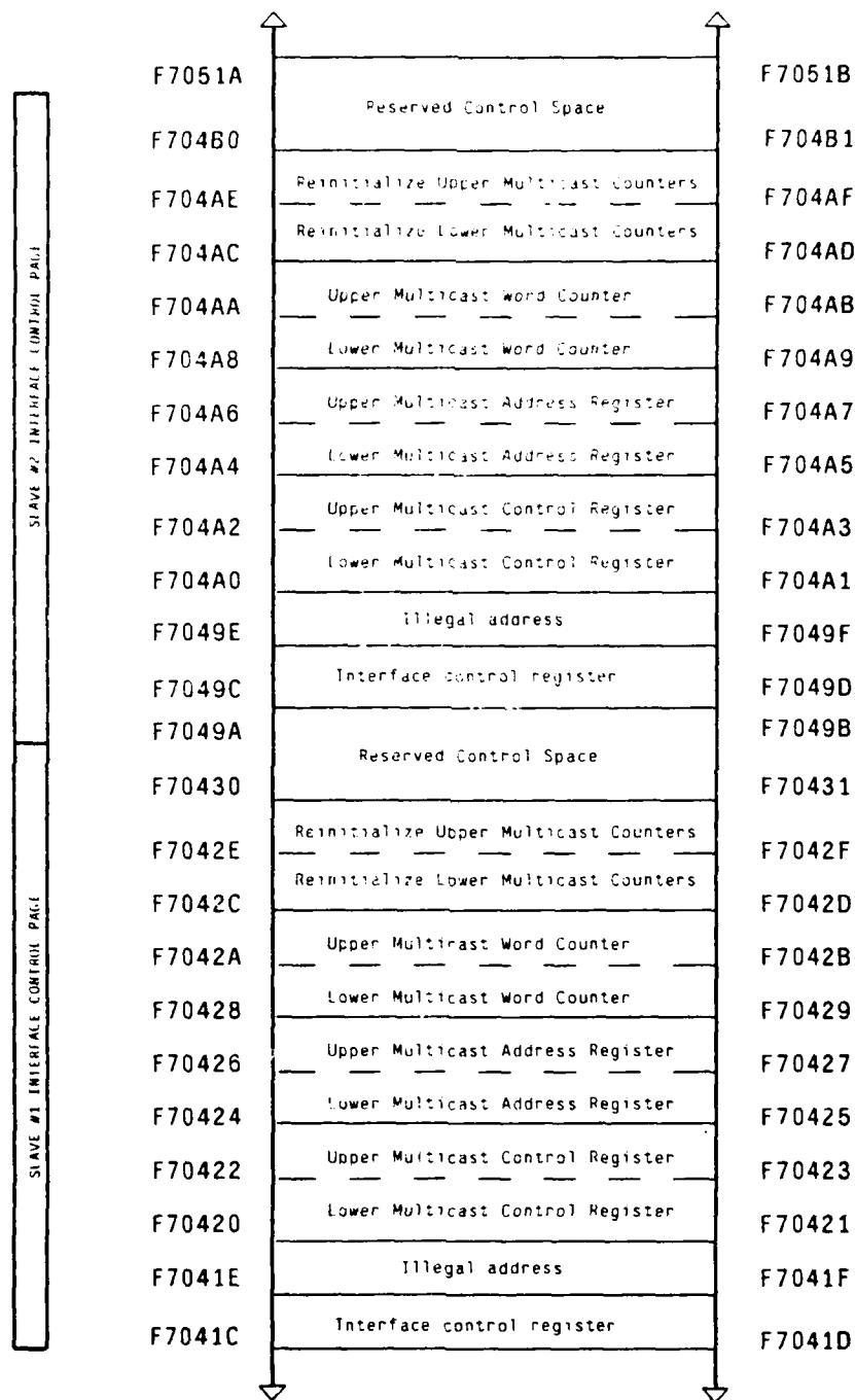
Figure 4-20: Slave #1 and Slave #2 interface control pages
