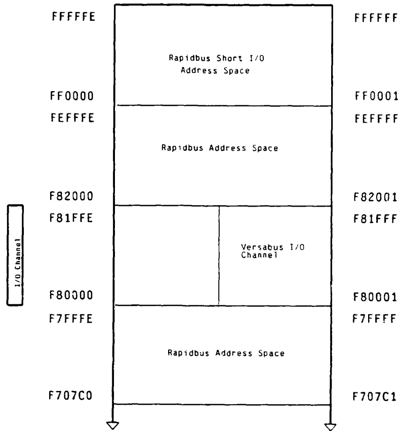
Figure 4-24: I/O and RAPIDbus address space
