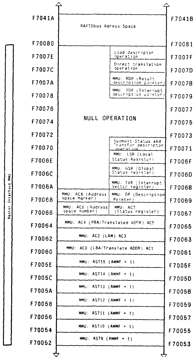
Figure 4-19: Master interface control page [MMU]
