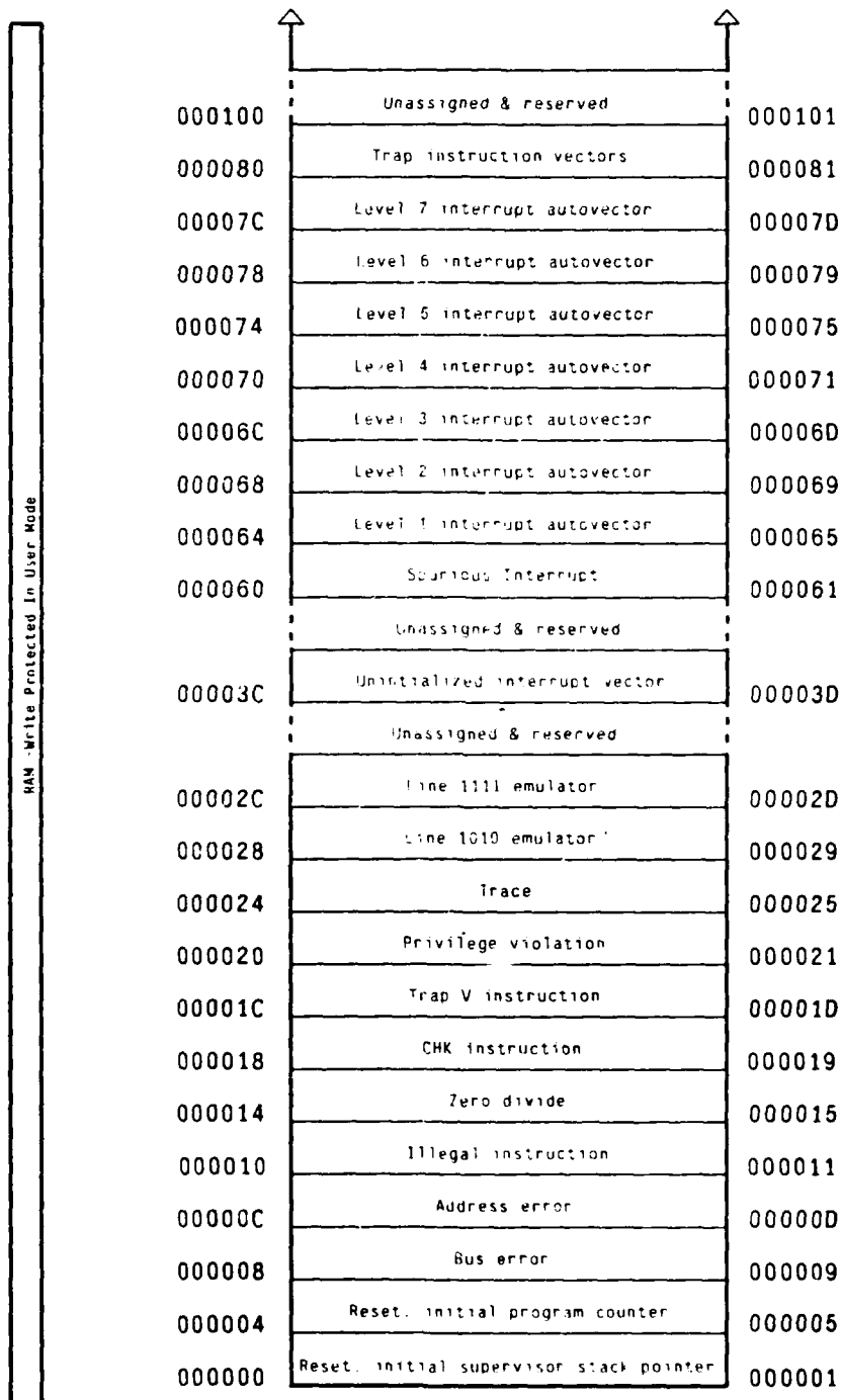
Figure 4-14: Lower RAM supervisor space
