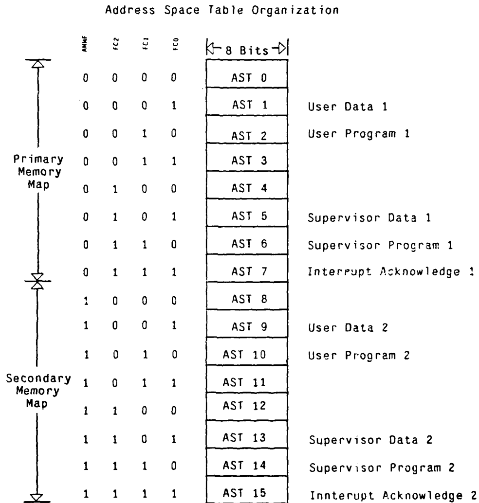
Figure 4-2: The address space tables links the incoming function code and memory map bit from the control register with the cycle address space number [16].
