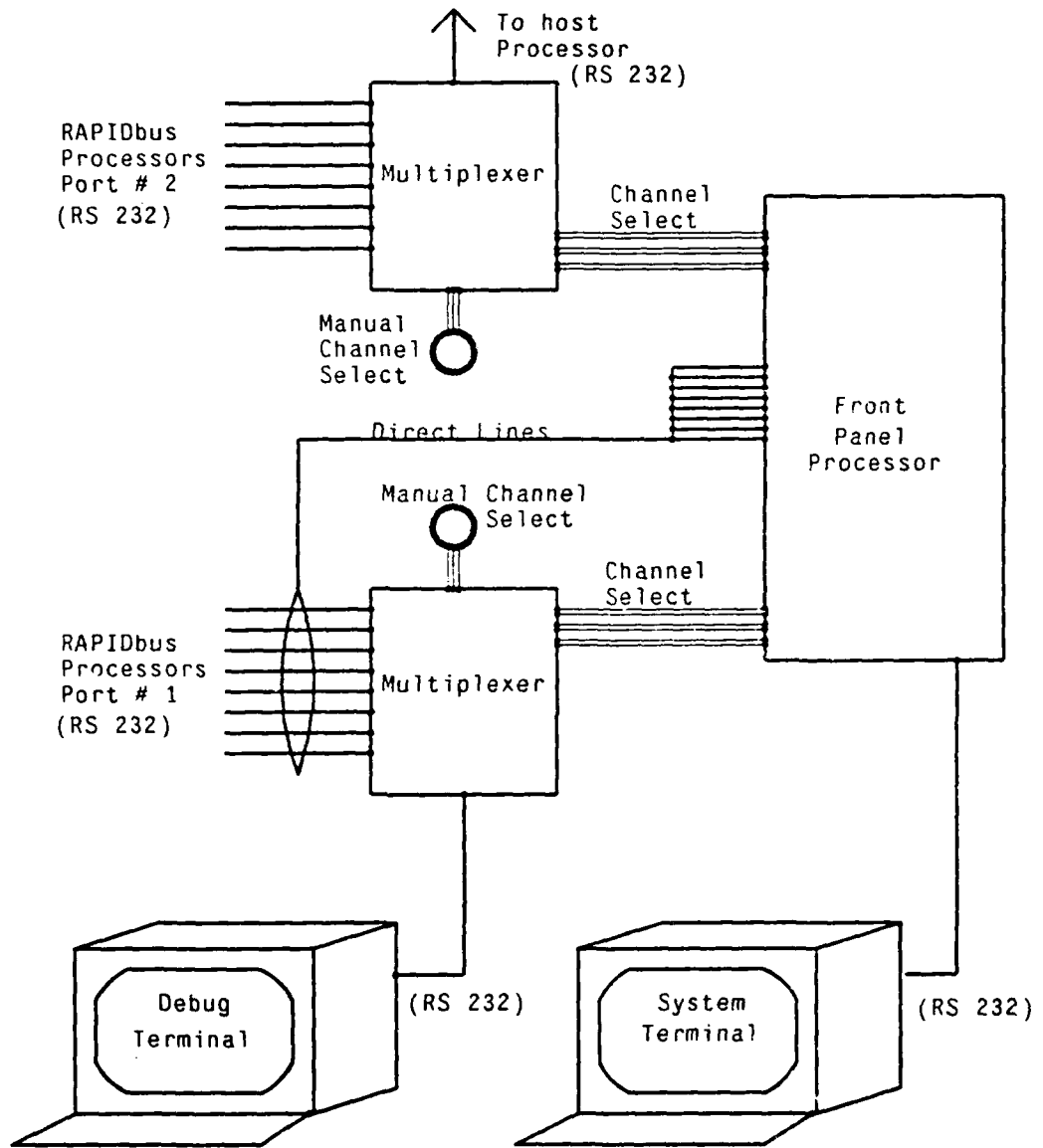
Figure 7-4: The front panel processor simplifies interactions with multiple processors.
