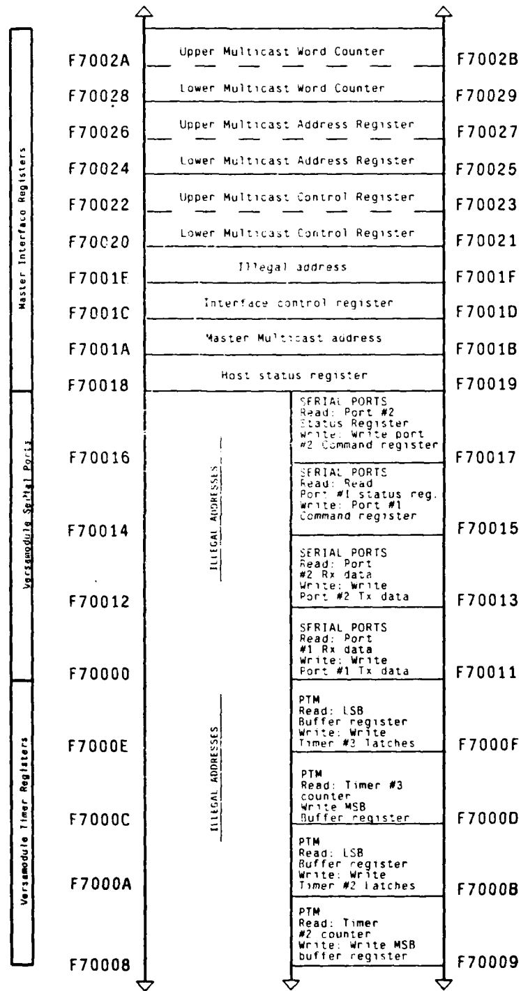
Figure 4-17: Versamodule registers, and master interface control page
