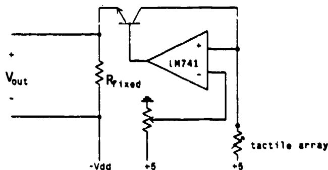
Figure 3-1: resistance to voltage conversion
