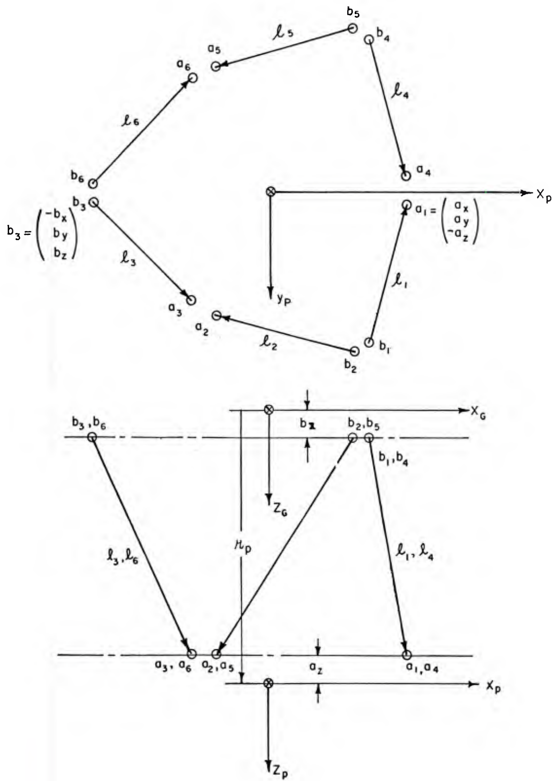
Figure 1. Triogonal system
