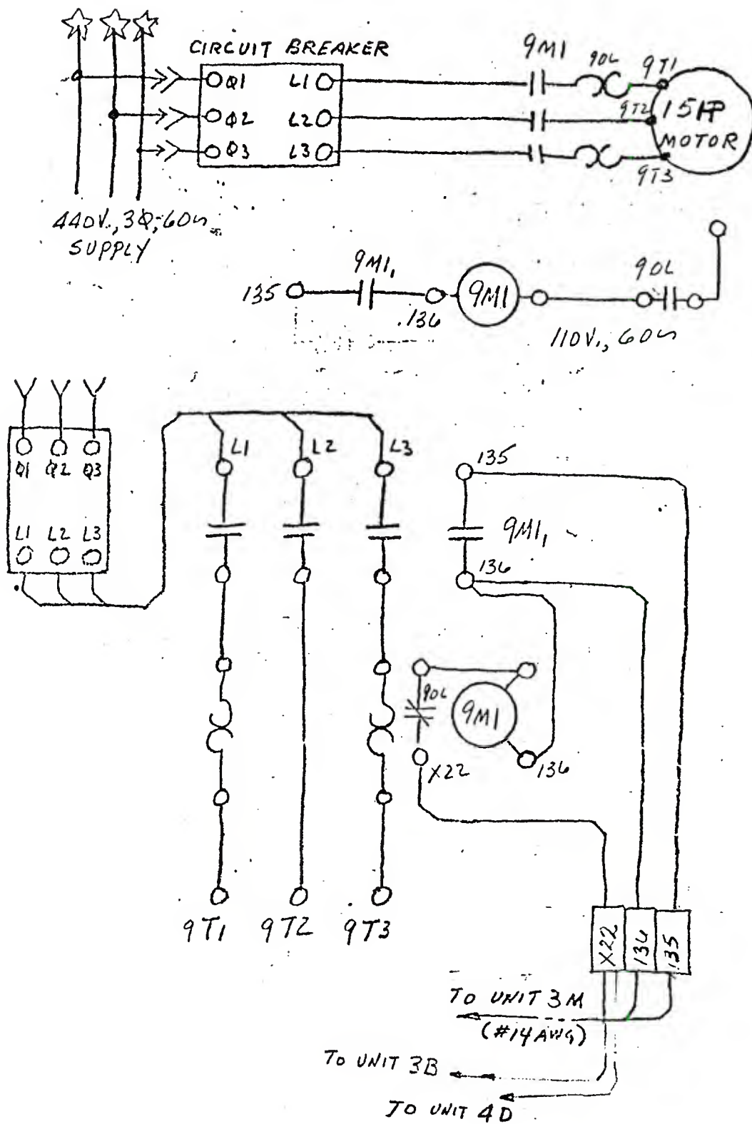
Drawing A-2642. Motor starter - unit 4B (unit 4D)
