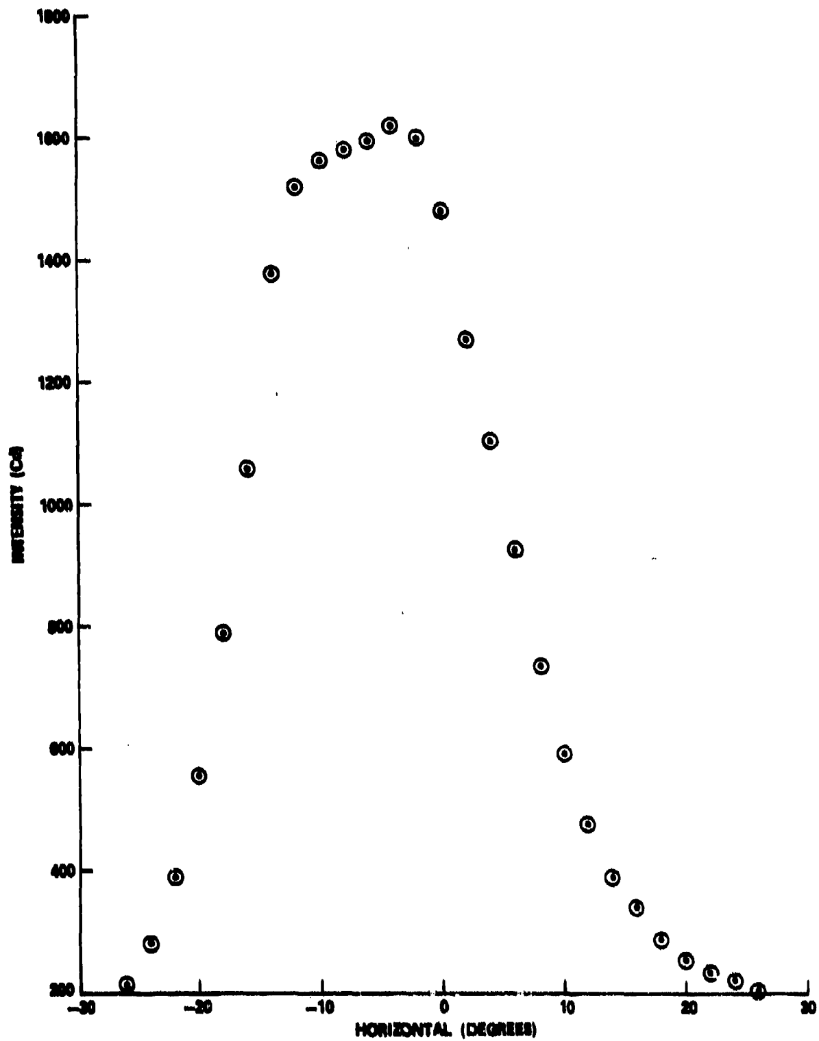
FIGURE 8. PHOTOMETRIC DATA (HORIZONTAL) FOR TAXI-HOLDING POSITION LIGHT WITH 12-INCH DIAMETER LENS
