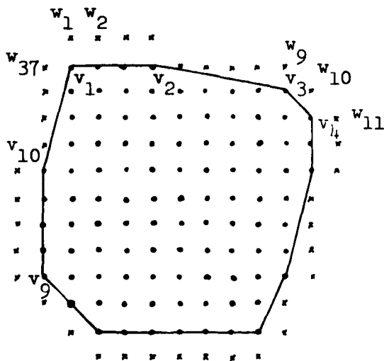
Figure 6. P = \{v_1, v_2, \dots, v_{10}\} and R = \{w_1, w_2, \dots, w_{37}\} , P(v_1, v_3) = \{v_2\} , R(v_1, v_3) = \{w_1, w_2, \dots, w_{10}\} , P(v_3, v_1) = \{v_4, \dots, v_{10}\} and R(v_3, v_1) = \{w_{11}, \dots, w_{37}\} .
