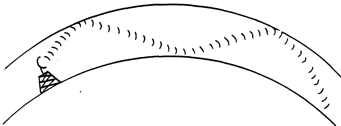
Figure 8. Ducting of Radar Waves and Over-the-Horizon Coverage
