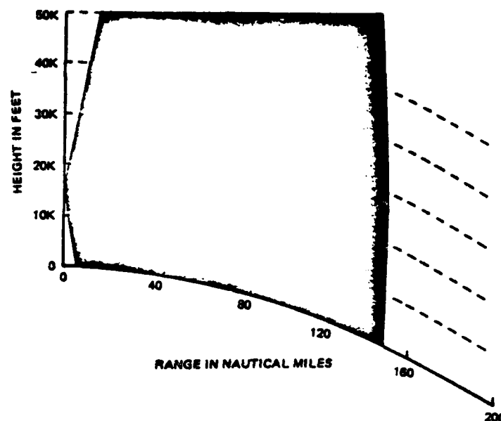
Figure 16. Coverage diagram for typical airborne early-warning radar with 150 nmi free space detection range in the presence of a 15 to 17 kft elevated duct. Radar altitude is 15 kft.
