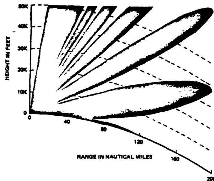
Figure 13. Coverage diagram for the 220 MHz SPS-28 air-search radar at 80 ft for a 1000 ft high surface-based duct and based on a free-space detection range of 100 nmi.
