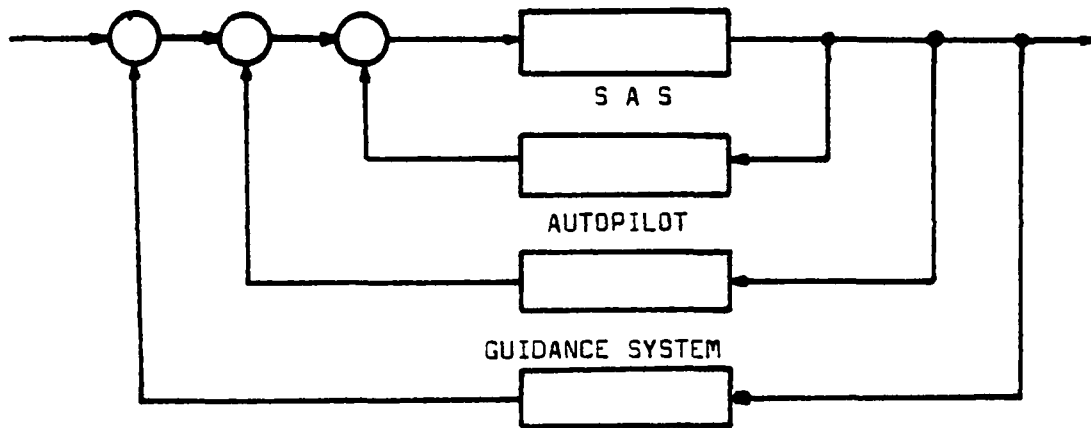
Figure VI.D-3. General Idea of a Guidance System
