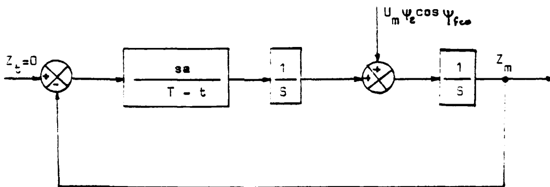
Fig. VII.B-3. Lag-free System with Step Velocity Input
