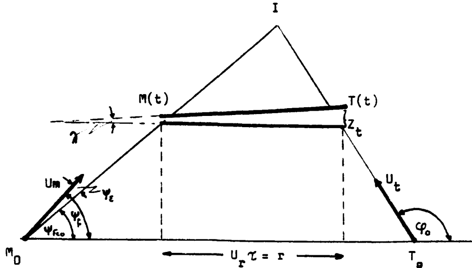
Fig. VII.B-1. Interception Geometry
