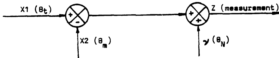
Fig. VI.C-1. Measurement Z contaminated by noise v
