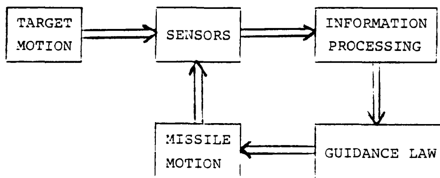
Fig. III.C-1. Structure of information flow in missile guidance loops.
