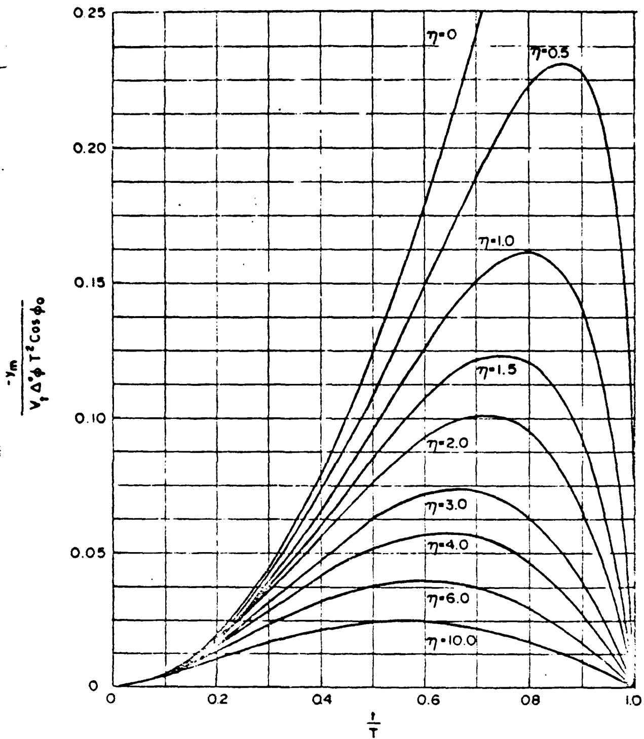
Fig. IV.C-7. Relative Missile Trajectory Caused by Target Maneuver, (see equation IV.C-13) Unlimited Missile, NO Time Lags
