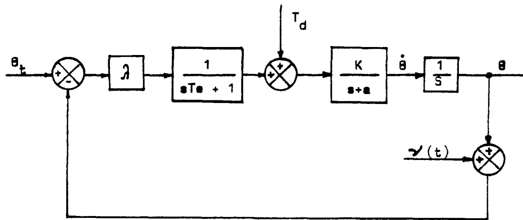
Fig. VI.B-6. Block Diagram of a 3rd Order Tracker
