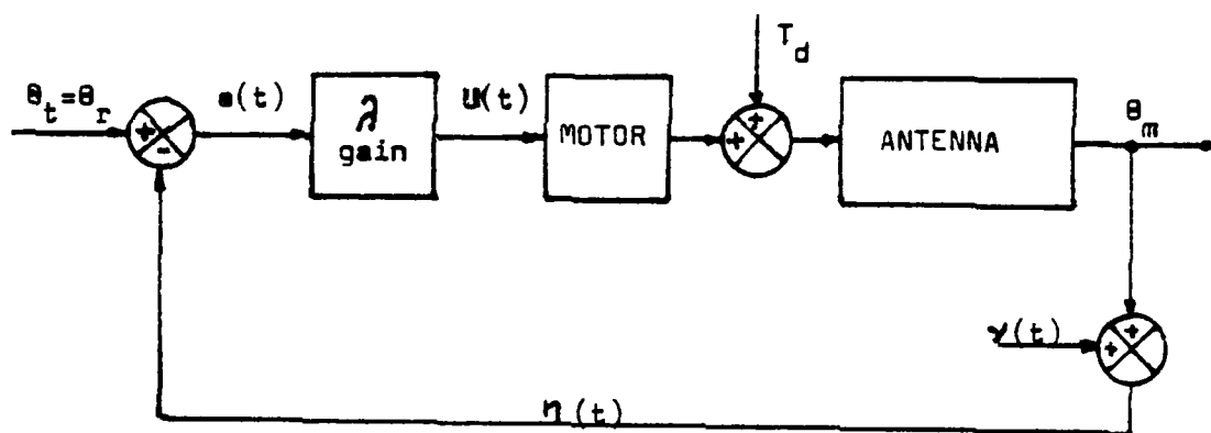
Fig. VI.B-3. Functional Block Diagram of a Tracker
