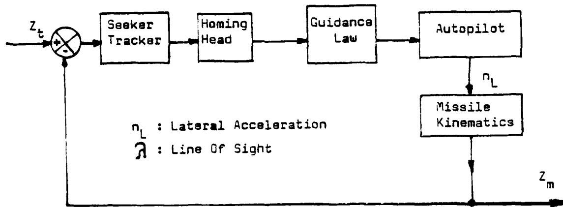
Fig. VII.B-2. Functional Representation of Homing System
