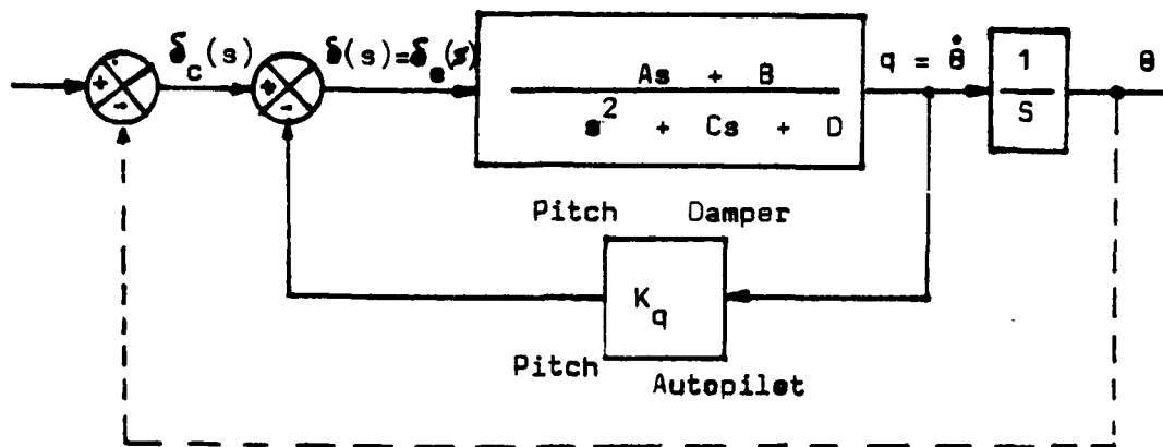
Fig. VI.D-5. Block Diagram of a Pitch Damper
