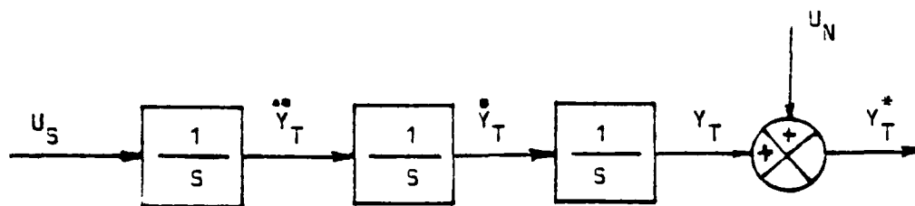
Figure VI.C-2. Kalman Filter Formulation
