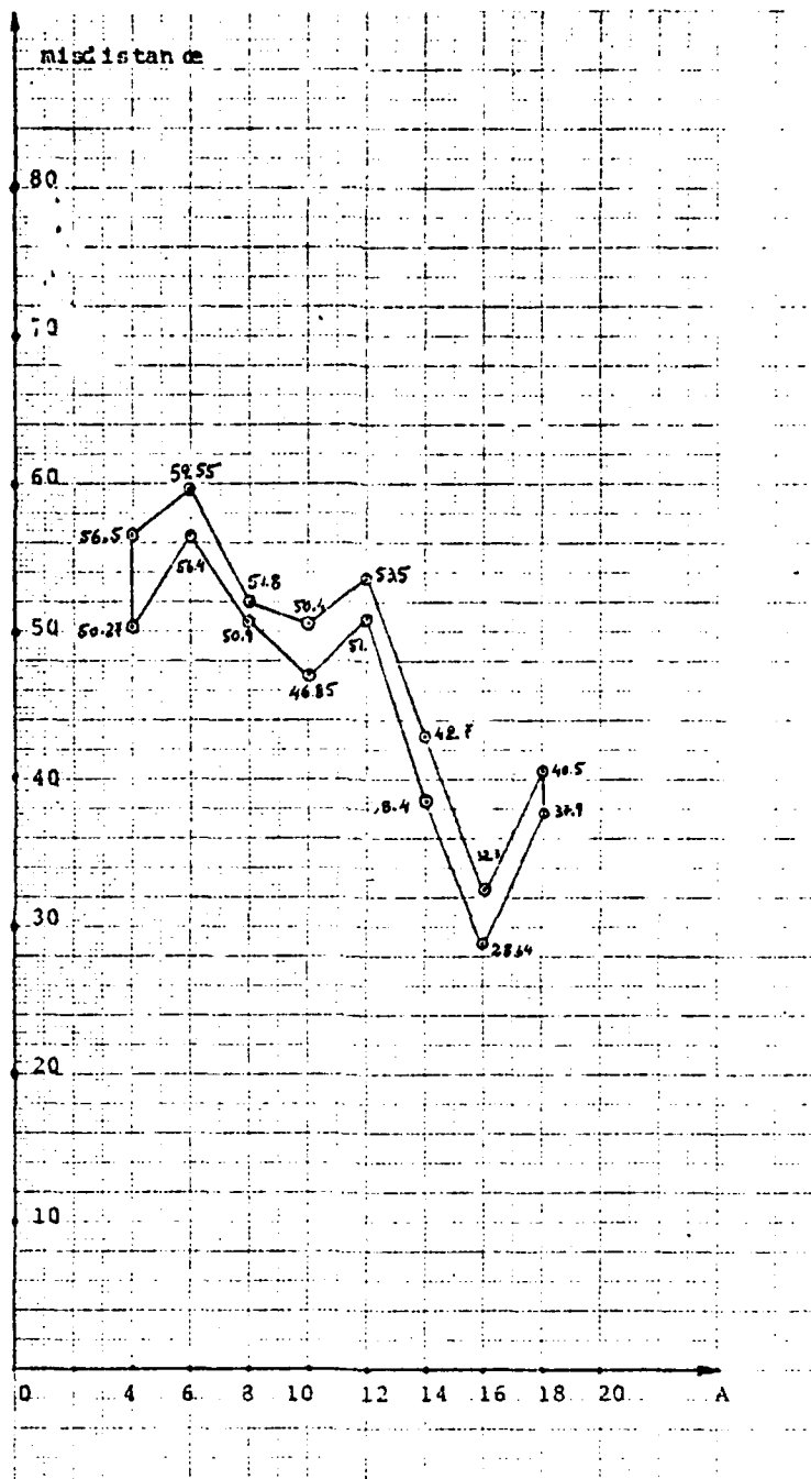
Fig. VII.D-3. MCG Law Utilization. Domain of misdistance variation vs. \hat{t}_{go} ( A = \hat{t}_{go}/t_{go} ) and for filter characteristic frequency \omega_0 = 0.8 . Case of a 2nd order autopilot.
