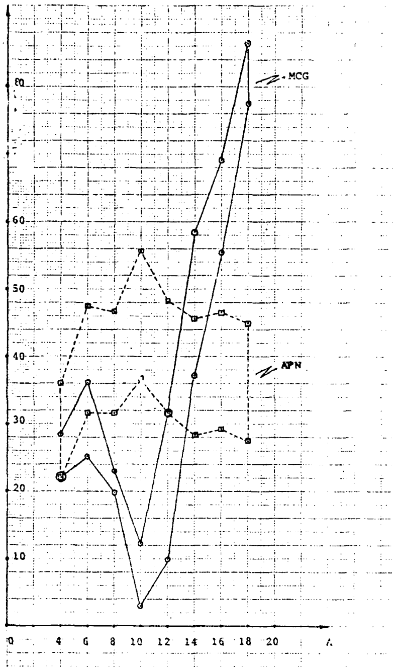
Fig. VII.D-9. Comparison of misdistance variation domain between APN and MCG law, vs. \hat{t}_{go} ( A = \hat{t}_{go}/t_{go} ) and for \omega_0 = 1.2 .
