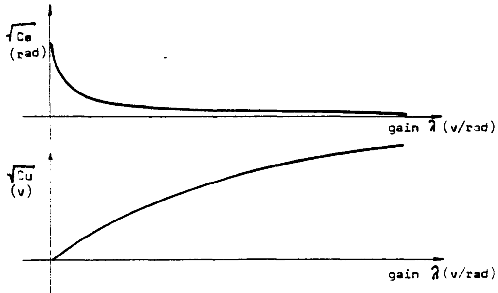
Fig. VI.B-7. rms Tracking Error and rms Input Voltage as Functions of the Gain for a Tracker with Position Servo
