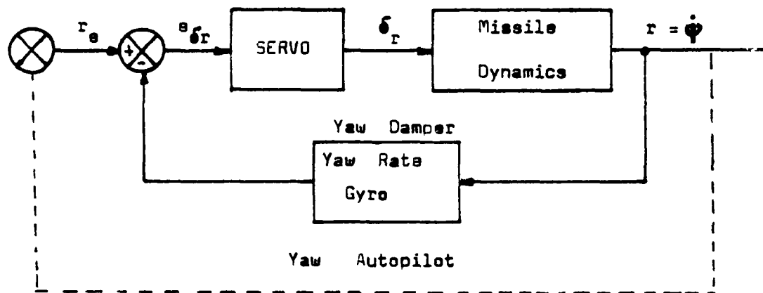
Fig. VI.D-7. Functional Block Diagram of a Yaw Damper
