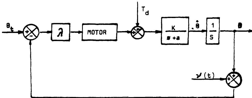
Fig. VI.B-4. Block Diagram of a 2nd Order Tracker
