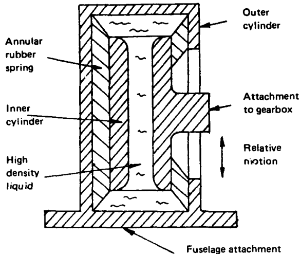
Figure 1. LIVE Isolator
