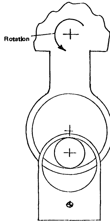
Figure 2. Monofilar Absorber
