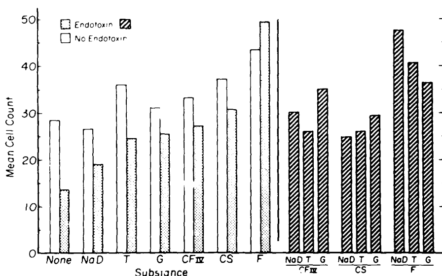
Fig. 11. Histogram of the mean cell count of attached cells. Culture dishes were either coated or uncoated with 12.5 \text{ ng cm}^{-2} of LPS from E. coli . LPS-coated and uncoated dishes were treated for 5 min each with either one mmolar sodium deoxycholate (NaD), one mmolar taurocholic acid (T) or one mmolar glycocholic acid (G) prior to cell incubation. One mmolar solutions of the bile acids were used since it was determined that this concentration was not toxic to the human fibroblasts. Alternatively, LPS-coated or uncoated dishes were treated for 30 min with either 0.15% human plasma fraction IV 1 (Cohn; (CF IV )), human citrated serum (CS), or 50 \mu\text{g ml} human plasma fibronectin (F). The percentage of CF IV was the maximum permissible concentration that could be filtered through a 0.22 \mu\text{m} filter without occluding the pores. Additionally, LPS-coated dishes were pretreated with a combination of bile acid for 5 min, rinsed in pyrogen free water, incubated for 30 min at 37 C either with CF IV , CS, or F and rinsed again thoroughly with pyrogen free water prior to the 90 min incubation with 1.4 \times 10^4 fibroblasts culture dish.
