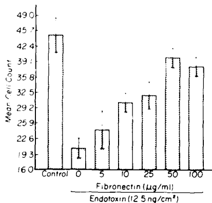
Fig. 6. Histogram of the mean cell count of attached cells: S.E.M. on culture dishes coated with 12.5 ng/cm 2 of LPS from F. nucleatum . LPS-coated dishes were pretreated with plasma fibronectin (5 100 μg/ml) for 30 min at 37 C prior to the 90 min incubation with 1.88 \times 10^4 fibroblasts/culture dish.
