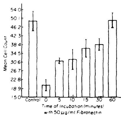
Fig. 10. Histogram of mean cell count of attached cells \pm SEM on culture dishes coated with 12.5 ng/cm 2 of LPS from E. nucleatum . LPS-coated culture dishes were pretreated with 50 \mu\text{g/ml} plasma fibronectin for 5-60 min at 37 C prior to the 90 min incubation with 1.88 \times 10^4 fibroblasts culture dish.
