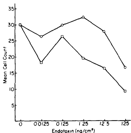
Fig. 5. Each point was the mean cell count of 12 determinations (3 from each of 4 culture dishes). Each determination was an exact count of attached cells in a 4 mm 2 area on the tissue culture dish. B. melaninogenicus LPS-coated culture dishes, \circ ; F. nucleatum LPS-coated culture dishes \square .
