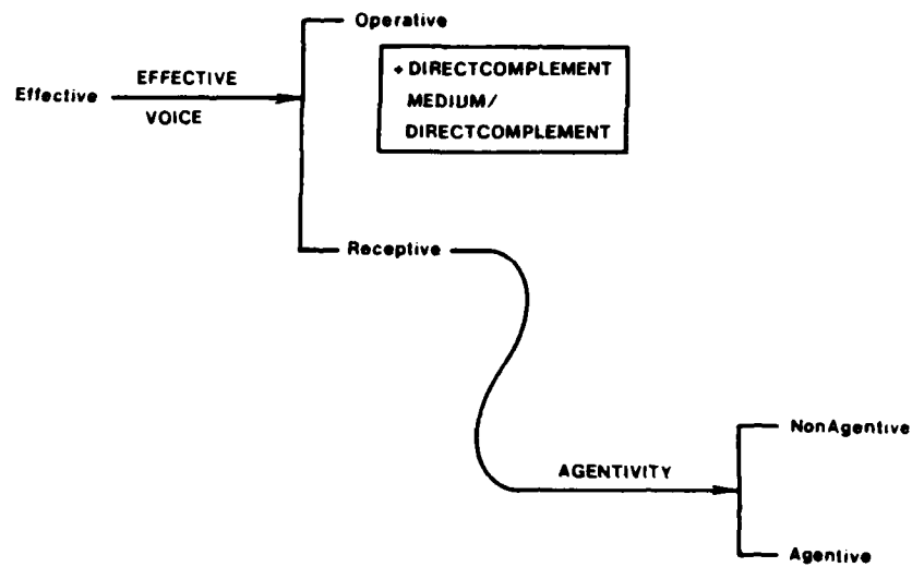
Figure 2-12: Clause voice
