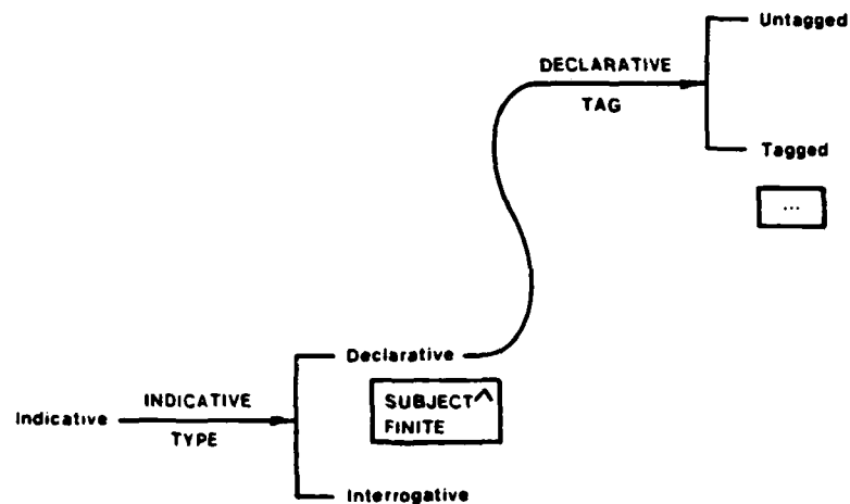
Figure 2-17: Mood II
