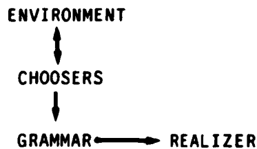
Figure 2-1: Role interactions
