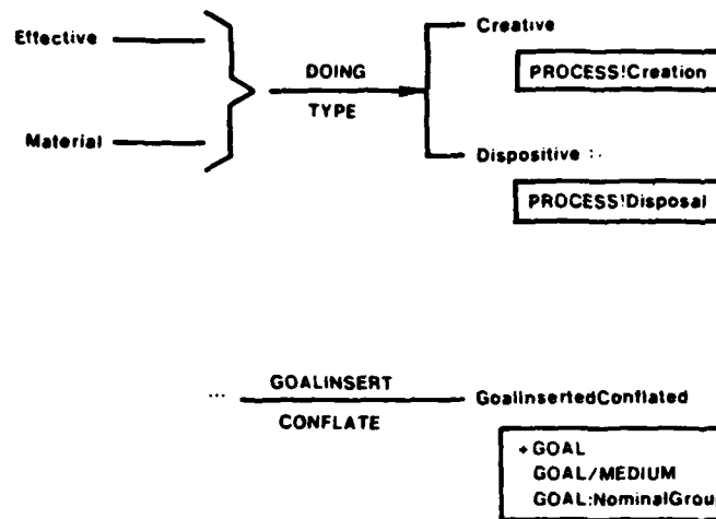
Figure 2-10: Transitivity II
