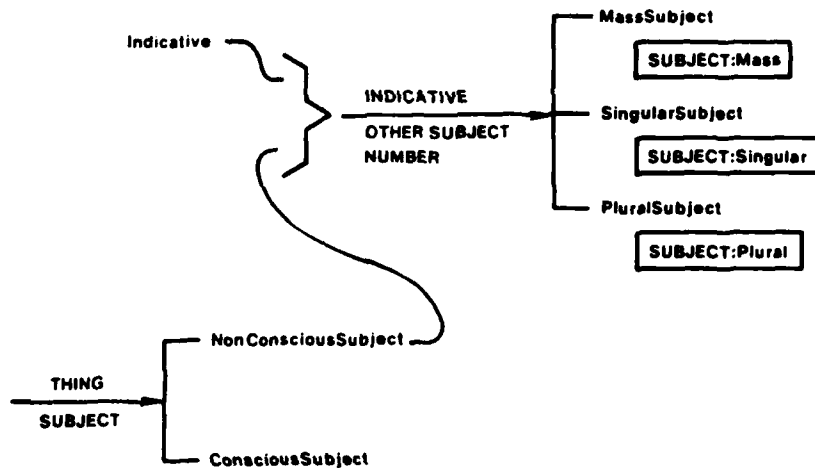
Figure 2-25: Subject person
