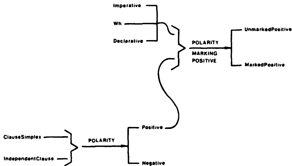
Figure 2-23: Polarity
