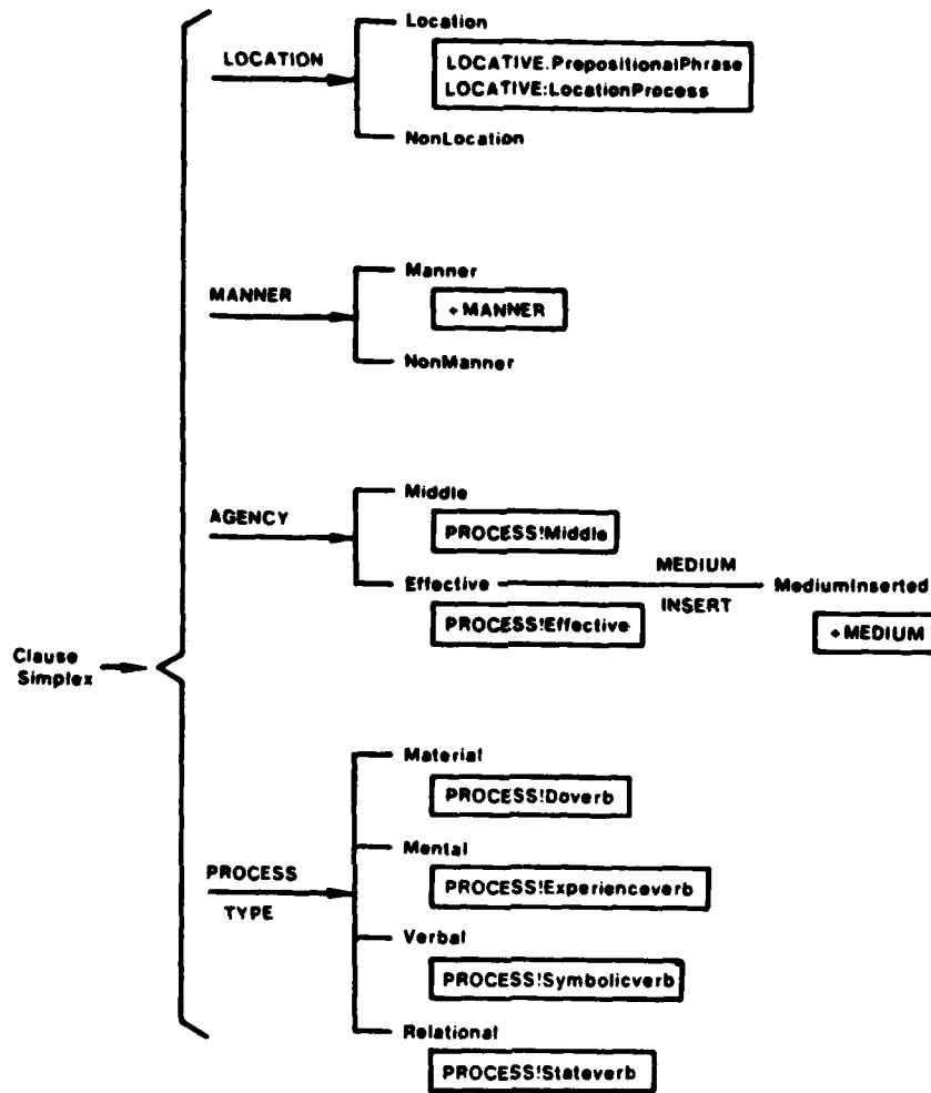
Figure 2-8: Transitivity I
