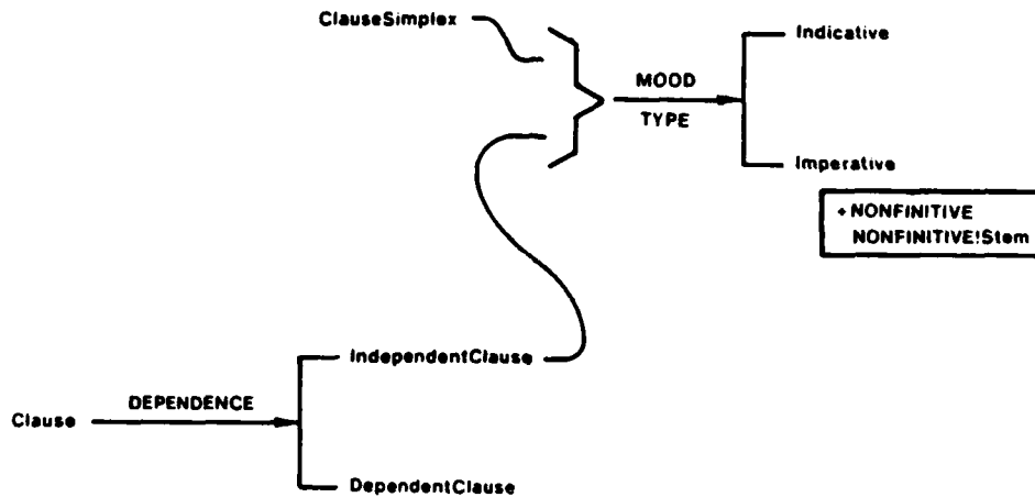
Figure 2-15: Mood I
