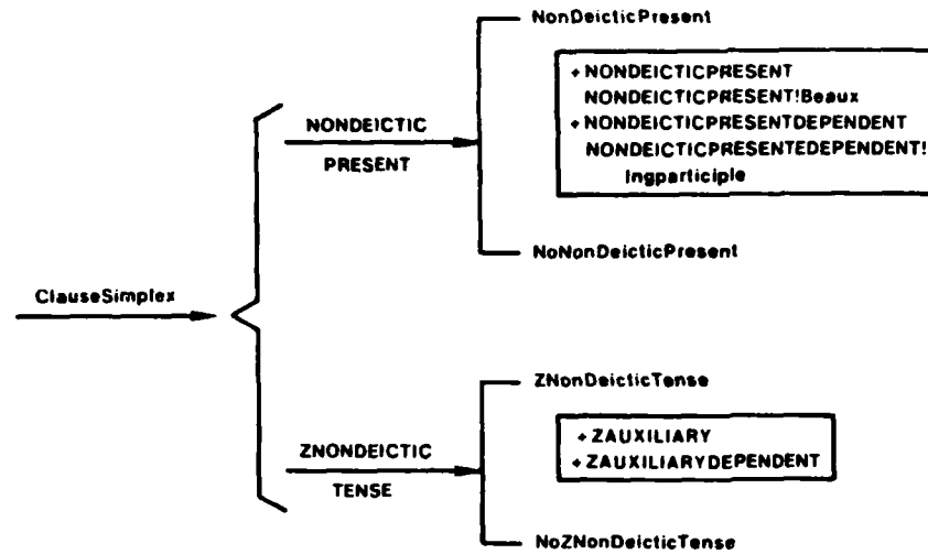
Figure 2-7: Secondary tense
