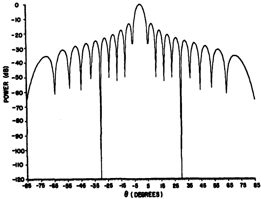
Fig. 9b — One-way antenna pattern when 20 static unweighted elements spaced \lambda/2 apart are used in transmit
