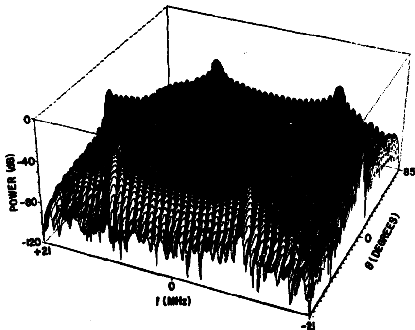
Fig. 5 — One-way response when ten unweighted elements spaced \lambda/2 apart are moved through 20 elements during a 1\text{-}\mu\text{s} unweighted transmit pulse
