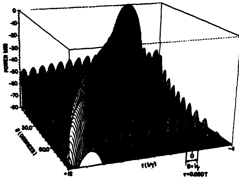
Fig. 3 — One-way response when 20 unweighted elements are moved through 20 elements during a Hamming-weighted transmit pulse
