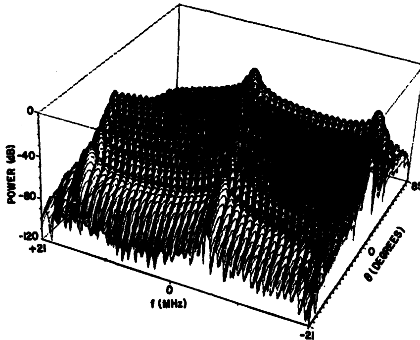
Fig. 7 — One-way response when ten unweighted elements spaced \lambda/4 apart are moved through 20 elements during 1- \mu s unweighted transmit pulse
