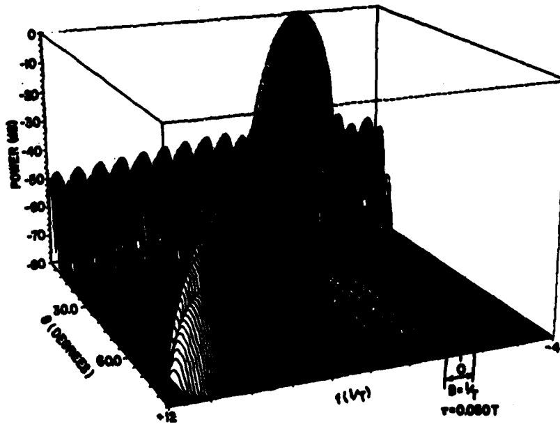
Fig. 4 — One-way response when 20 Hamming-weighted elements are moved through 20 elements during a Hamming-weighted transmit pulse
