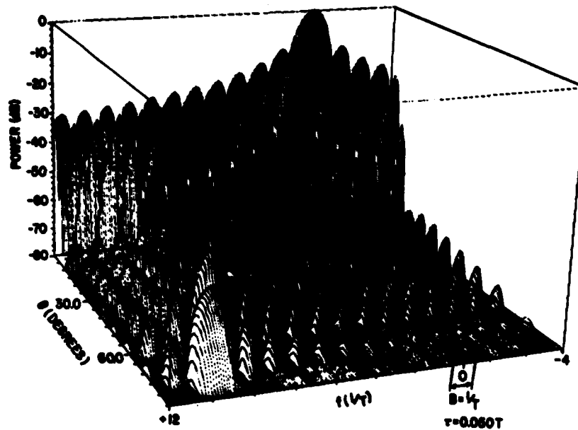
Fig. 2 — One-way response when 20 Hamming-weighted elements are moved through 20 elements during an unweighted transmit pulse
