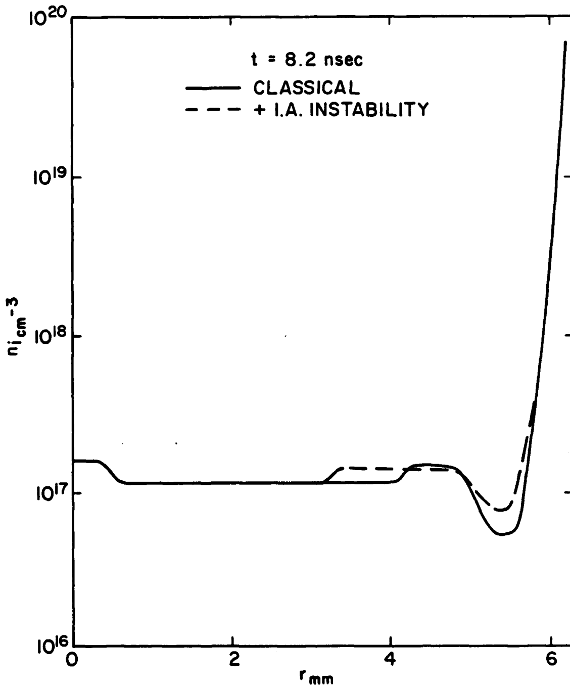
Fig. 1. Plasma channel density profiles with and without ion-acoustic instability for j_b = 10^7 A/cm 2 , n_0 = 4 \times 10^{17} cm -3 and \epsilon_b = 2 MeV at t = 8.2 nsec.
