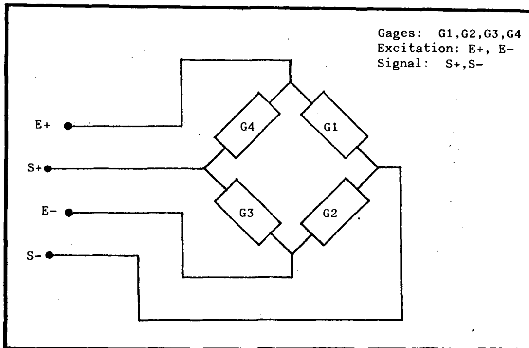
Figure 17. Strain Gage Bridge Configuration
