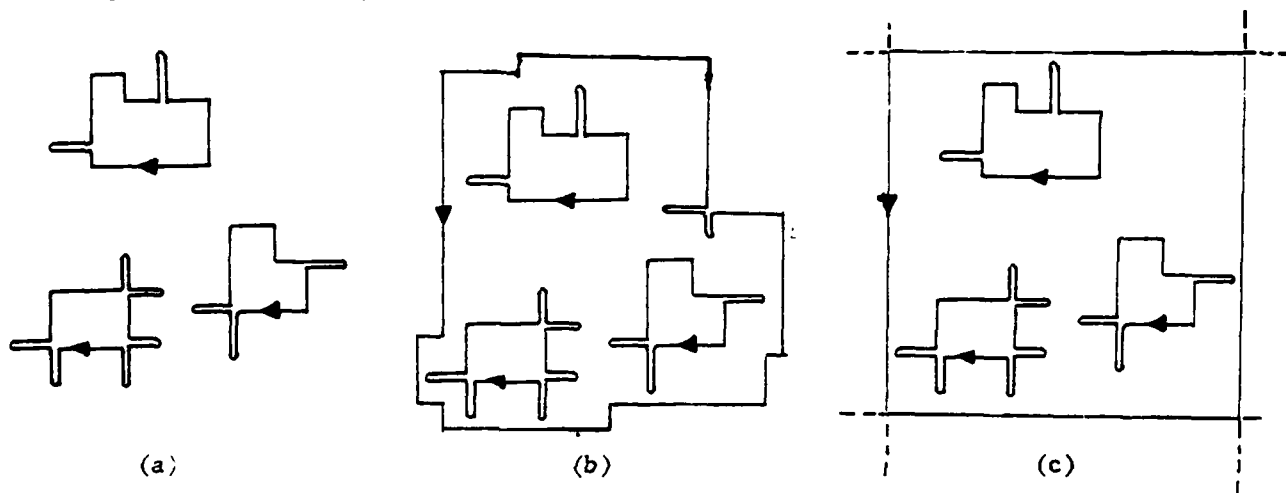
Figure 7. Types of boundaries of nontrivial regions
