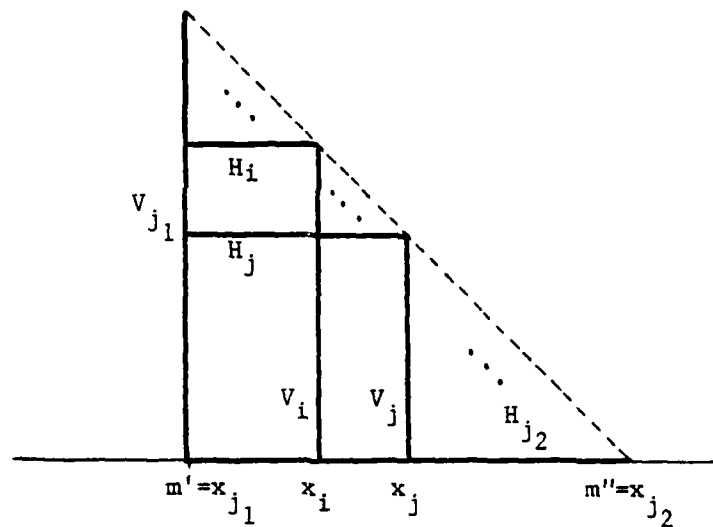
Figure 8. To show that SORTING is transformable to EXTERNAL CONTOUR.
