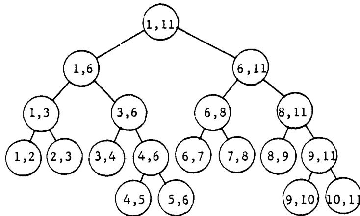
Figure 2. Illustration of T(1, 11) .
