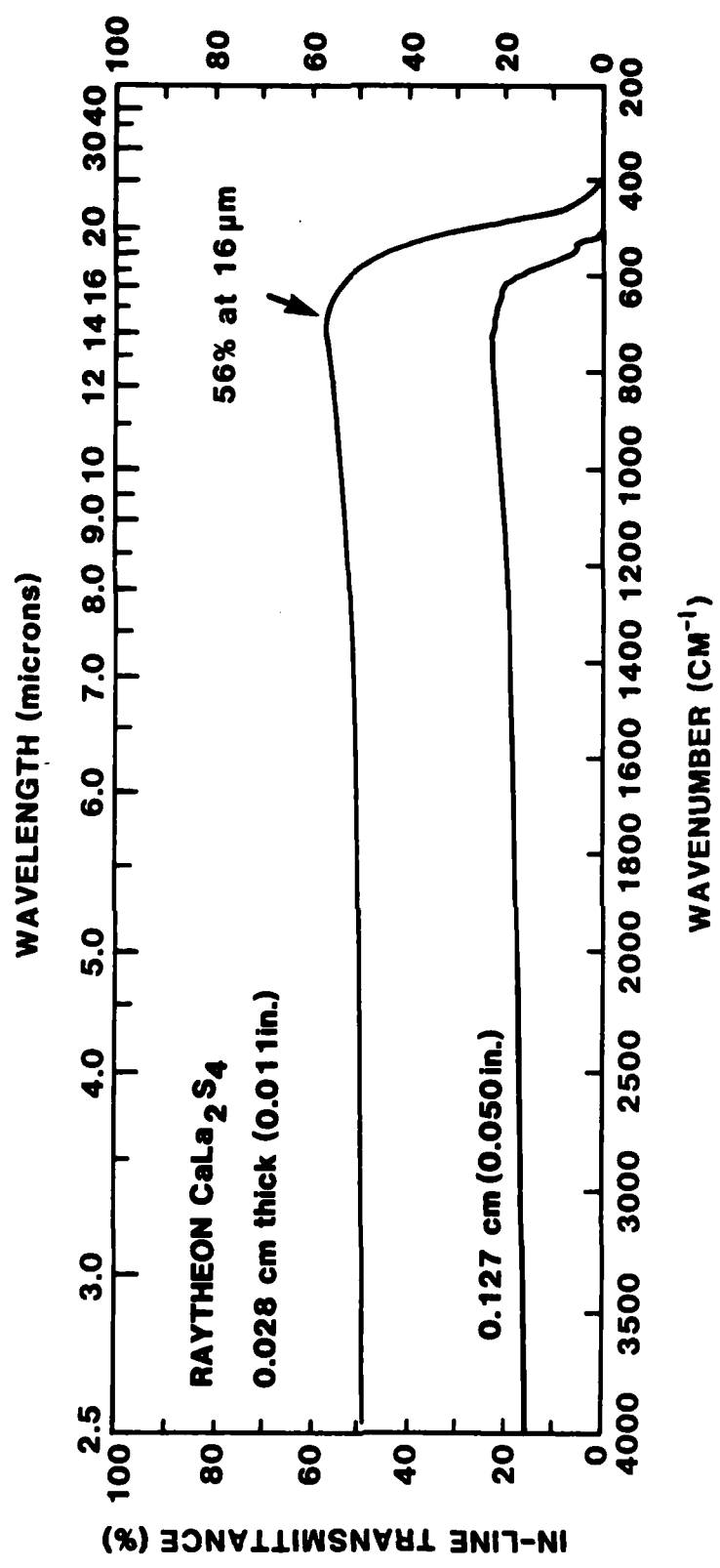
Figure 5. Transmittance results for CaLa 2 S 4 at thicknesses of 0.028 and 0.127 cm.
