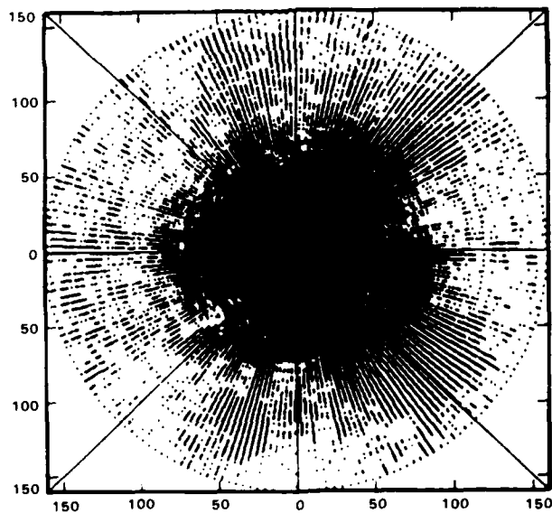
Fig. 3.11c. Comparison of NSSL and M.I.T. clutter data at 0.4^\circ elevation angle.
