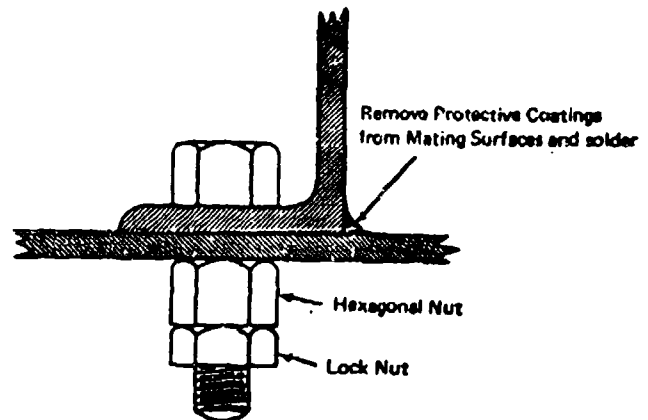
Figure 5-13. Acceptable Bonding Technique Using Bolts
