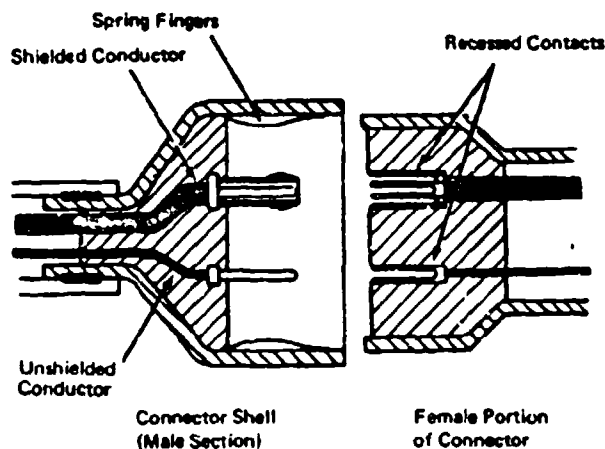
Figure 5-9. Multi-Coaxial Connector Design
