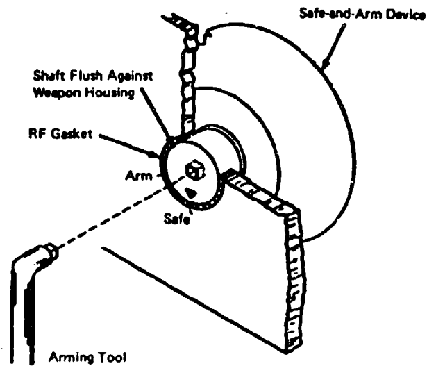
Figure 5-20. Acceptable Method of Shielding Safe and Arm Devices
