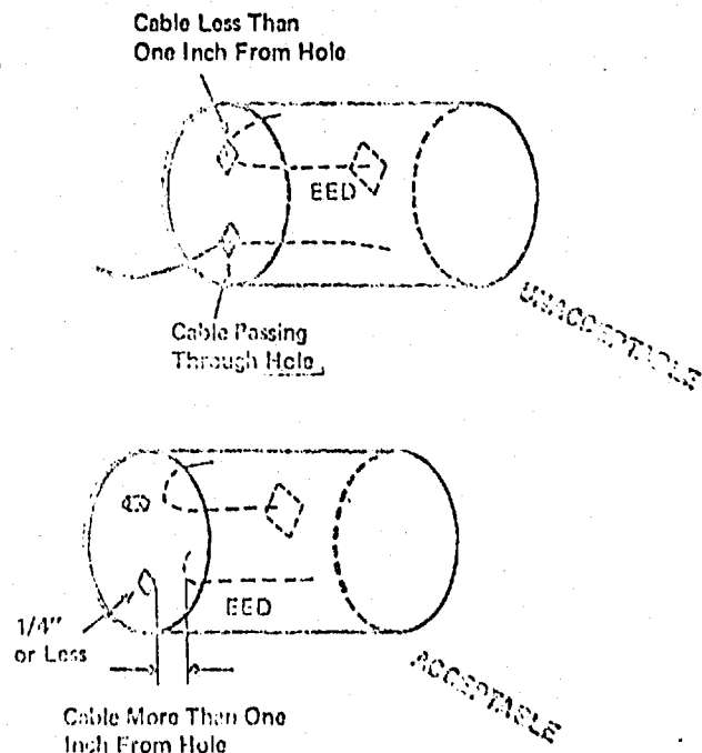
Figure 4-5. Holes in Partially Shielded Weapon Sections
