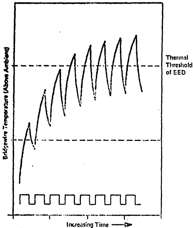
Figure 3-2. Temperature Increase Due to Thermal Stacking
