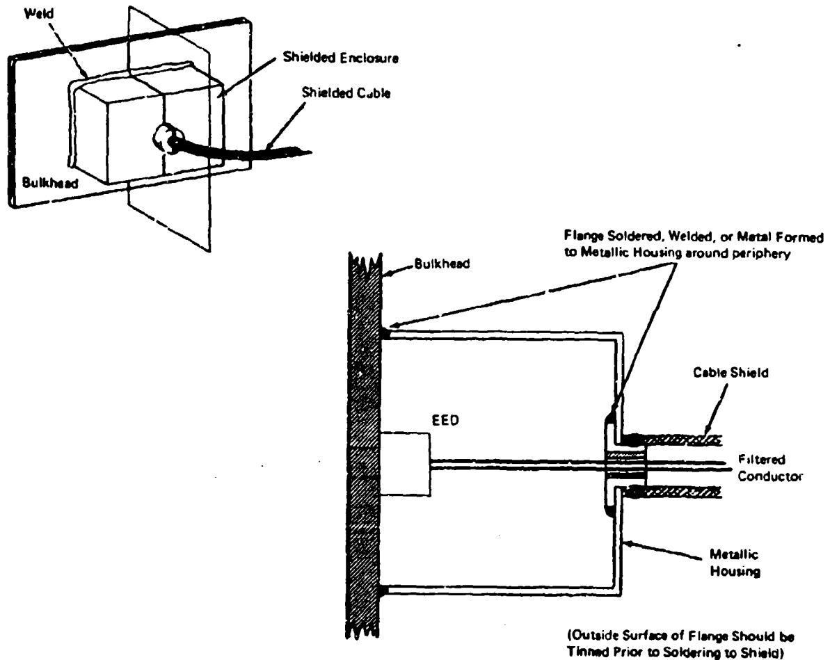
Figure 5-10. Acceptable Method of Routing Rigid Cable Through Shielded Enclosure
