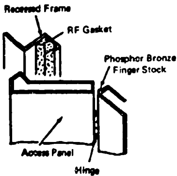
Figure 5-17. Acceptable Methods for Temporary Aperture Design
