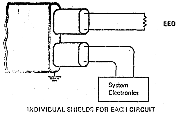
INDIVIDUAL SHIELDS FOR EACH CIRCUIT
