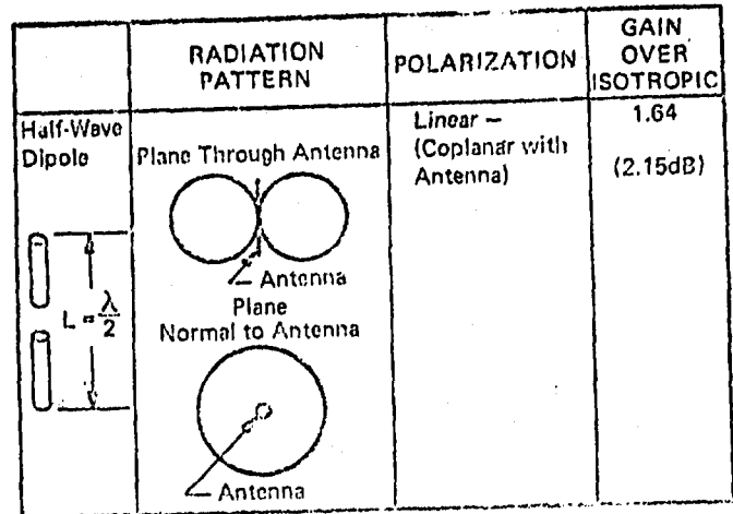
Figure 2-7. Characteristics of a Half-Wave Dipole
