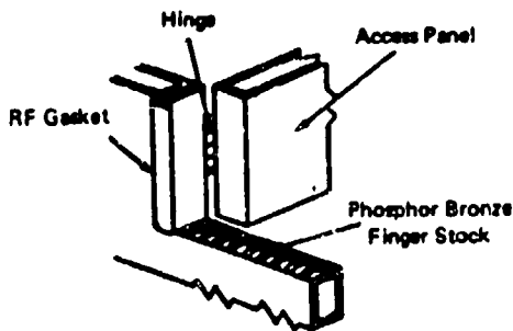
Figure 5-17. Acceptable Methods for Temporary Aperture Design
