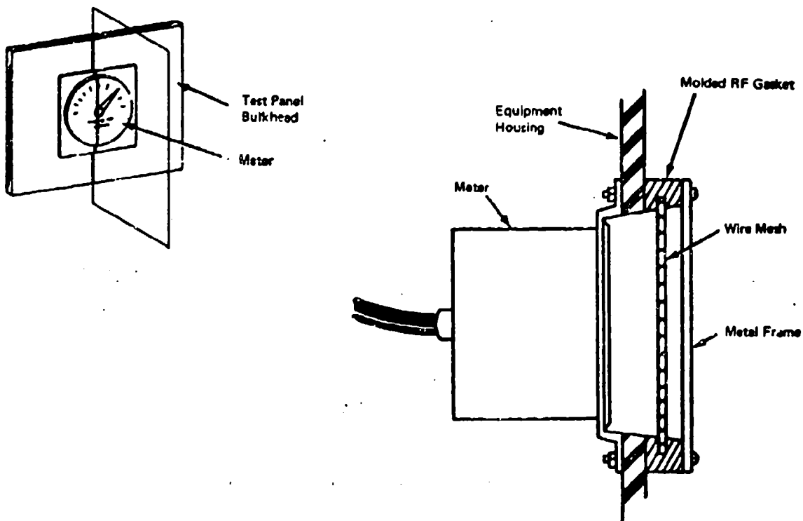
Figure 5-19. Acceptable Method of Shielding Panel-Mounted Meters
