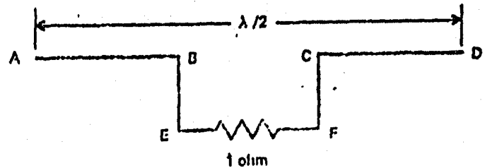
Figure 2-10. An EED Matched to a Dipole Antenna
