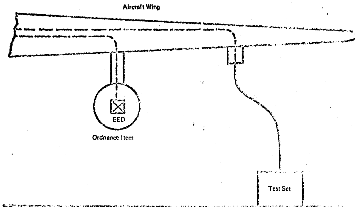
Figure 4-15. Unacceptable Use of Test Set
