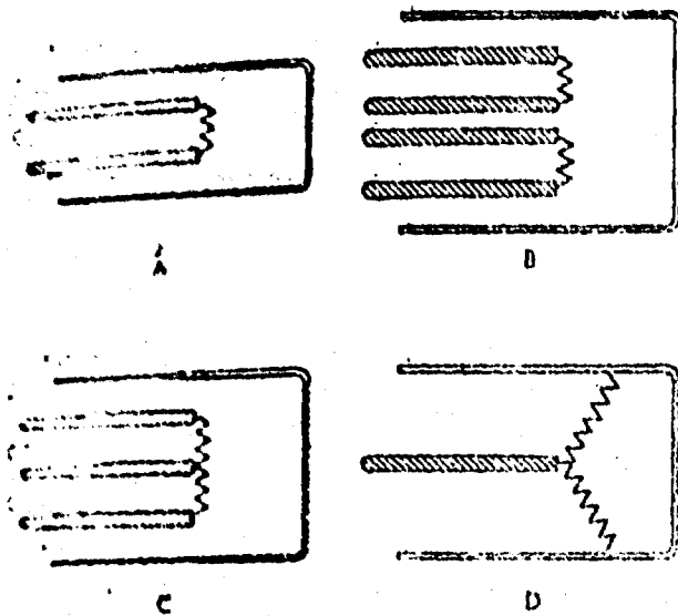
Figure 3-6. Four Types of Hot Bridgewire (HBW) EEDs
