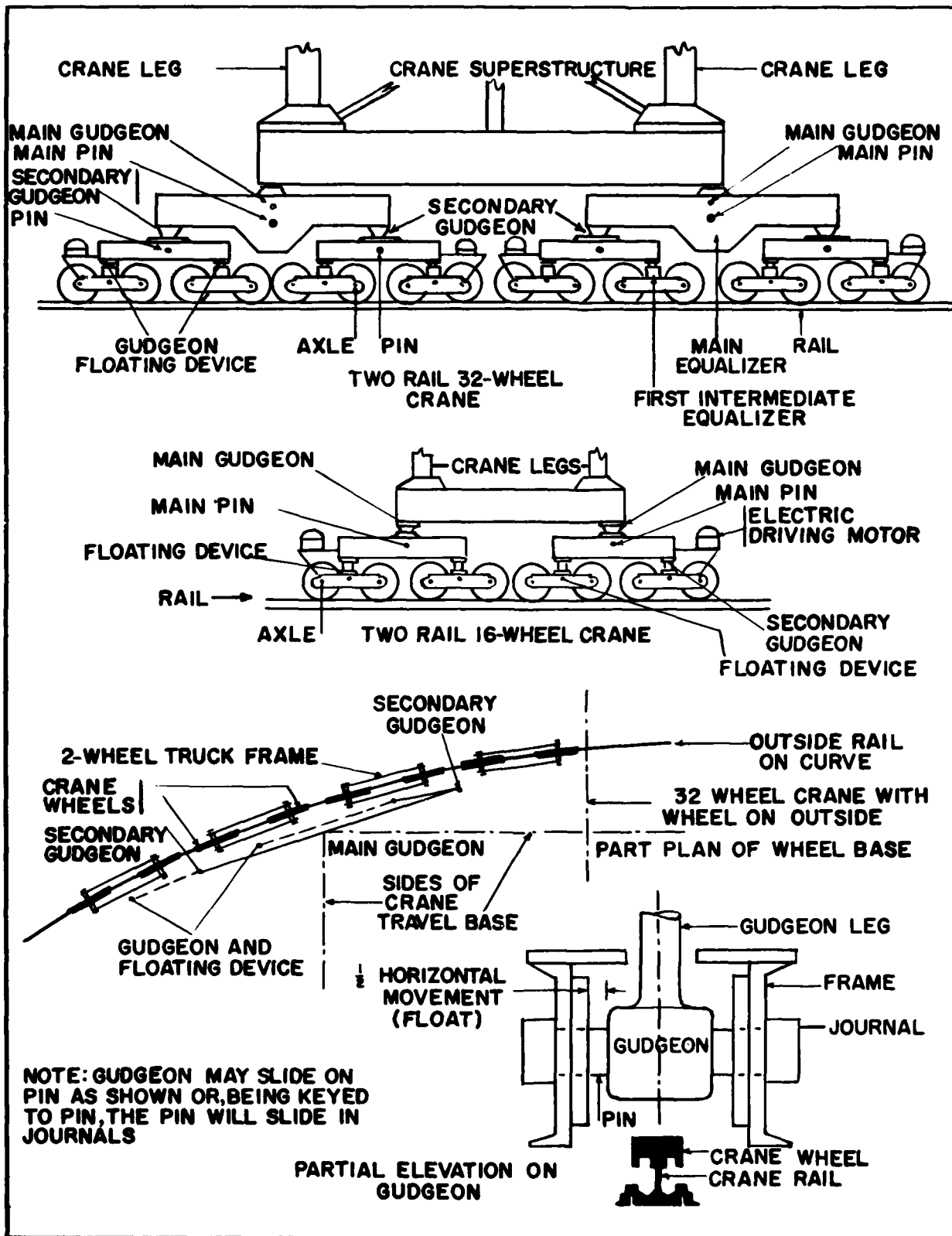
FIGURE 3 Travel Bases for Cranes
