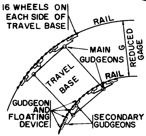
32-WHEEL CRANE TRAVEL BASE PLAN ON CURVE RAIL
