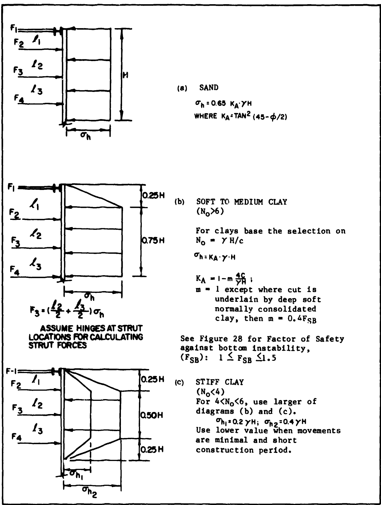
FIGURE 26 Pressure Distribution for Brace Loads in Internally Braced Flexible Walls
