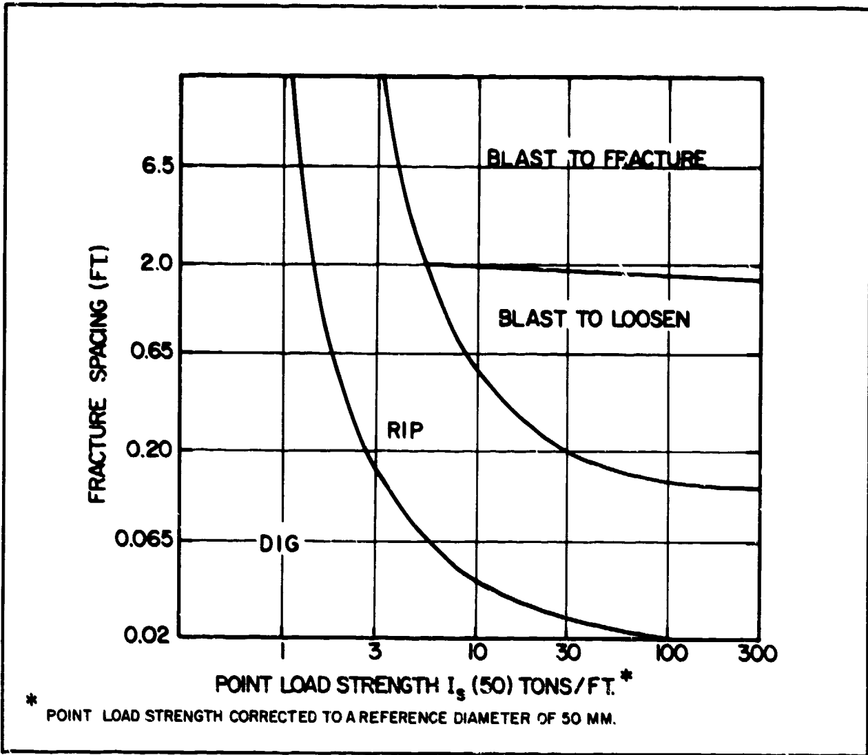
FIGURE 9 Suggested Guide for Ease of Excavation
