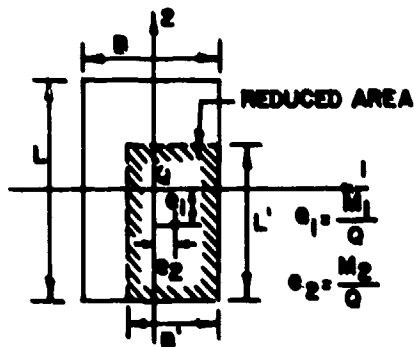
(B) REDUCED AREA-RECTANGULAR FOOTINGS
