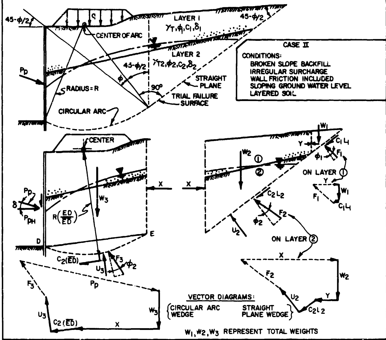
FIGURE 9 Computation of General Passive Pressures 7.2-71
