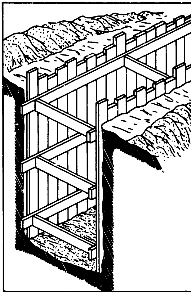
Requirements for Close Sheetting
