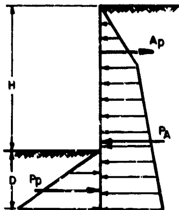
LOAD DIAGRAM
