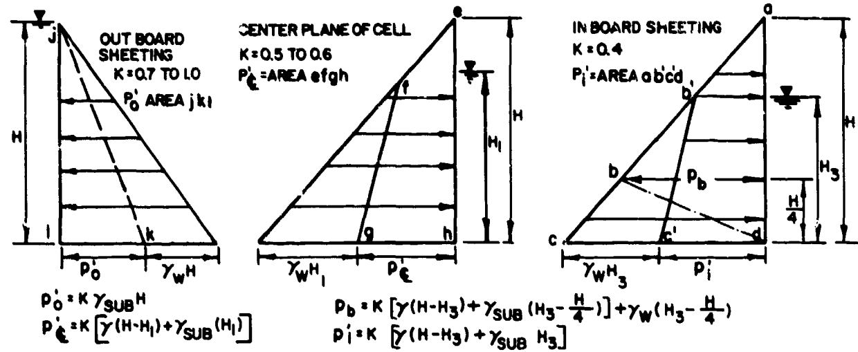
FIGURE 27 Design Criteria for Cellular Cofferdams 7.2-119
