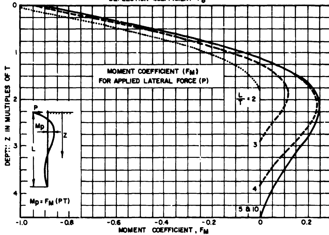
FIGURE 12 Influence Values for Laterally Loaded Pile (Case II. Fixed Against Rotation at Ground Surface) 7.2-239
