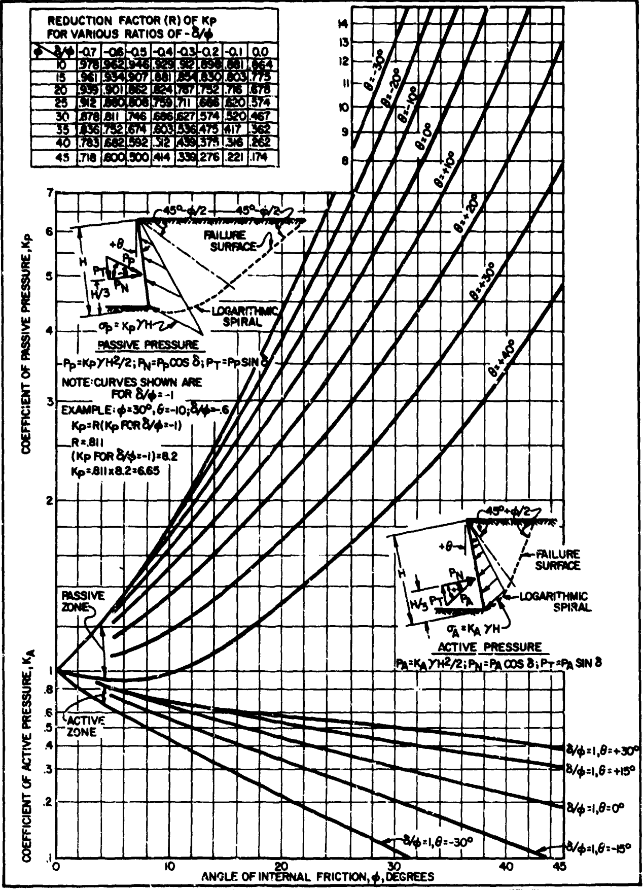
FIGURE 5 Active and Passive Coefficients with Wall Friction (Sloping Wall)
