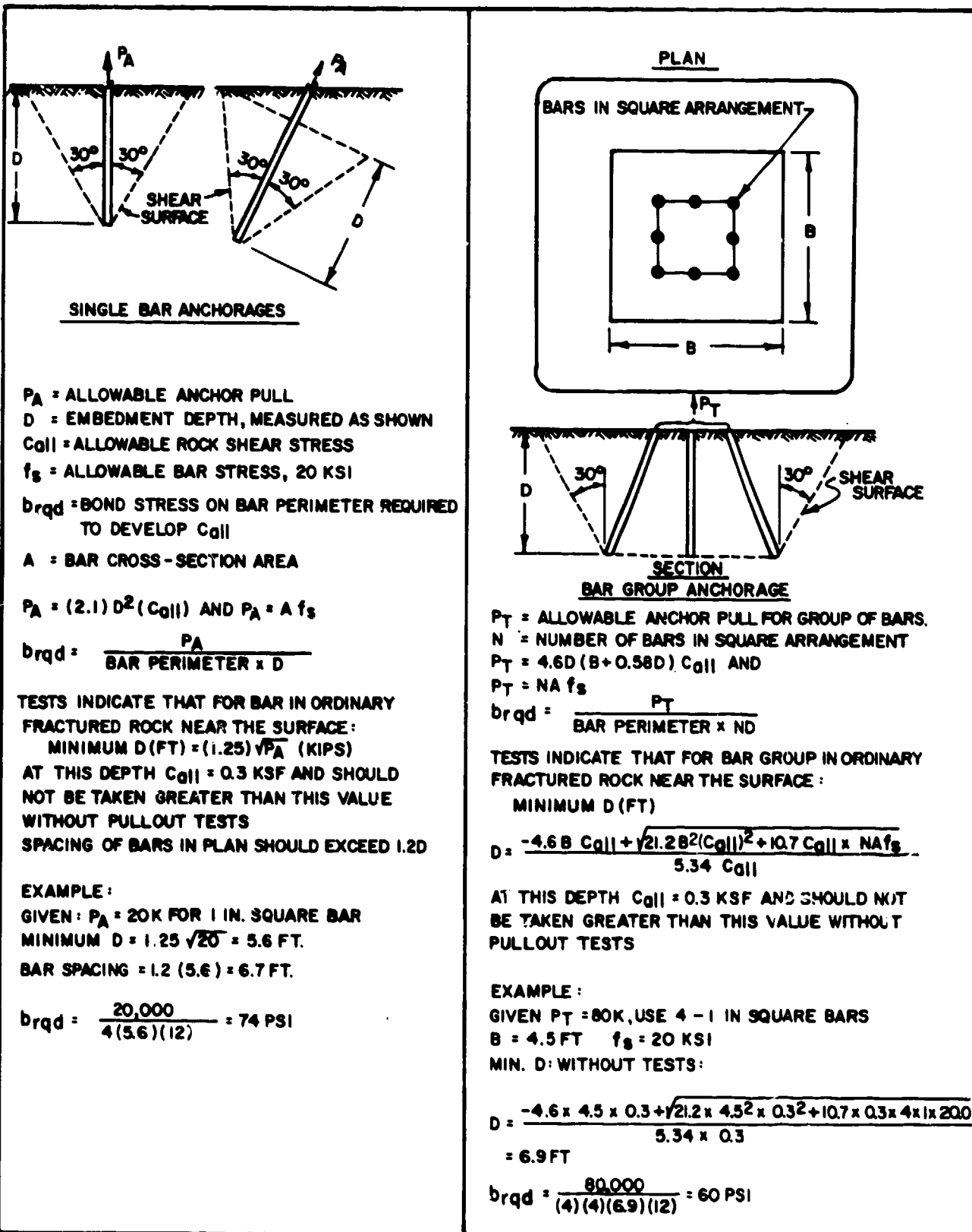
FIGURE 16 Capacity of Anchor Rods in Fractured Rock
