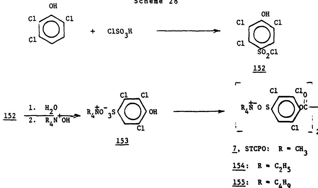
Scheme 28
