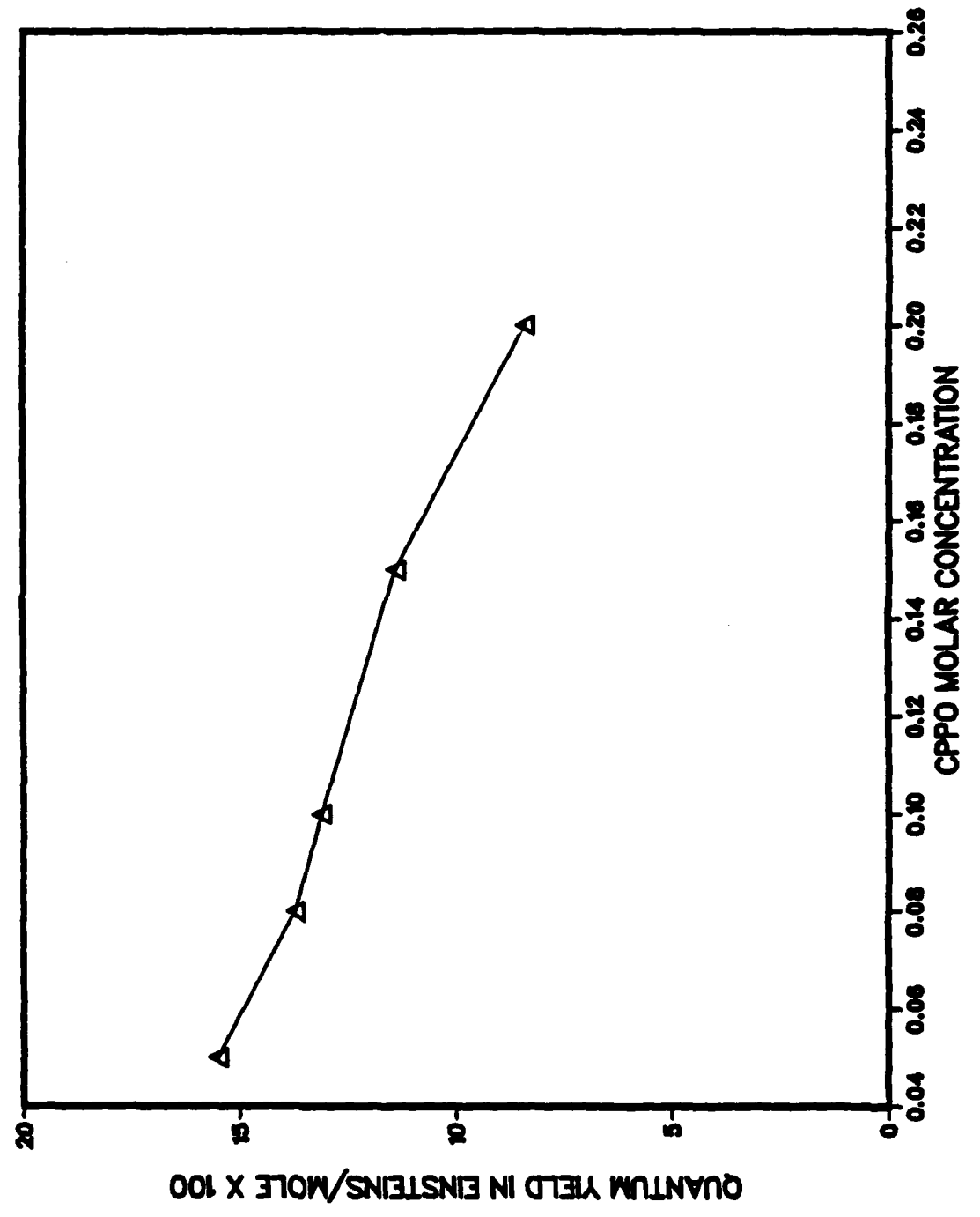
FIG.16: EFFECT OF CPPO CONCENTRATION ON BOBPEA EFFICIENCY
