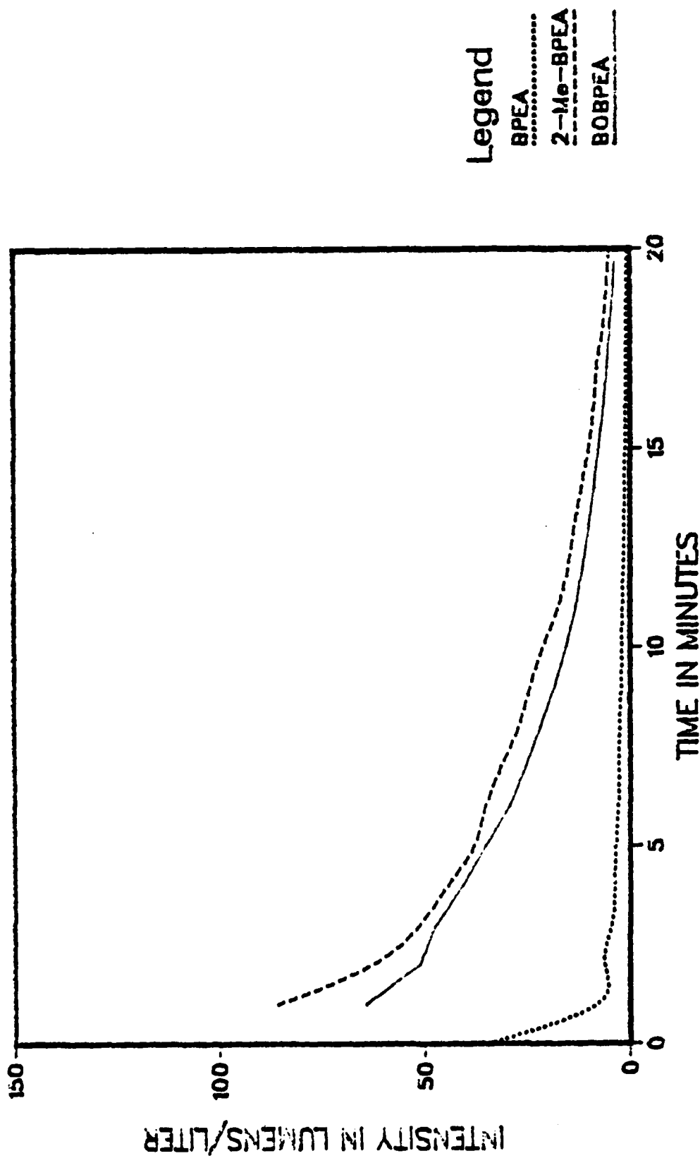
FIG. 11: CHEMILUMINESCENCE OF ALKYL BPEA DERIVATIVES IN AQUEOUS EMULSION
