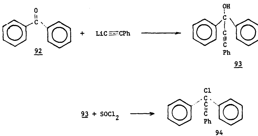
Scheme 15
