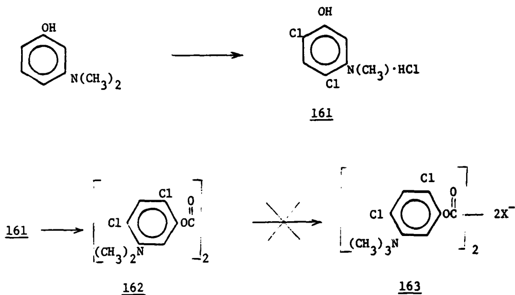
Scheme 29
