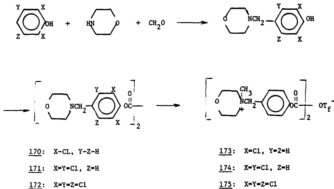
Scheme 31
