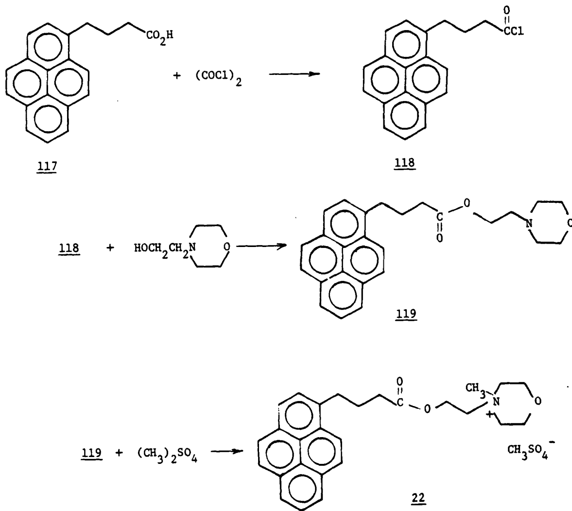
Scheme 23
