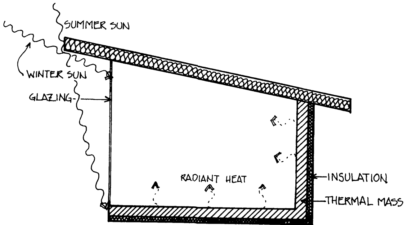
Figure 1. Direct gain.
