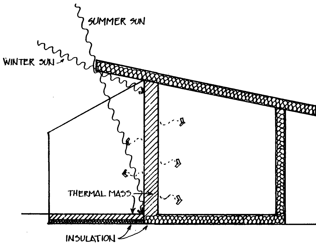
Figure 4. Attached sunspace.
