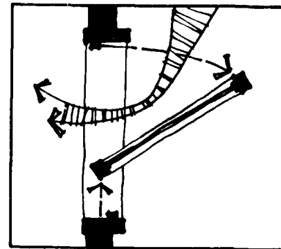
Use both high and low windows or vents in the house to improve air movement at night. Windows must be operable, preferably they should be of a vertical casement type to minimize unventilated air pockets
