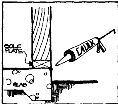
Seal the building against infiltration by caulking under the sole plate and around other openings in the building shell. Weatherstripping on doors and windows is also essential.
