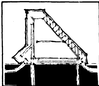
Use thermal chimneys when there are no breezes to induce air movement through the stack effect
