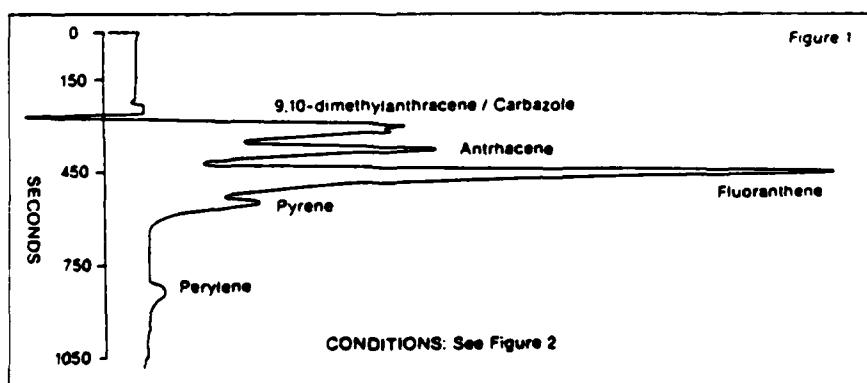
FIGURE 50. Separation of aromatic hydrocarbons with UV detection.
