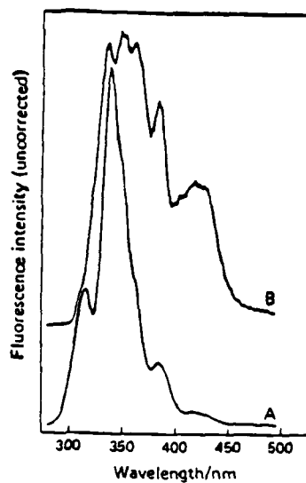
FIGURE 29. Synchronously excited spectra (30 nm) of a naphthenic oil (1 mg ml -1 ). (A) cyclohexane. (B) chloroform. B is at ten times greater sensitivity than A. (From Lloyd, J. B. F., Analyst , 100, 82, 1975. With permission.)
