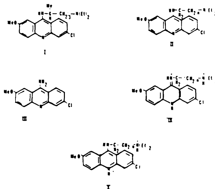
FIGURE 9 Structure of atabrine and related species. I atabrine (base form). II, homologous series n = 1 to n = 7 (base form). III, parent compound (base form). IV, homologous series (acid form). V, proposed excited state species (acid form). (Reprinted with permission from Love, L. J. C., Upton, L. M., and Ritter, A. W., Anal. Chem. , 50, 2059, 1978. Copyright 1978 American Chemical Society.)
