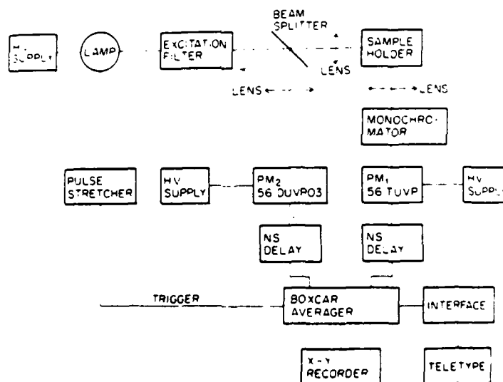
FIGURE 8 Block diagram of a nanosecond fluorimeter. The photomultipliers are manufactured by Amperex. The triggering signal was stretched by a Tektronix rise-time limiter. The input to each channel was delayed by about 80 nsec. (From Badca, M. G. and Georghiou, S., Rev. Sci. Instrum. , 47, 314, 1976. With permission.)
