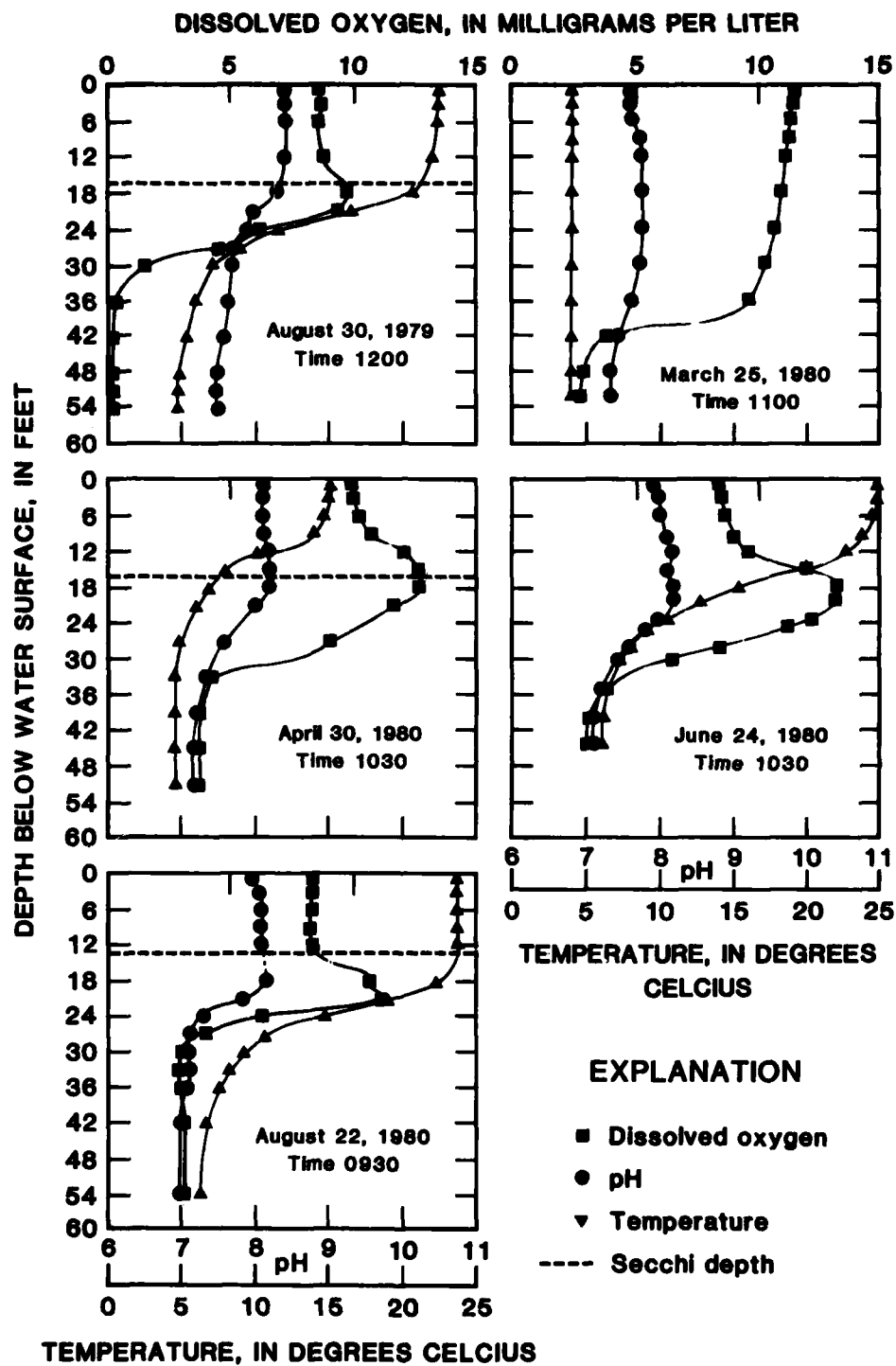
Figure 8.--Vertical profiles of Courthouse Lake
