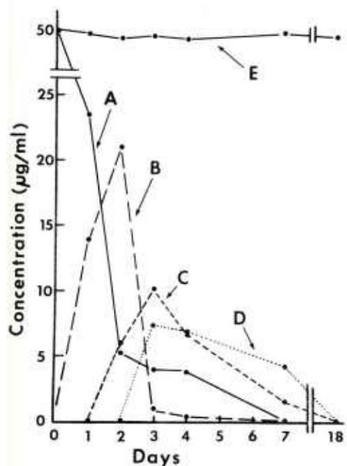
Figure 3. Disappearance of RDX and production of intermediates during anaerobic incubation. A = RDX; B = 1-nitroso-3,5-dinitrohexahydro-1,3,5-triazine; C = 1,3-dinitroso-5-nitro-hexahydro-1,3,5-triazine; D = 1,3,5-trinitroso-hexahydro-1,3,5-triazine; E = RDX incubated under aerobic conditions.
