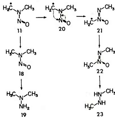
Figure 8. Proposed RDX biodegradation pathway. 18, dimethylnitrosamine; 19, 1,1-dimethylhydrazine; 20, hypothetical intermediate; 21, dimethyldiazene-1-oxide radical; 22, dimethyldiazene-1-oxide; 23, 1,2-dimethylhydrazine.
