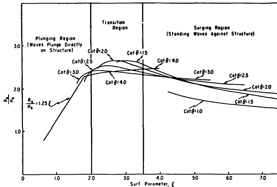
Figure 7. R_s/H_s versus the surf parameter for d_s/H_s > 3 .
