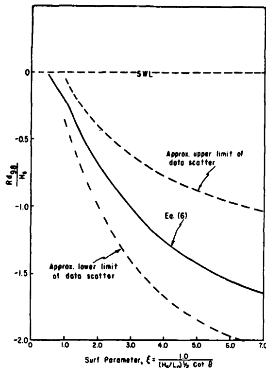
Figure 8. Rd_{98}/H_s versus the surf parameter.
