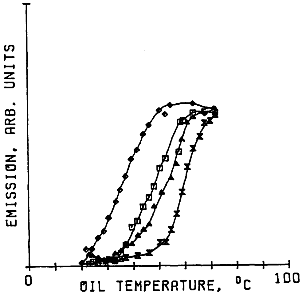
FIGURE 2. EMISSION INTENSITY AS A FUNCTION OF TEMPERATURE FOR VARIOUS GRADES OF PENNZOIL MOTOR OIL. 20W, 30W, 40W, 50W.
