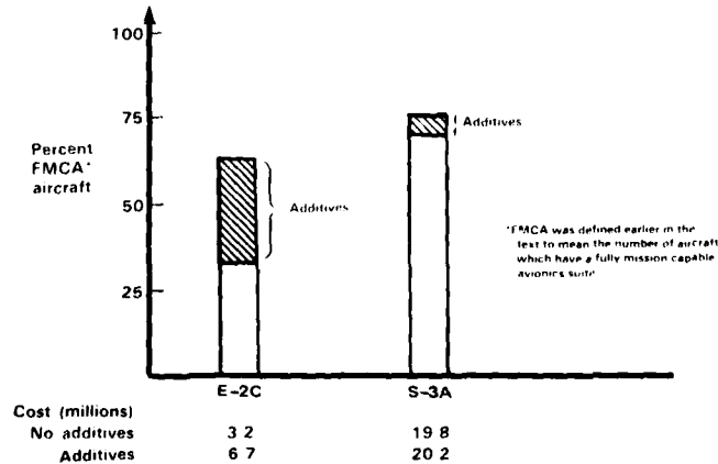
Fig. IV-1-Costs and effects of AVCAL additives on aircraft availability—day 90 of scenario
