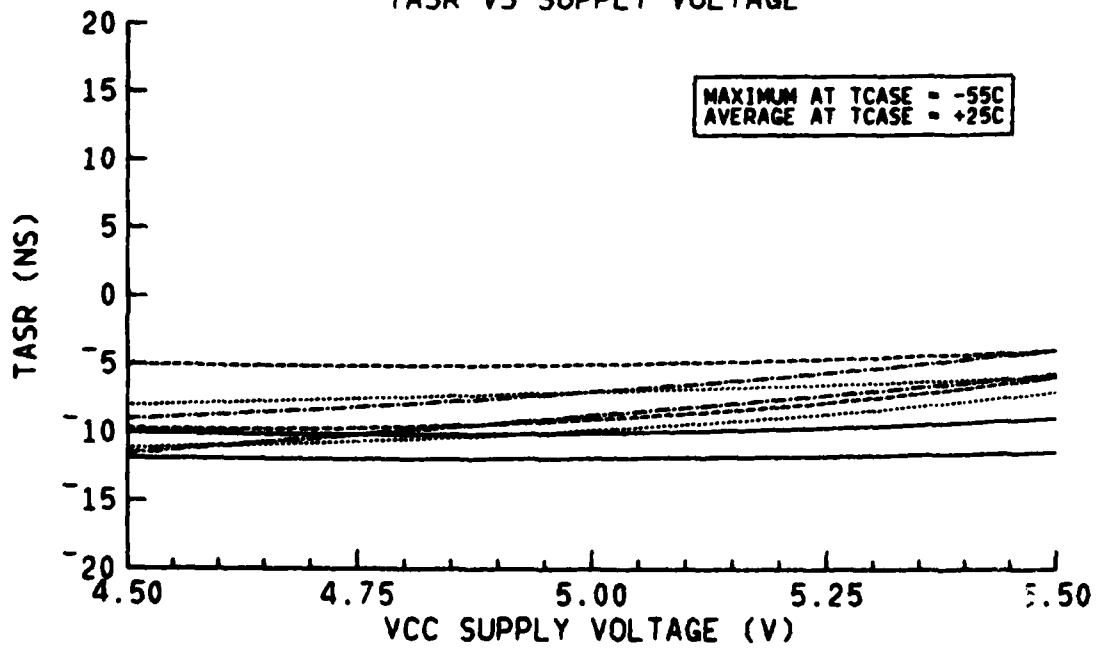
TASR VS SUPPLY VOLTAGE
