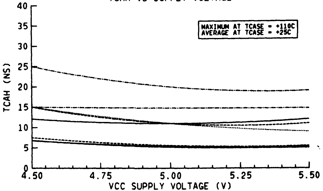
TCAH VS SUPPLY VOLTAGE
