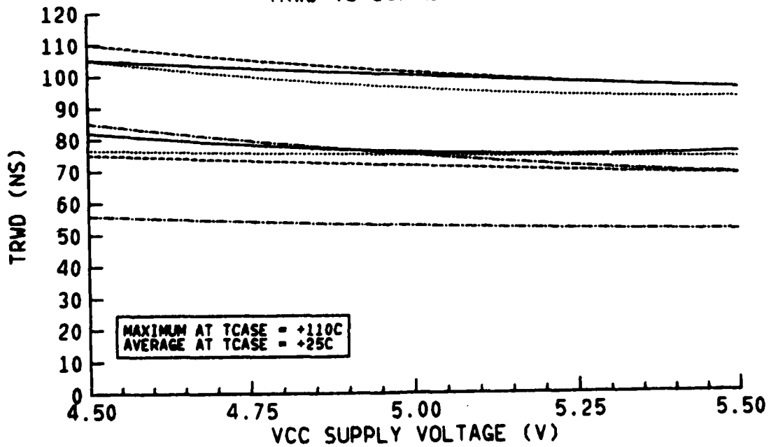
TRWD VS SUPPLY VOLTAGE
