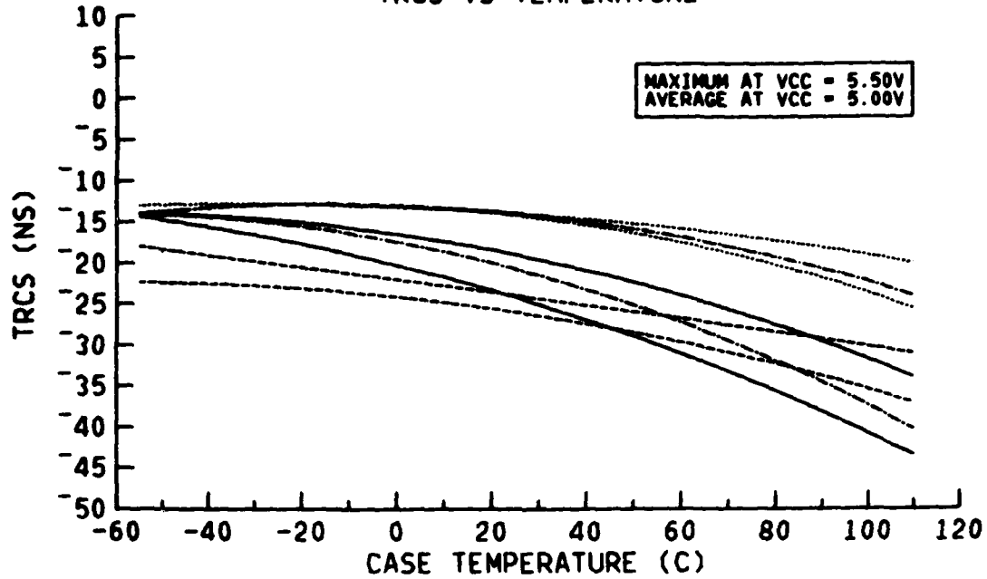
TRCS VS TEMPERATURE
