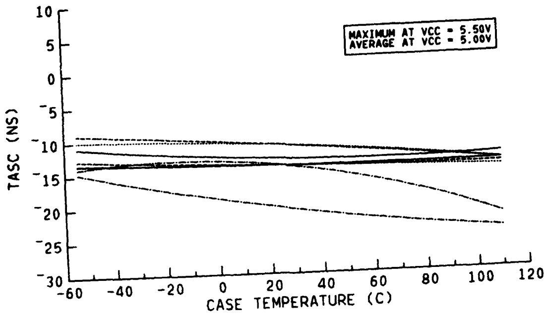
TASC VS TEMPERATURE
