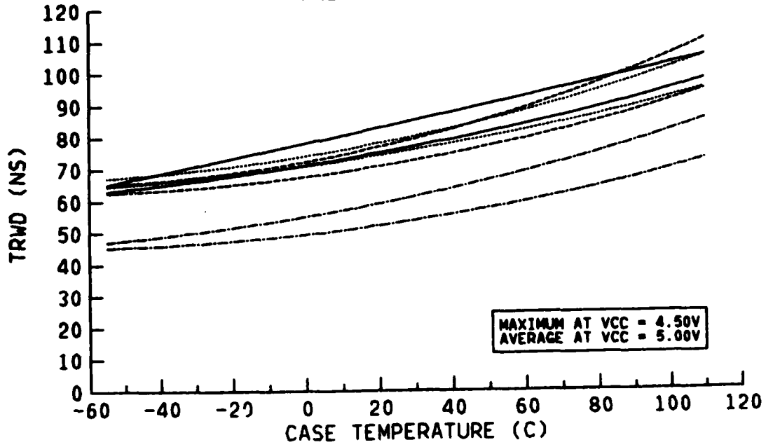
TRWD VS TEMPERATURE
