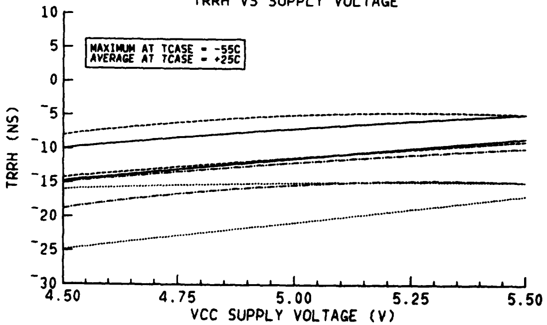
TRRH VS SUPPLY VOLTAGE
