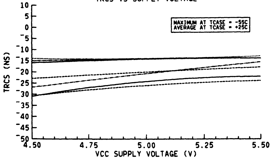
TRCS VS SUPPLY VOLTAGE
