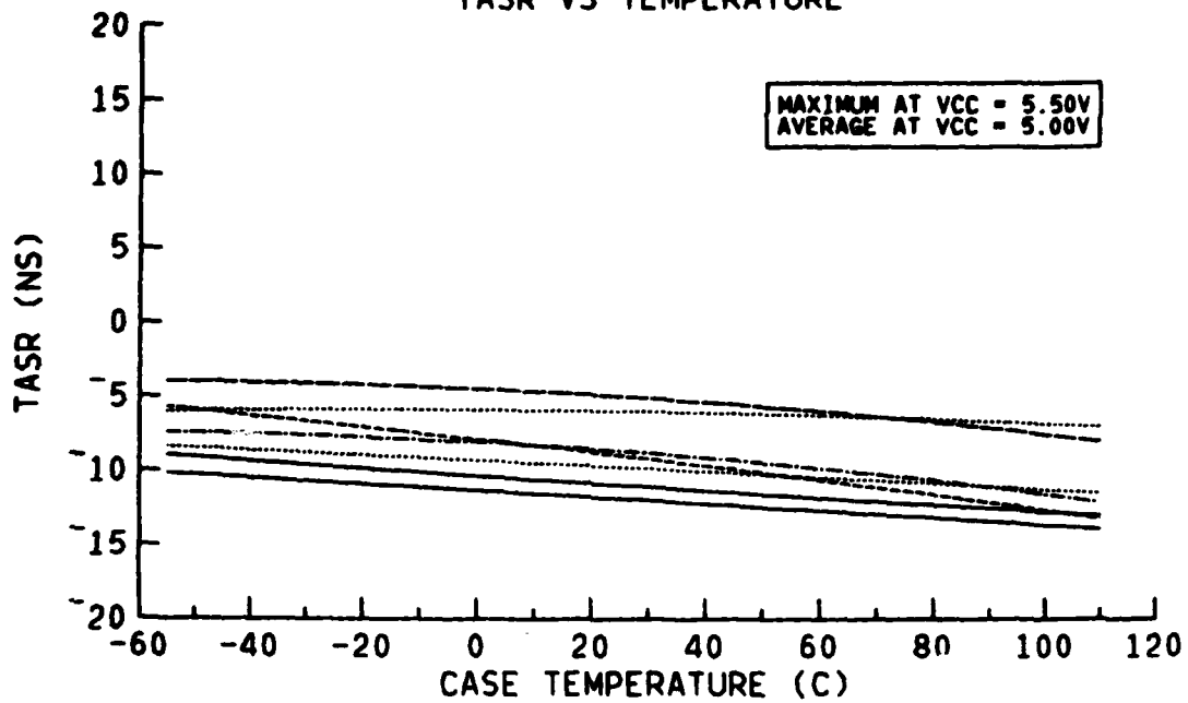
TASR VS TEMPERATURE
