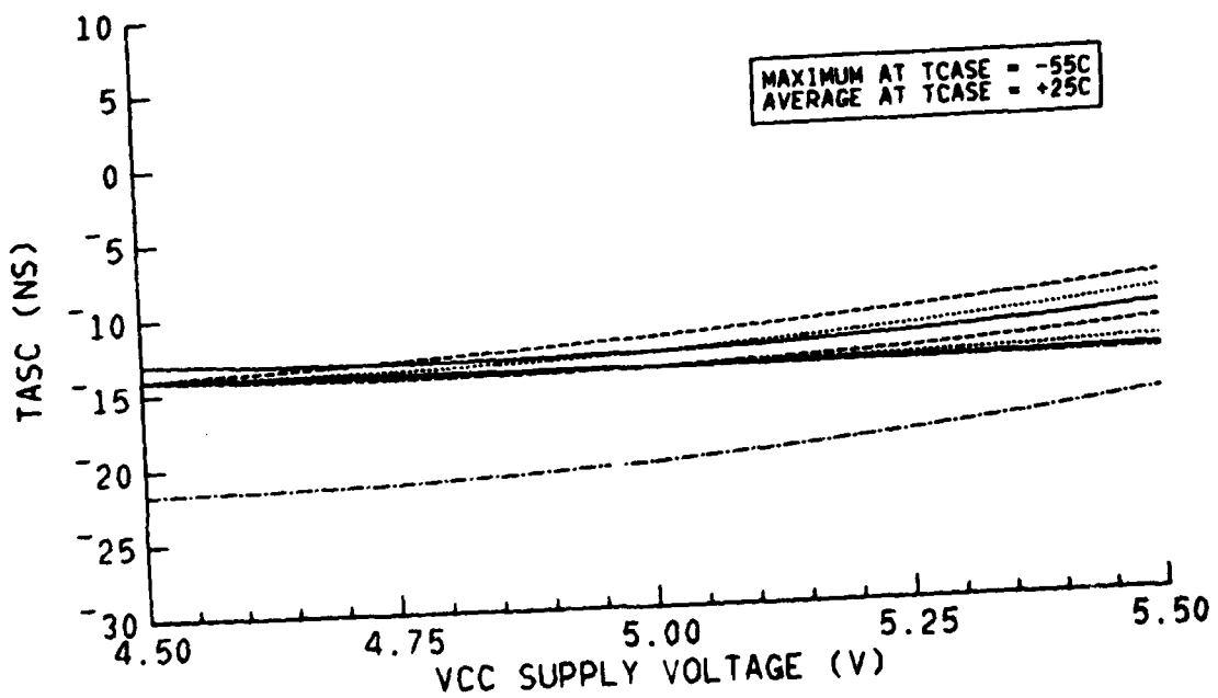
TASC VS SUPPLY VOLTAGE
