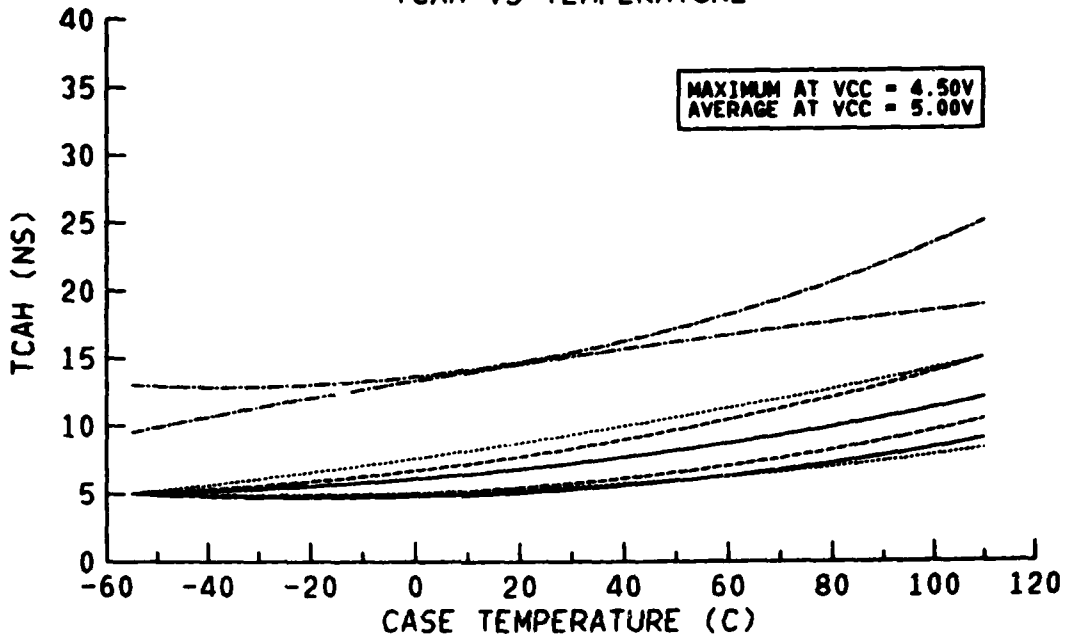
TCAH VS TEMPERATURE
