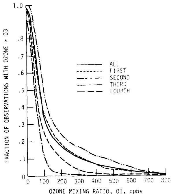
Figure 6. Cumulative ambient ozone frequency distribution for B747-100 for one year.
