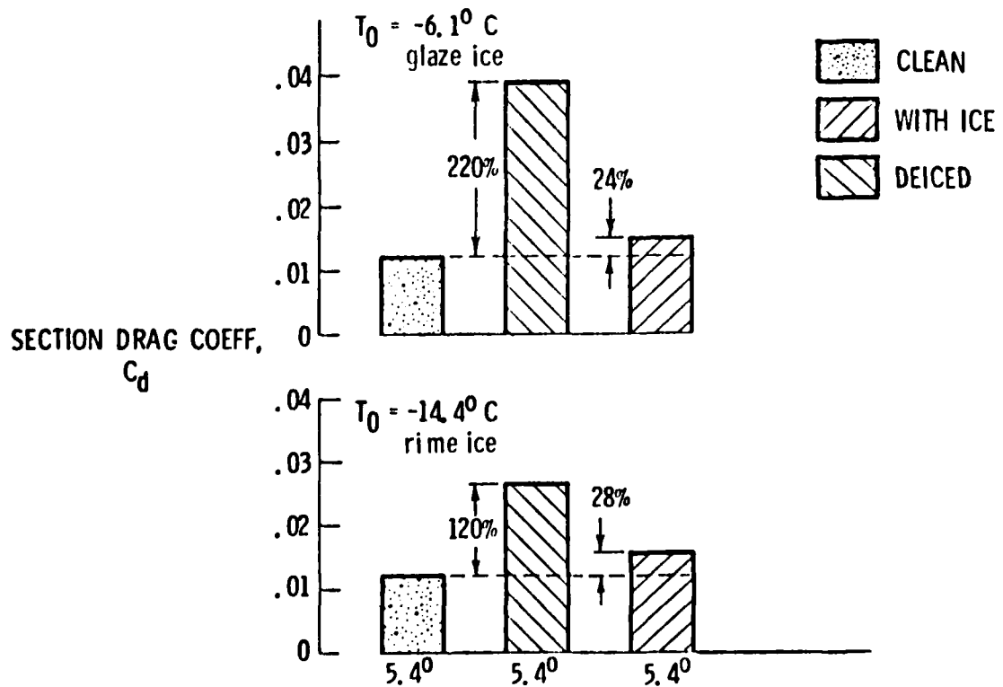
Figure 10. Section drag of helicopter rotor model with pneumatic boot.
