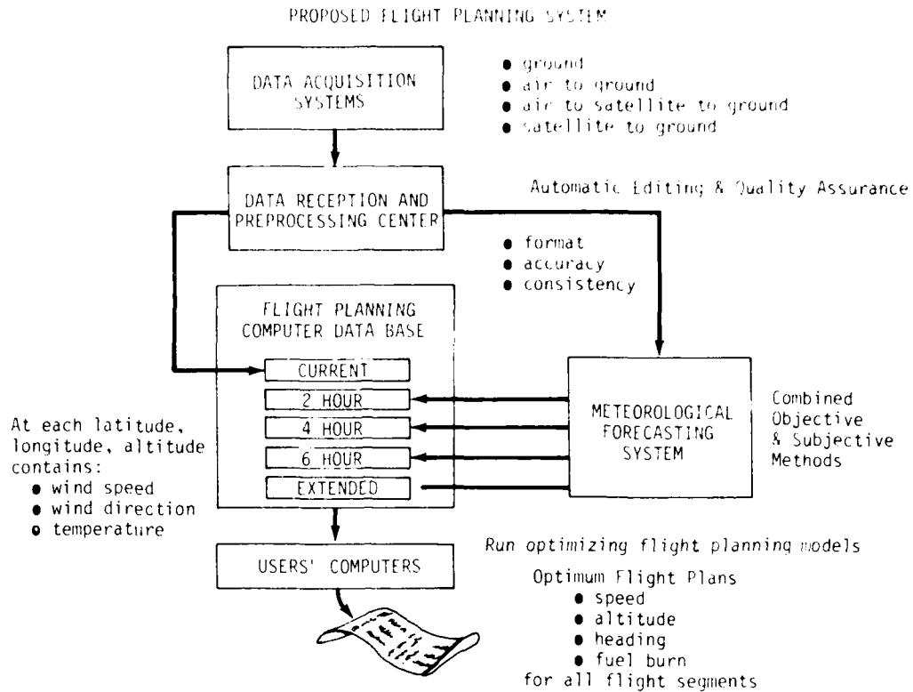
Figure 2. A conceptual plan for development of a wind and temperature data system that is specifically tailored to the needs of flight planning. Such data are essential for maximum fuel savings that can be determined with new fuel-burn optimizing models.
