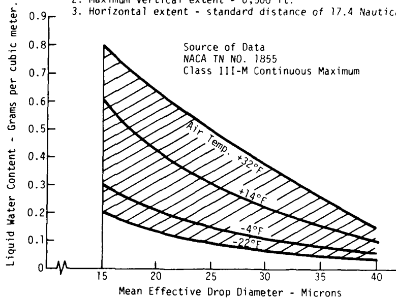
Figure 1. Continuous maximum (Stratiform Clouds) atmospheric icing conditions. Liquid water content vs. mean effective drop diameter.
