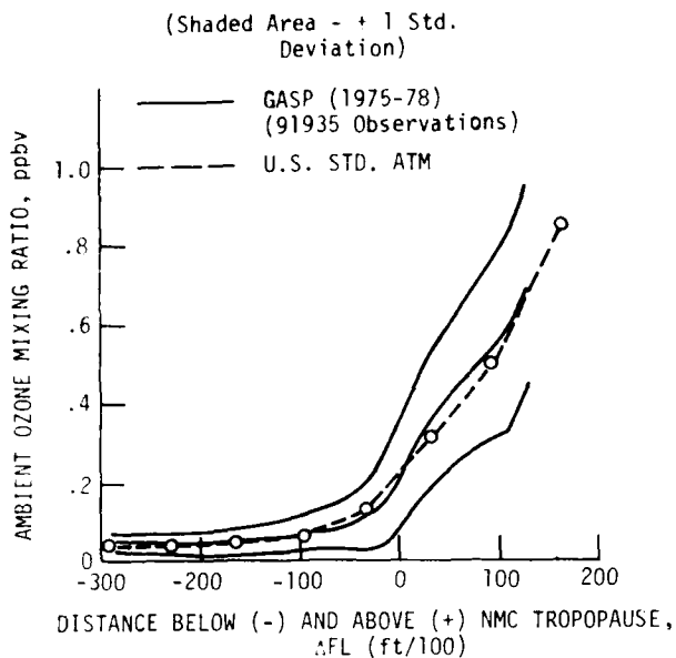
Figure 3. Ambient ozone mixing ratios with respect to the tropopause.
