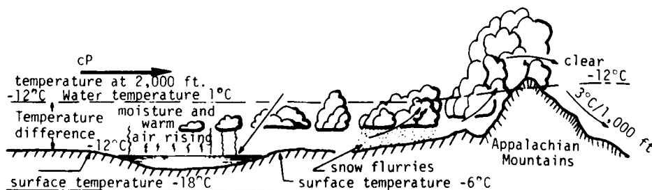
Figure 6. cP air moving over the Great Lakes.
