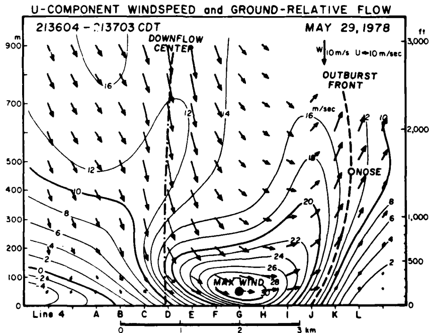
Figure 1. A vertical cross section through the 29 May 1978 microburst showing isotachs of horizontal windspeeds. The height of the maximum wind is estimated to be 50 m or lower. Arrows are ground-relative velocities in the plane which is stretched vertically.
