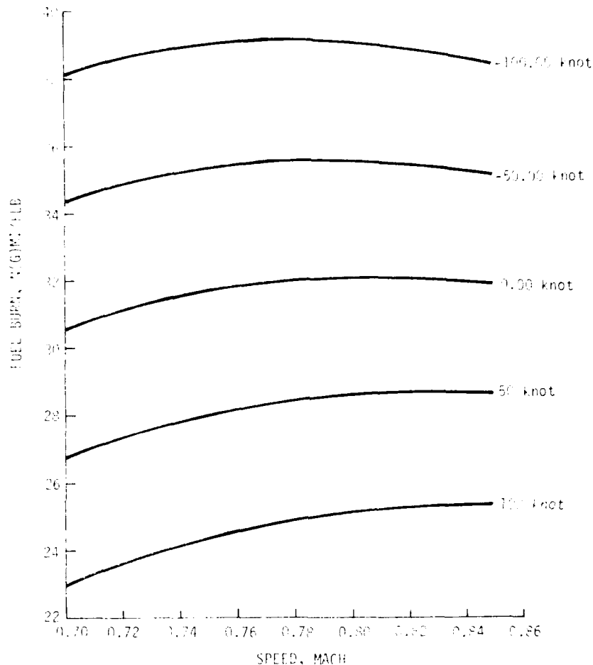
Figure 1. Example of the impact of wind on fuel efficiency in terms of nautical ground miles per kilopound of fuel burned for a DC-10-10 at 37,000 feet. Negative speeds signify tailwinds. Route and altitude selection to achieve the most distance for a given amount of fuel requires wind forecasts for the projected time of arrival for each segment of a trip.
