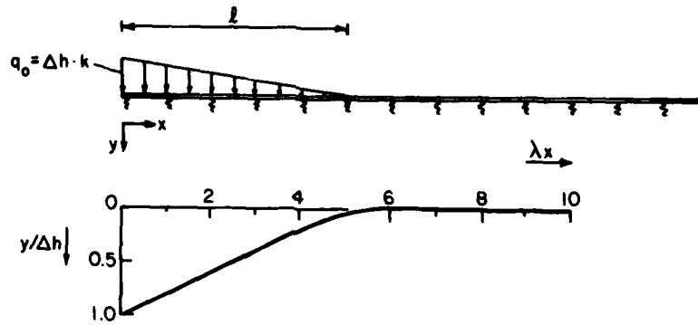
Figure 6. Deflection of the edge of the ice cover for the wave height \Delta h < 0.9d , \lambda l = 5 and s = 0 according to eq 32 and 33.
