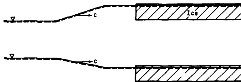
Figure 2. Negative and positive surge waves approaching the edge of an ice cover.
