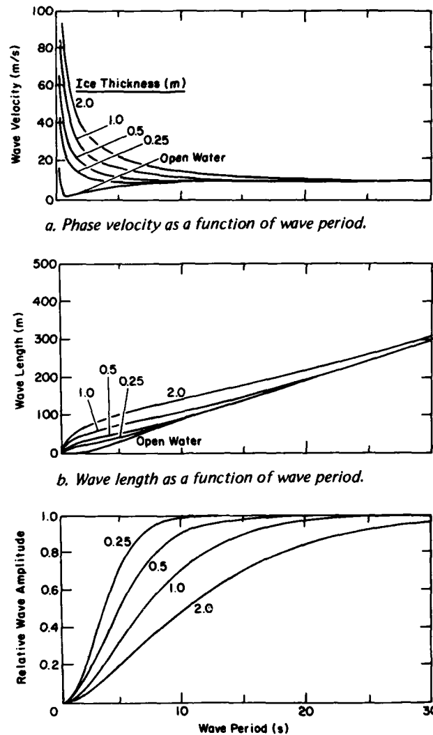
c. Damping of the amplitude as a function of wave period.
