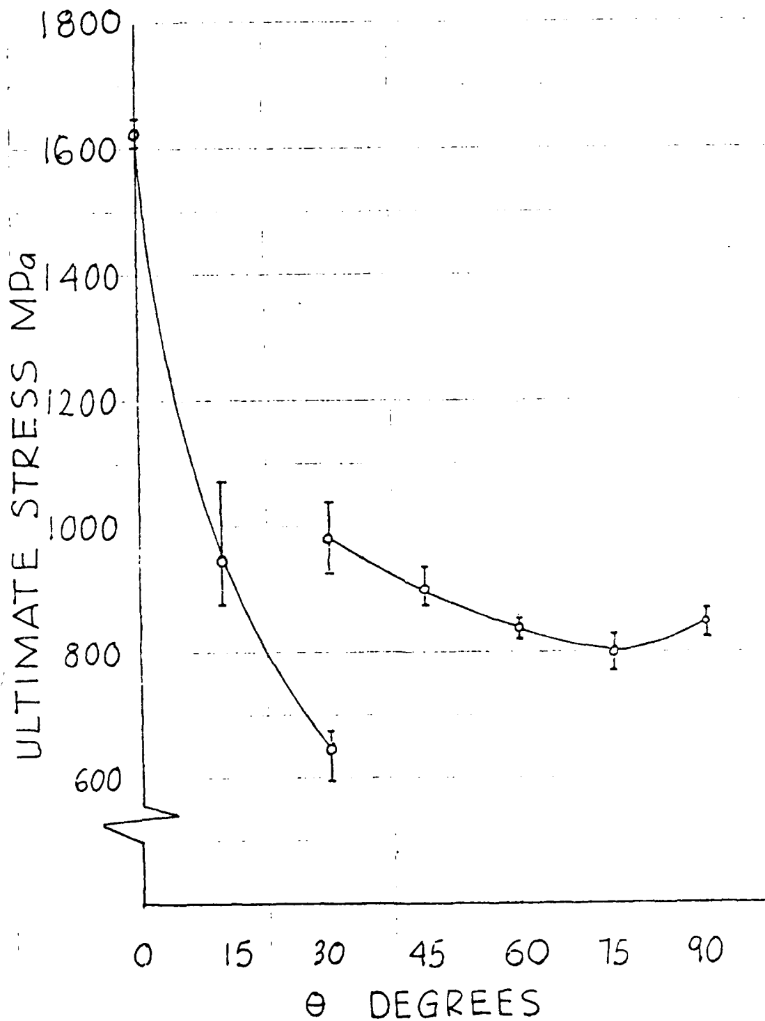
FIGURE 2 FRACTURE OF [0_2/\pm\theta]_s LAMINATE WITH A HOLE
