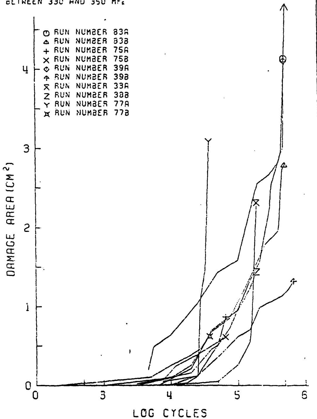
FIGURE 13 DAMAGE AREA VERSUS CYCLES ( \pm 45/0 ), FATIGUE FAILURES
