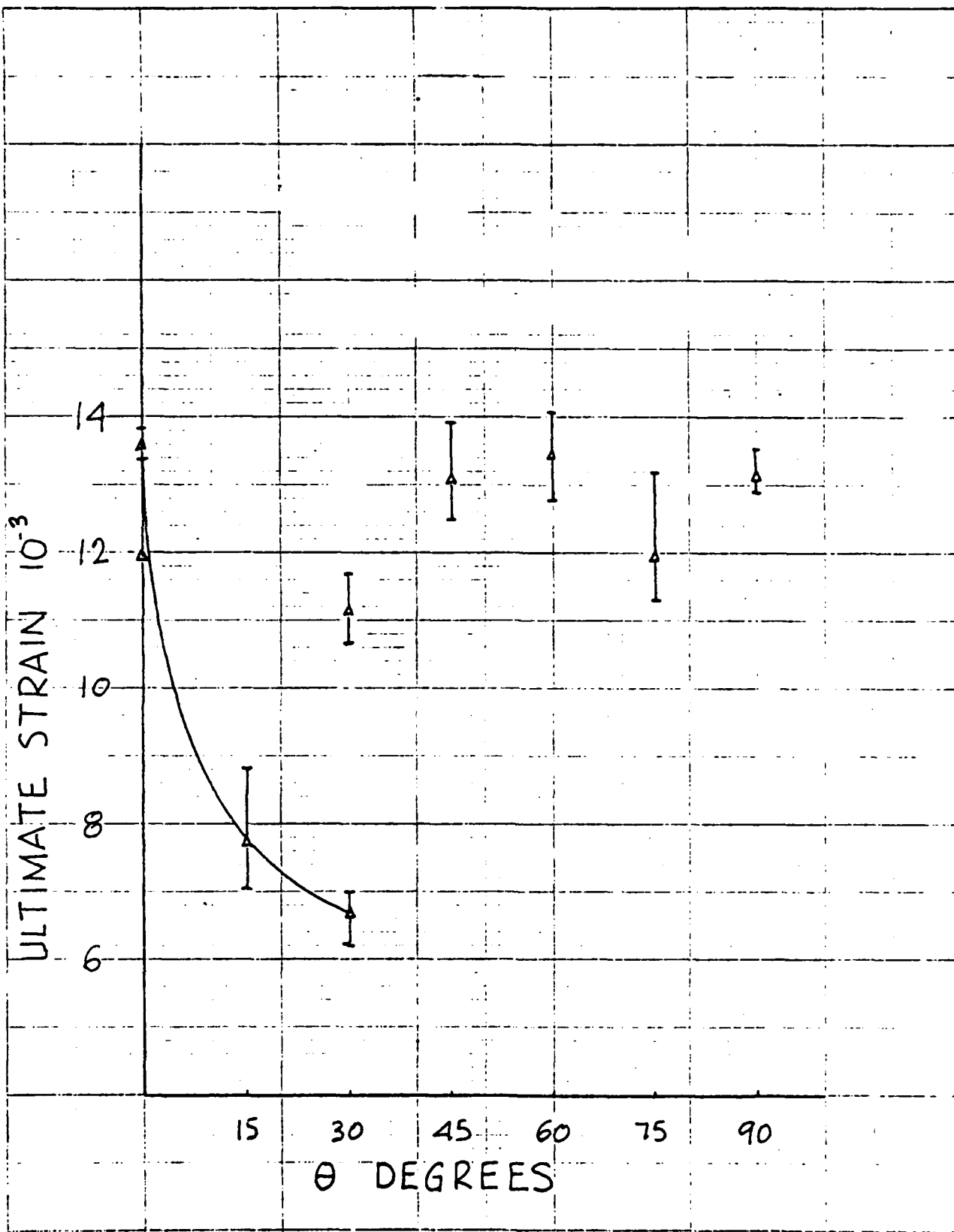
FIGURE 3 ULTIMATE STRAIN OF [0_2/\pm\theta]_s LAMINATES WITH A HOLE
