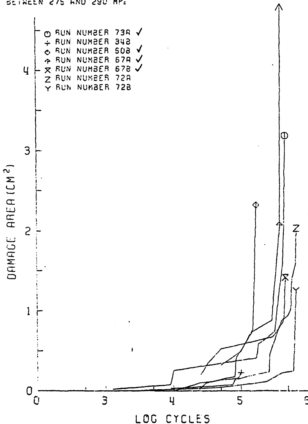
FIGURE 19 DAMAGE AREA VERSUS CYCLES (0/±30)ₛ FATIGUE TEST DATA
