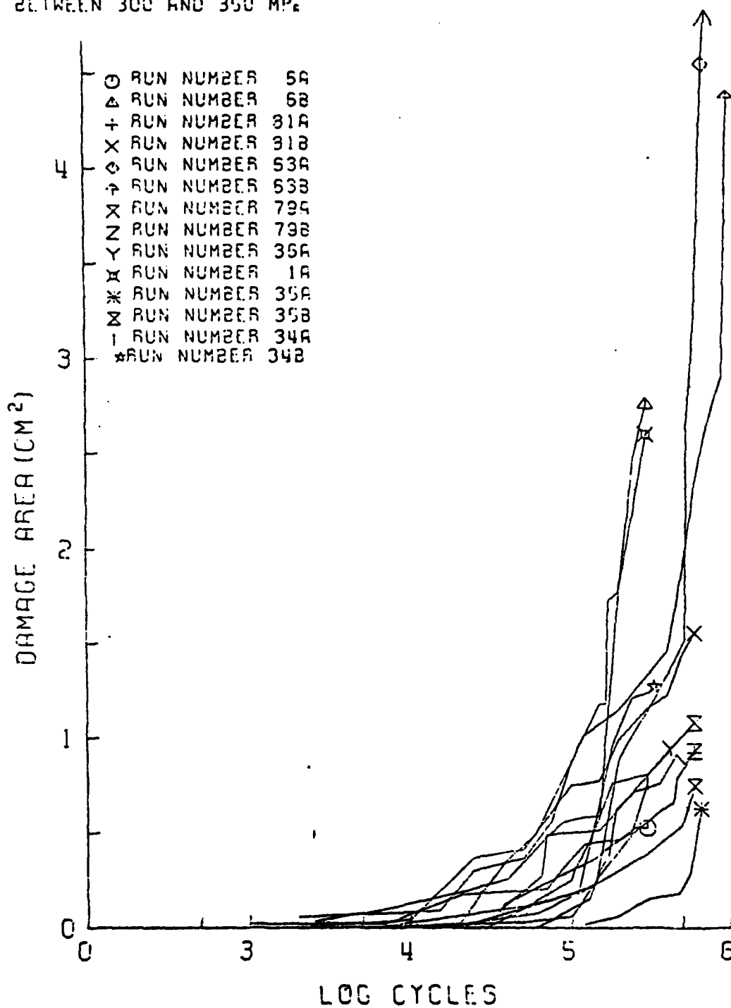
FIGURE 15 DAMAGE AREA VERSUS CYCLES ( \pm 45/0 ) s FATIGUE TEST - UNFAILED SPECIMENS
