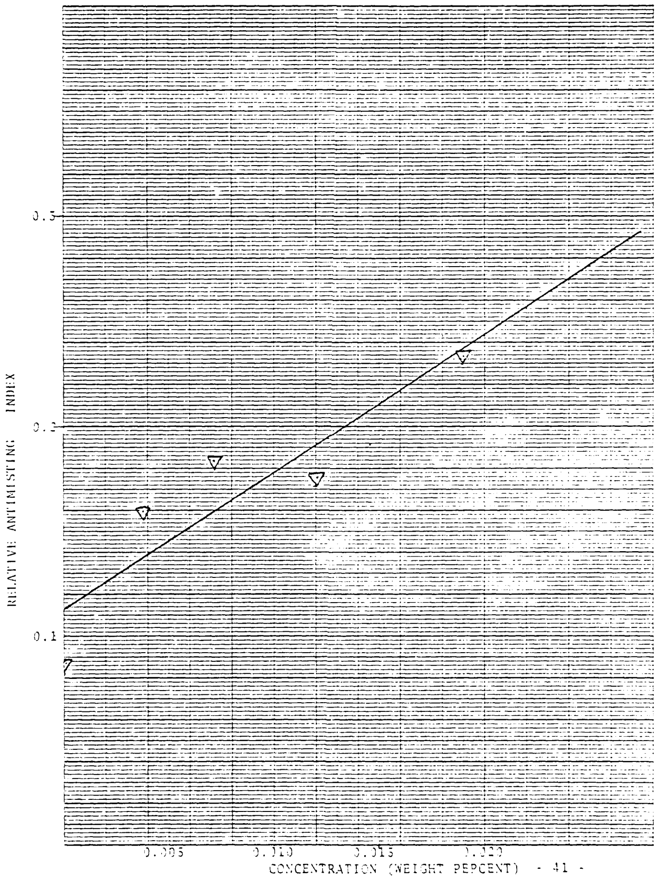
FIGURE 17: FIRESTONE RDP 10955 ANTIMISTING AS POLYMER CONCENTRATION
