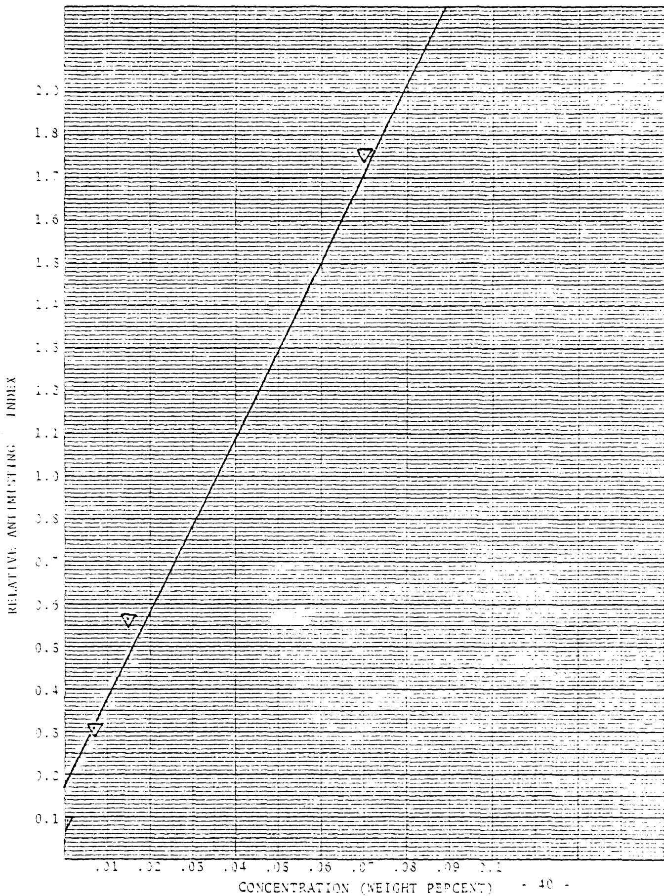
FIGURE 16: B-250 ANTIMISTING VS POLYMER CONCENTRATION
