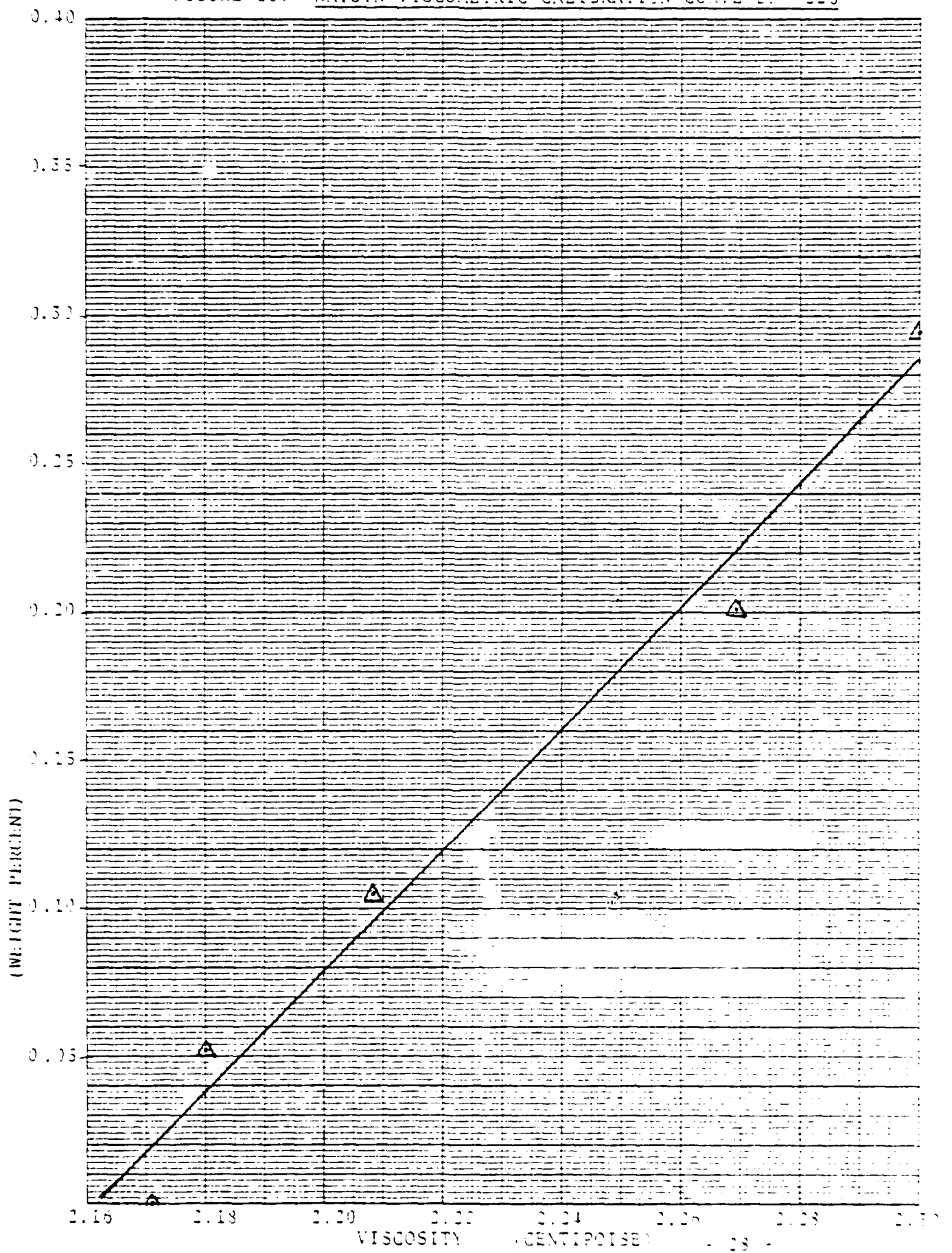
FIGURE 10: NATSYN VISCOMETRIC CALIBRATION CURVE (DF 7025)
