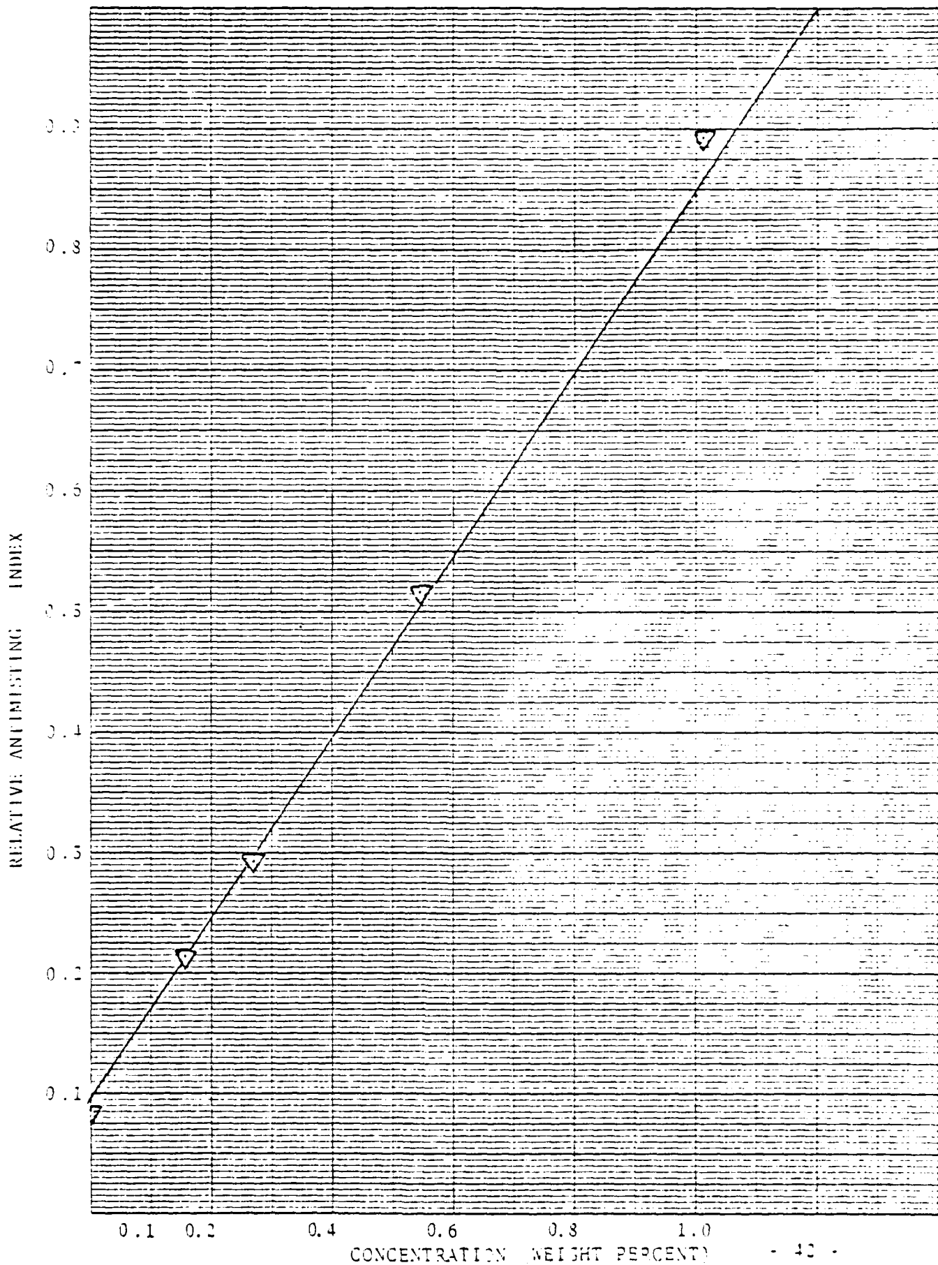
FIGURE 18: NATSYN ANTIMISTING VS POLYMER CONCENTRATION
