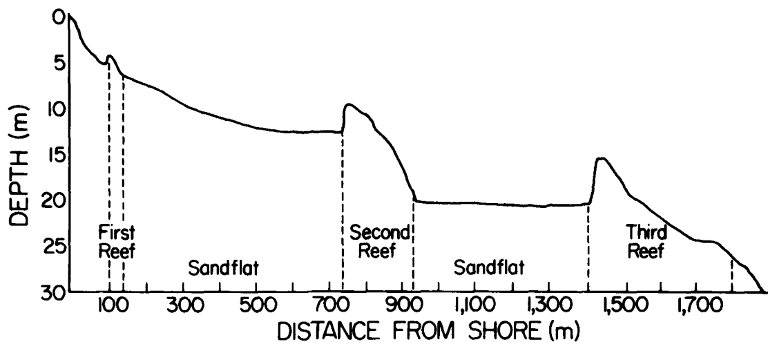
Figure 1. Profile of shelf morphology off Hillsboro Beach, Florida.
