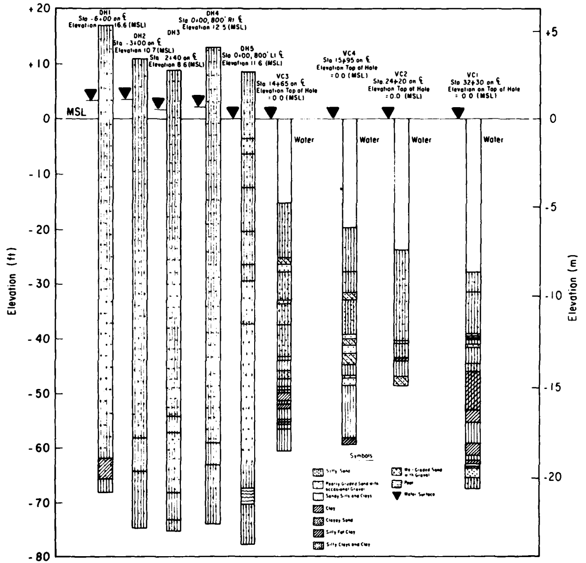
Figure 53. Summary of drill hole and vibracore logs.
