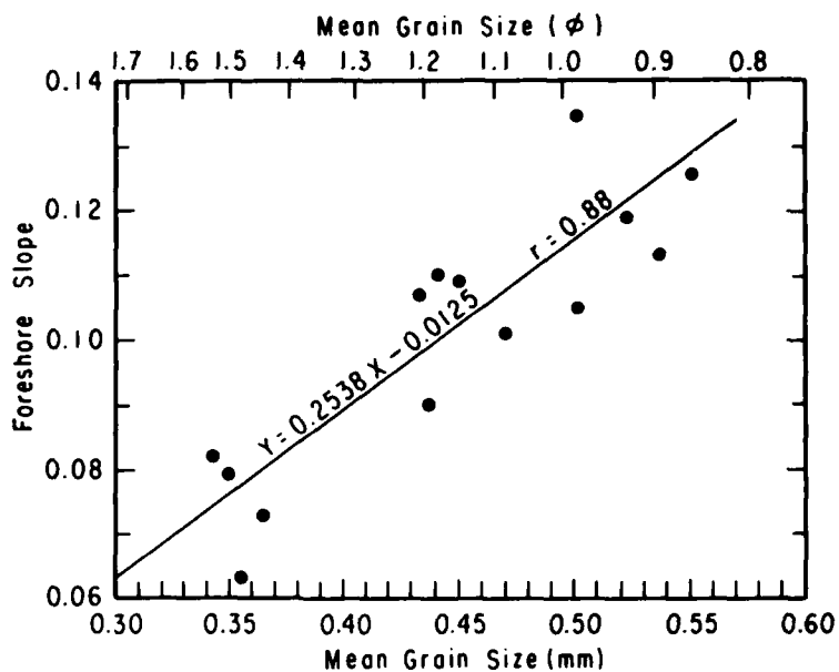
Figure 49. Average foreshore slope versus average mean grain size.
