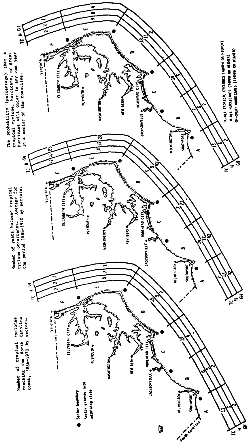
Figure 22. Hurricane statistics for North Carolina (adapted from Baker, 1978).
