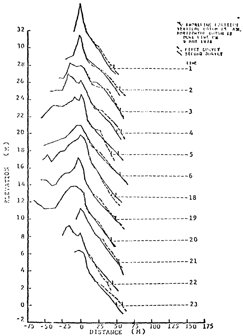
Figure 32. Typical storm changes, 4 November to 4 December 1974 ( \bar{\Delta v} = 5.8 \text{ m}^3/\text{m} ).
