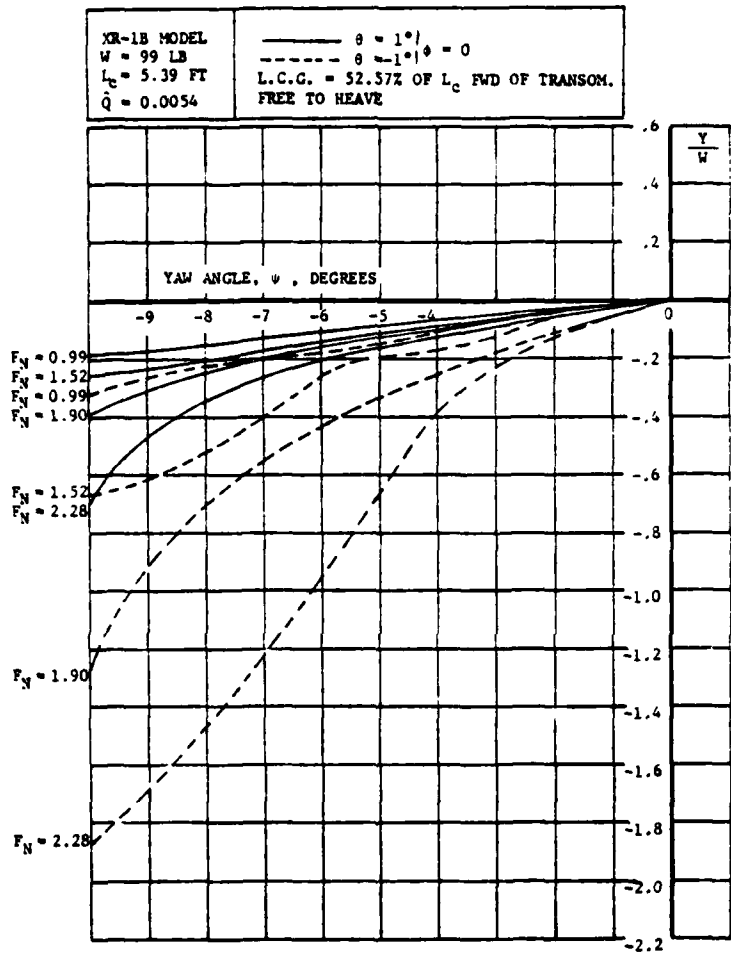
FIGURE A-2.1(g). SIDE FORCE V. YAW AND PITCH ANGLE AND FROUDE NO.
