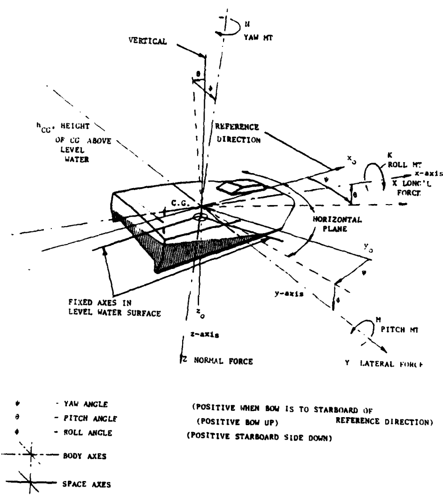
FIGURE 3-1. DEFINITION OF AXIS SYSTEM.
