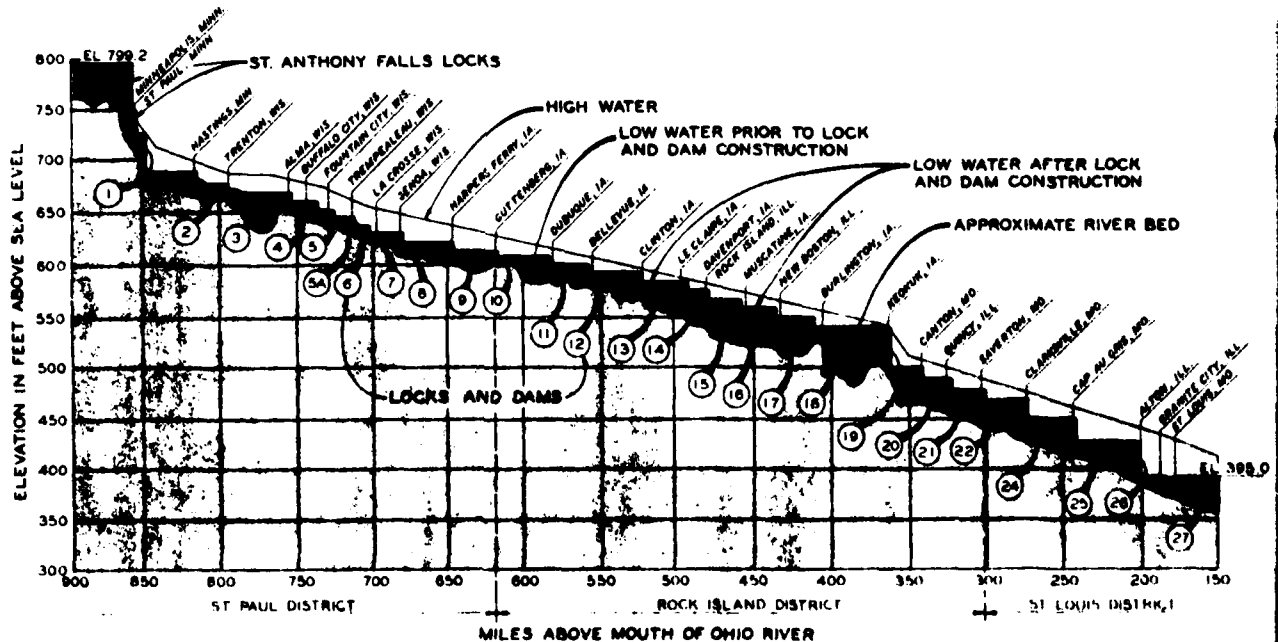
Fig. 2 . The 9-foot channel project has changed the Upper Mississippi River into a series of "steps" which river tows "climb" or "descend" as they travel upstream or downstream.
