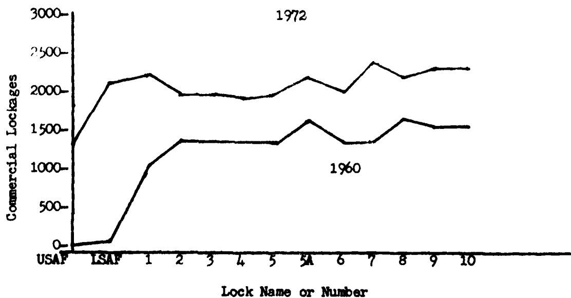
Figure 29. Commercial Lockages in Upper Mississippi River in 1960 and 1972. Source: St. Paul District of the U.S. Army Corps of Engineers, Annual Lockage Data, 1960 and 1972.
