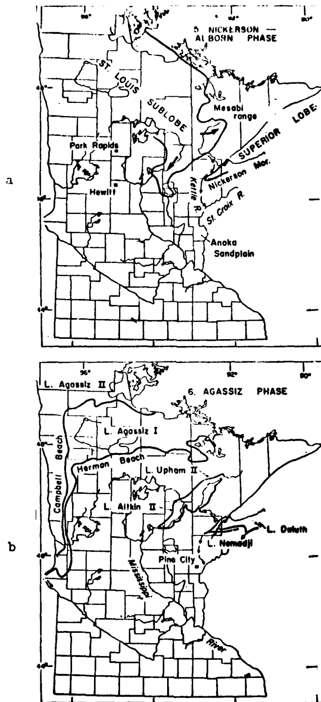
Figure 12. Nickerson-Alborn and Agassiz phases of Wisconsin glacialation in Minnesota (Wright and Ruhe, 1965).
