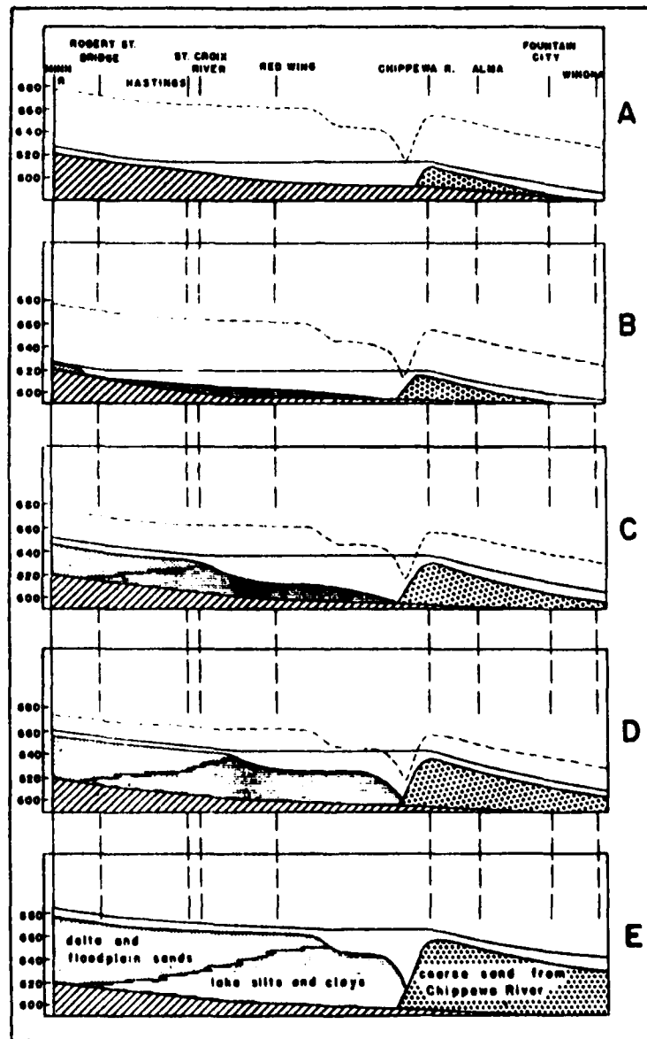
Figure/3.--Diagrammatic history of Lake Pepin (Zumberge, 1952). See text for complete explanation.
