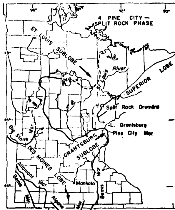
Figure 10. Hewitt, St. Croix, Automba-Vermilion, and Pine City-Split-Rock phases of Wisconsin glaciation in Minnesota (Wright & Ruhe, 1965).
