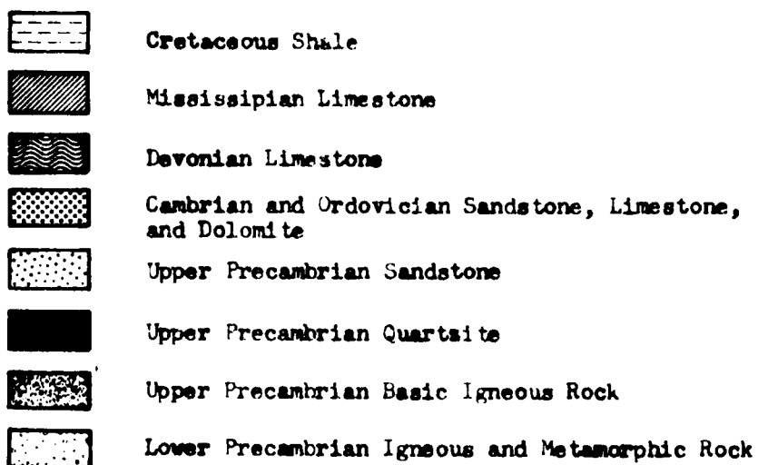
Figure // . Geologic map of the Upper Midwest.
